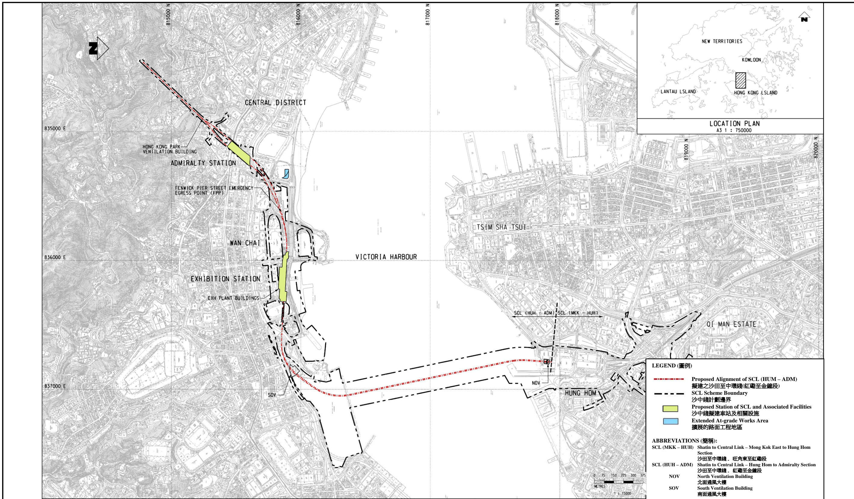
Figure 1: Alignment of Shatin to Central Link - Hung Hom to Admiralty Section 圖 沙田至中環綫 - 紅磡至金鐘段之全段走綫示意圖
