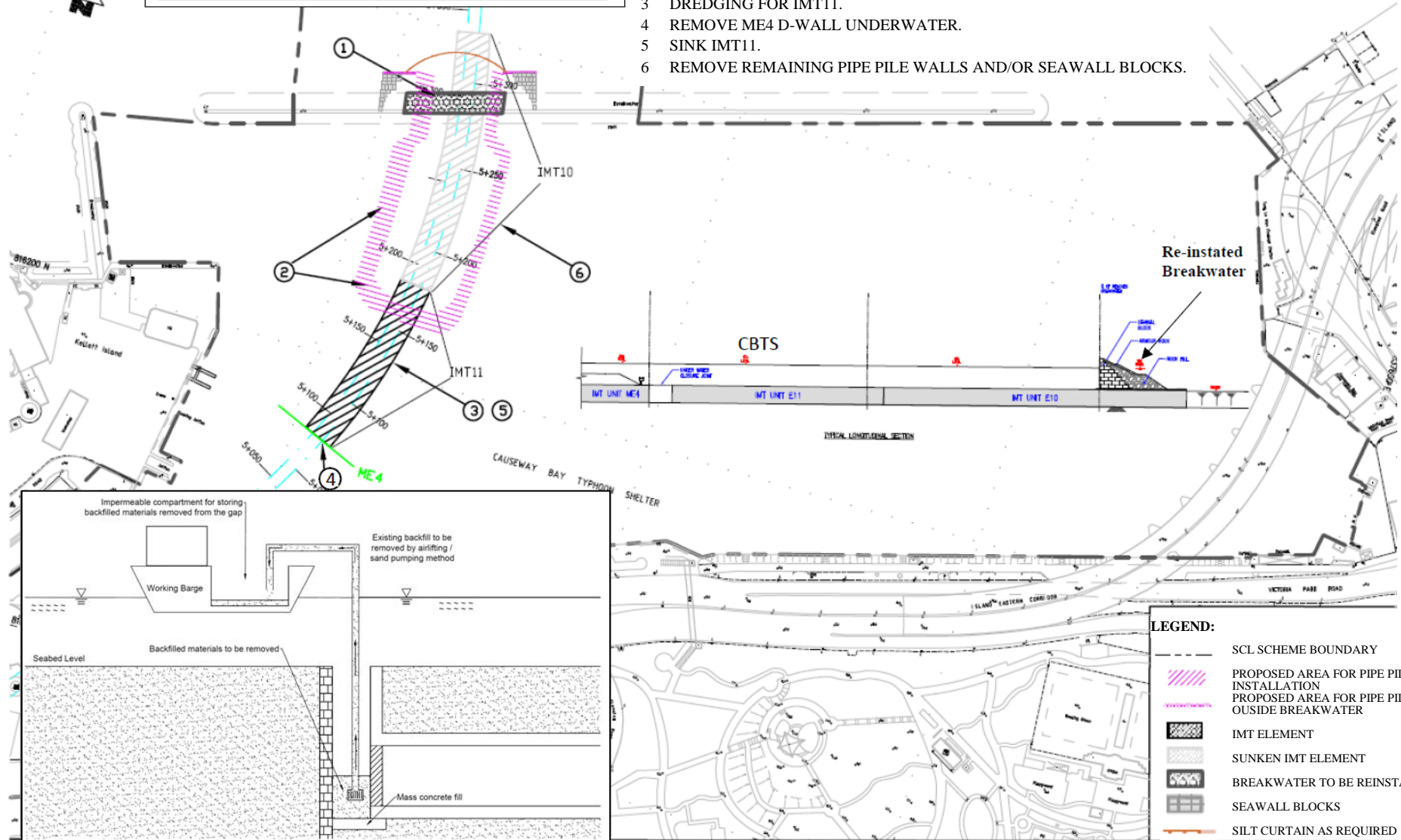
Figure 10: Final Stage of IMT Construction at CBTS
