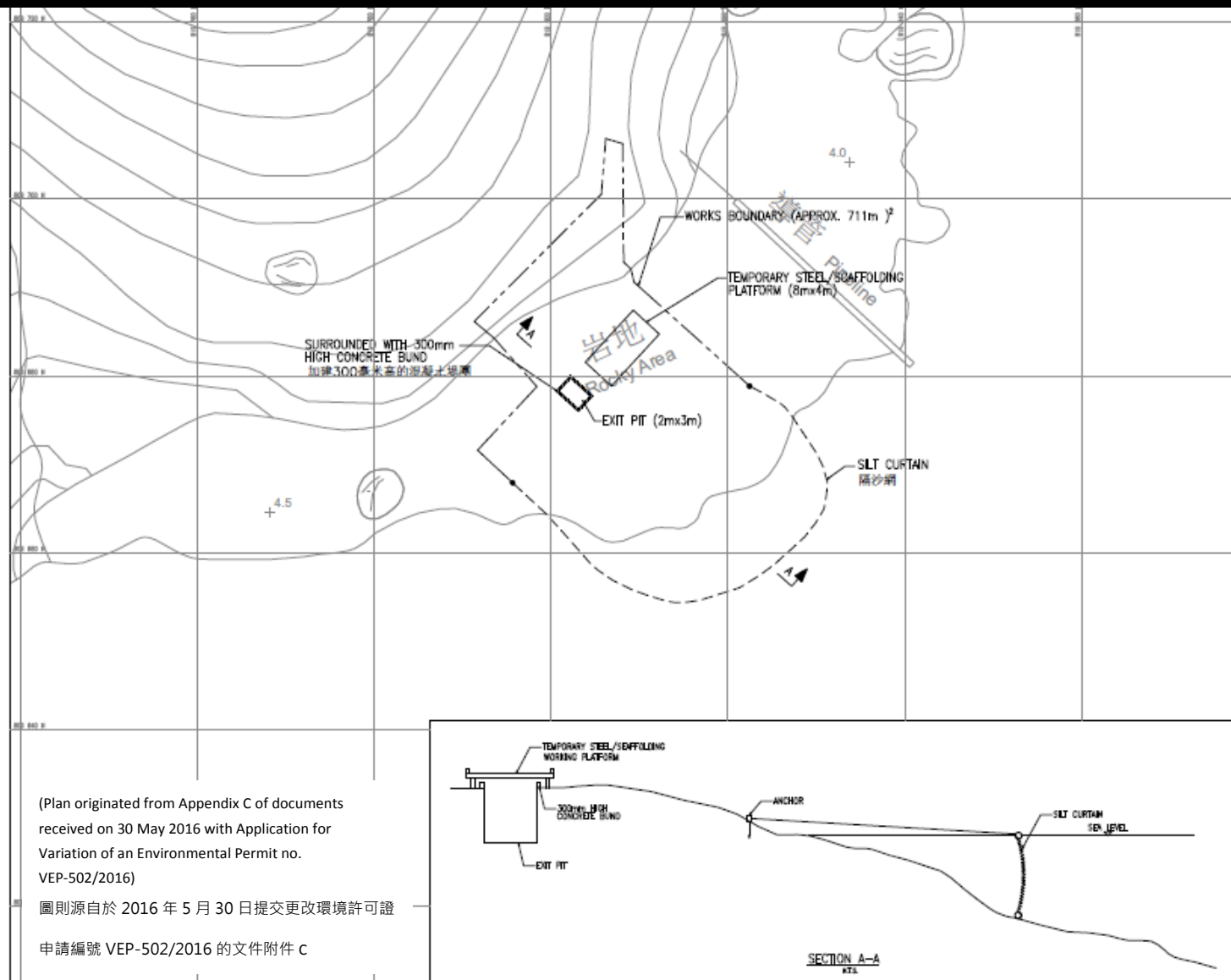
Figure 5: Schematic Layout and Silt Curtain Installation at Lantau Works Area
