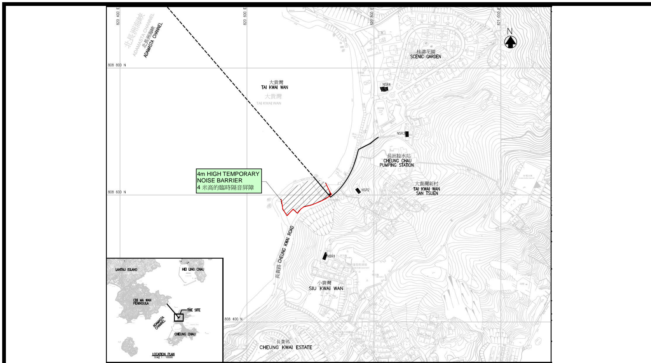
Figure 6: Location of Temporary Noise Barrier
