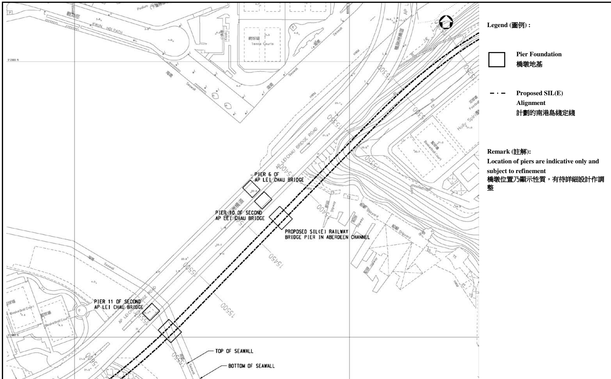
Figure 8: Railway Bridge Pier Foundation 圖 8: 鐵路橋的橋墩地基
