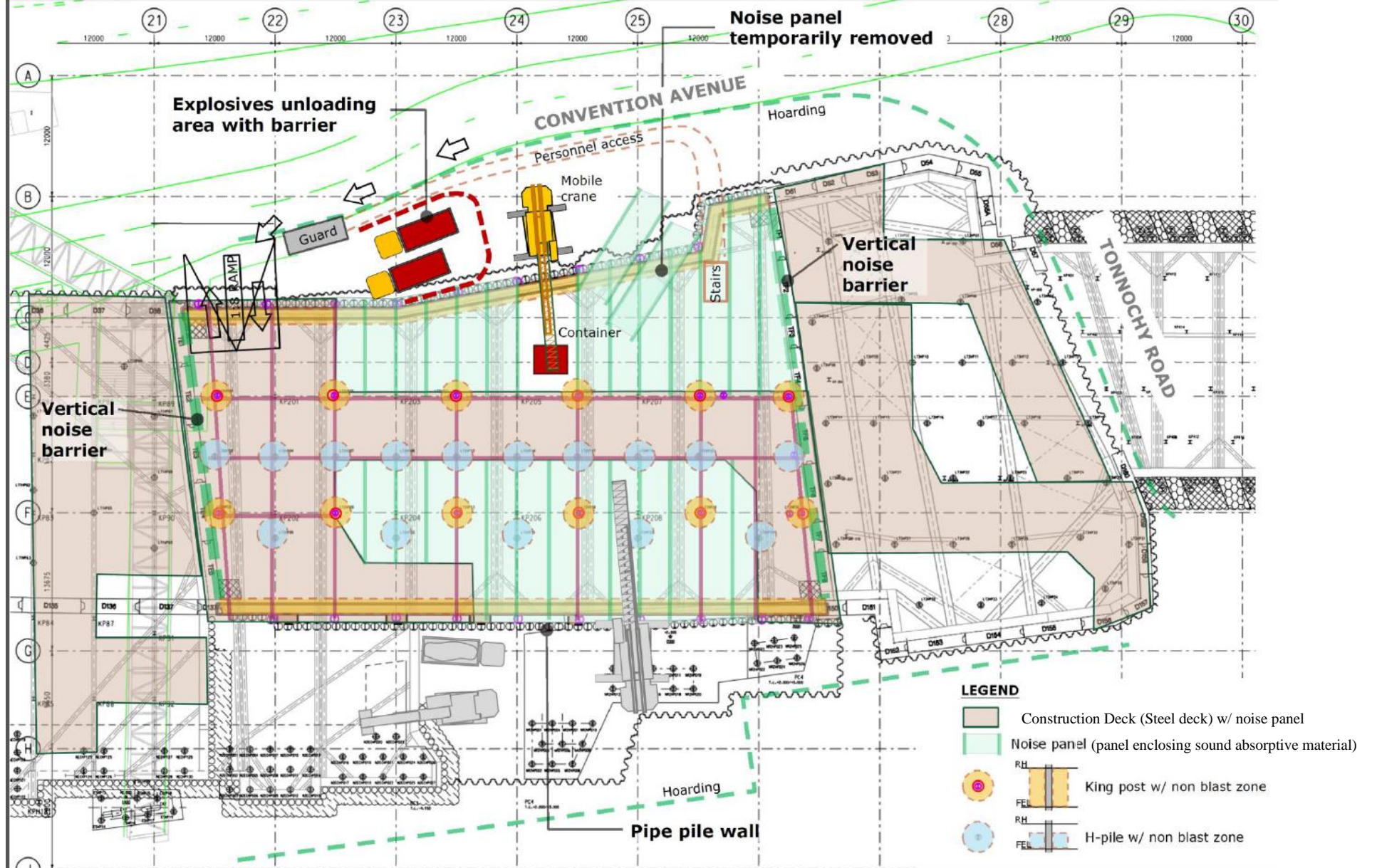
Figure 12: Indicative Design of the Noise Mitigation Measure at EXH Zone 2
