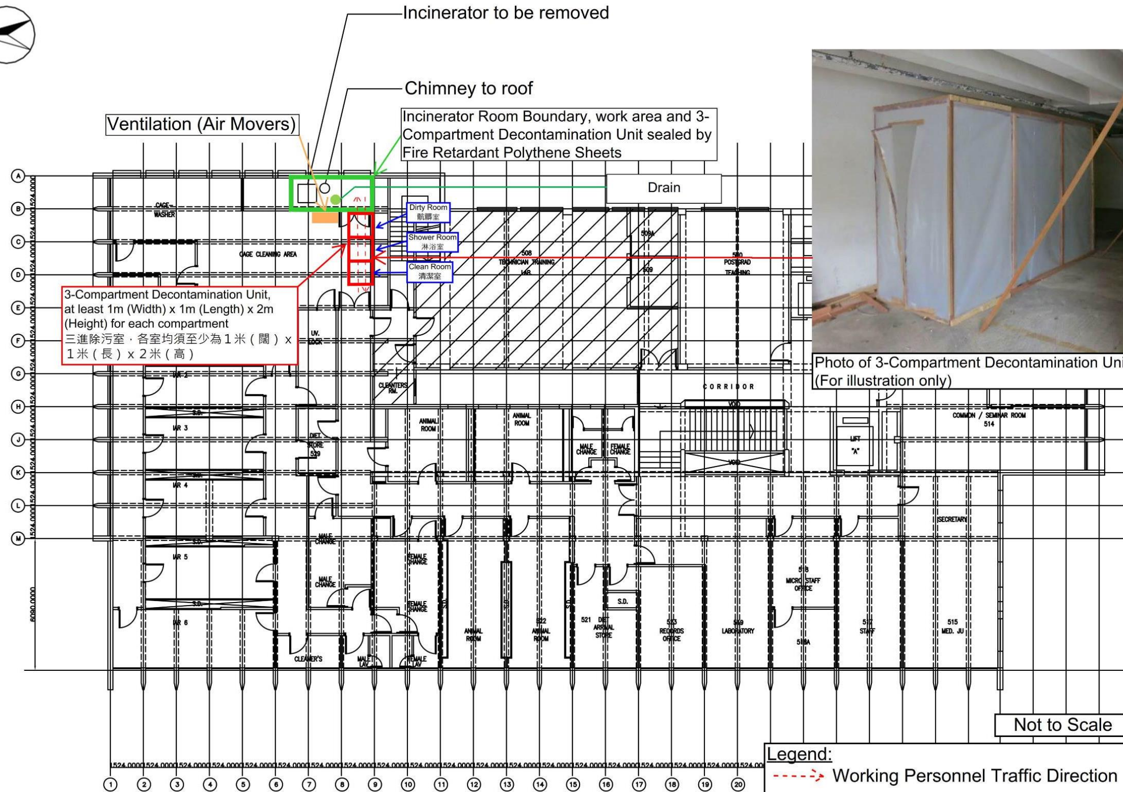
Figure 4: Floor Plan of the Incinerator Room in UPB
