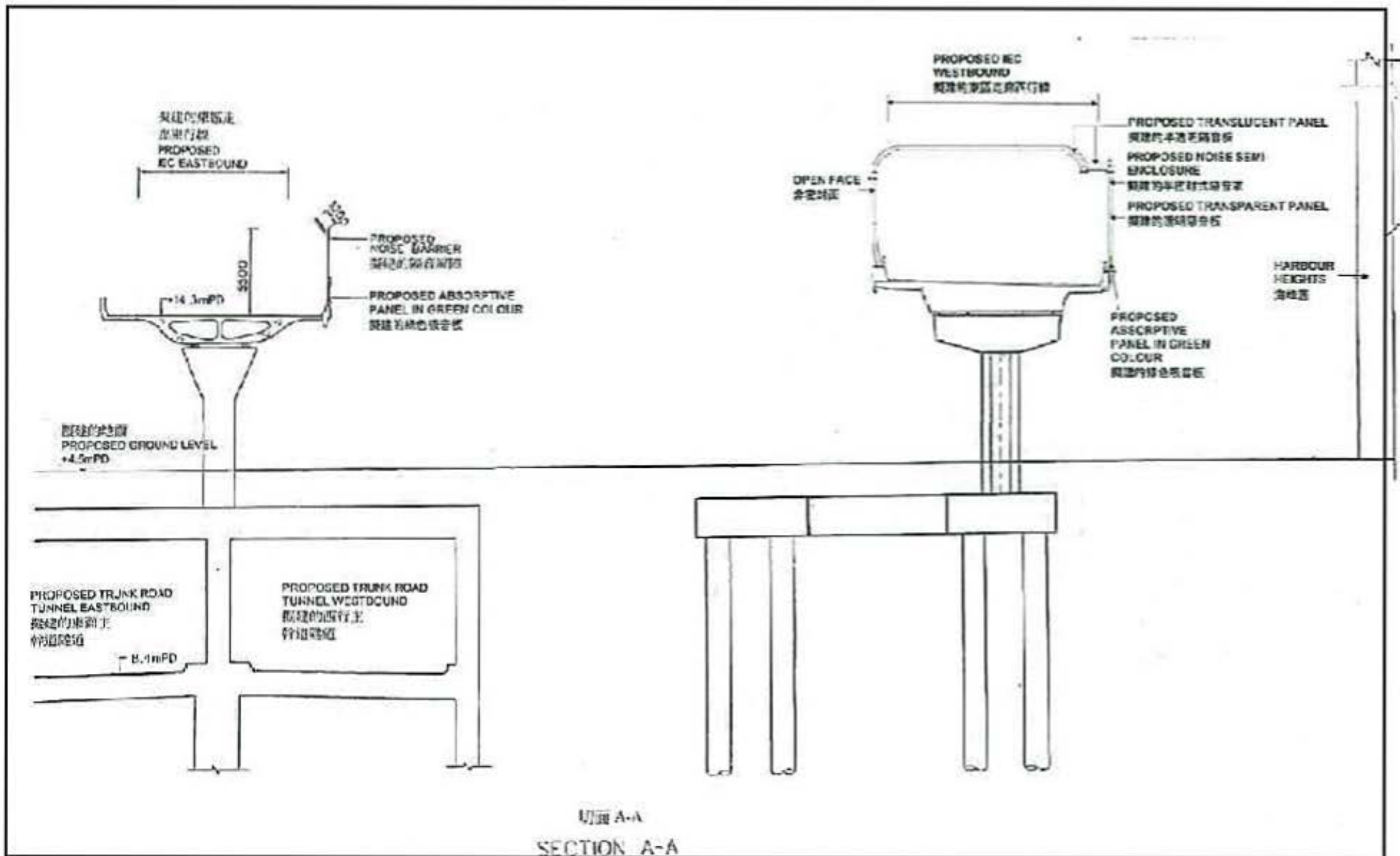
Figure 4c: Section of Direct Noise Mitigation Measures 圖 4c: 直接噪音緩解措施切面圖
