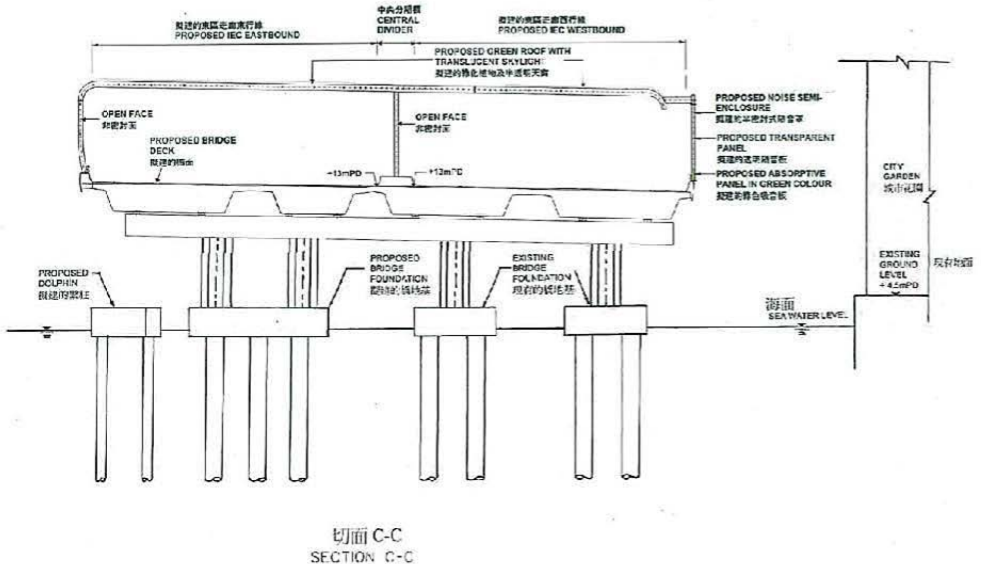
Figure 4e: Section of Direct Noise Mitigation Measures 圖 4e: 直接噪音緩解措施切面圖
