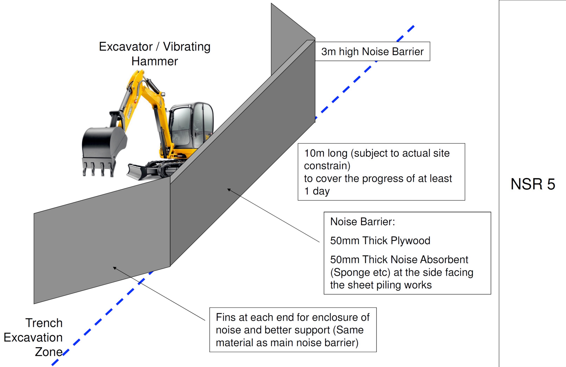
Figure 6 : Noise Barrier design
