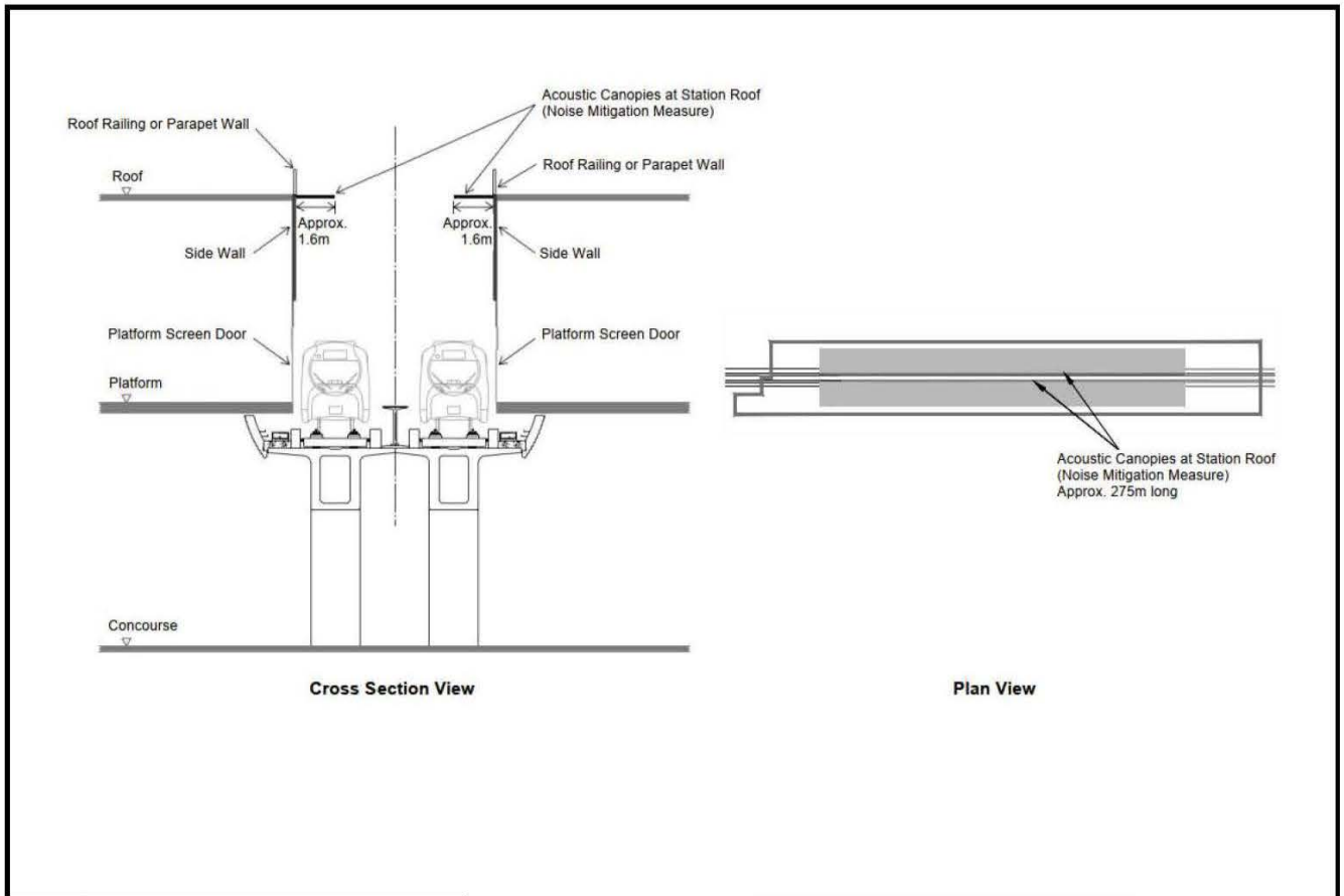
Figure 17 – Noise Mitigation Measures at Hung Shui Kiu Station
