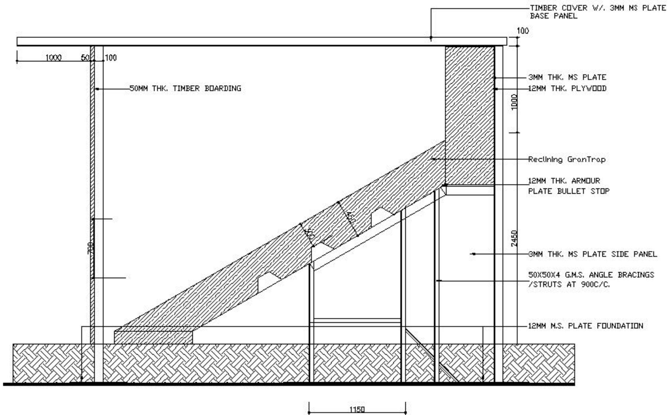
① TYPICAL DETAIL OF SHOOTING RANGE BULLET CATCHER D-01
