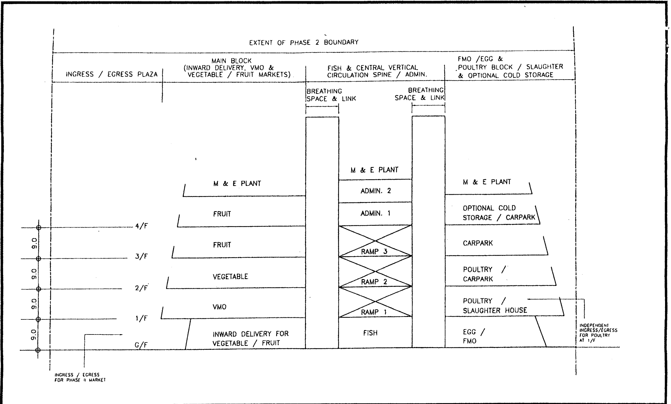
Project Boundary: Cheung Sha Wan Wholesale Market (Schematic Sectional Elevation)
