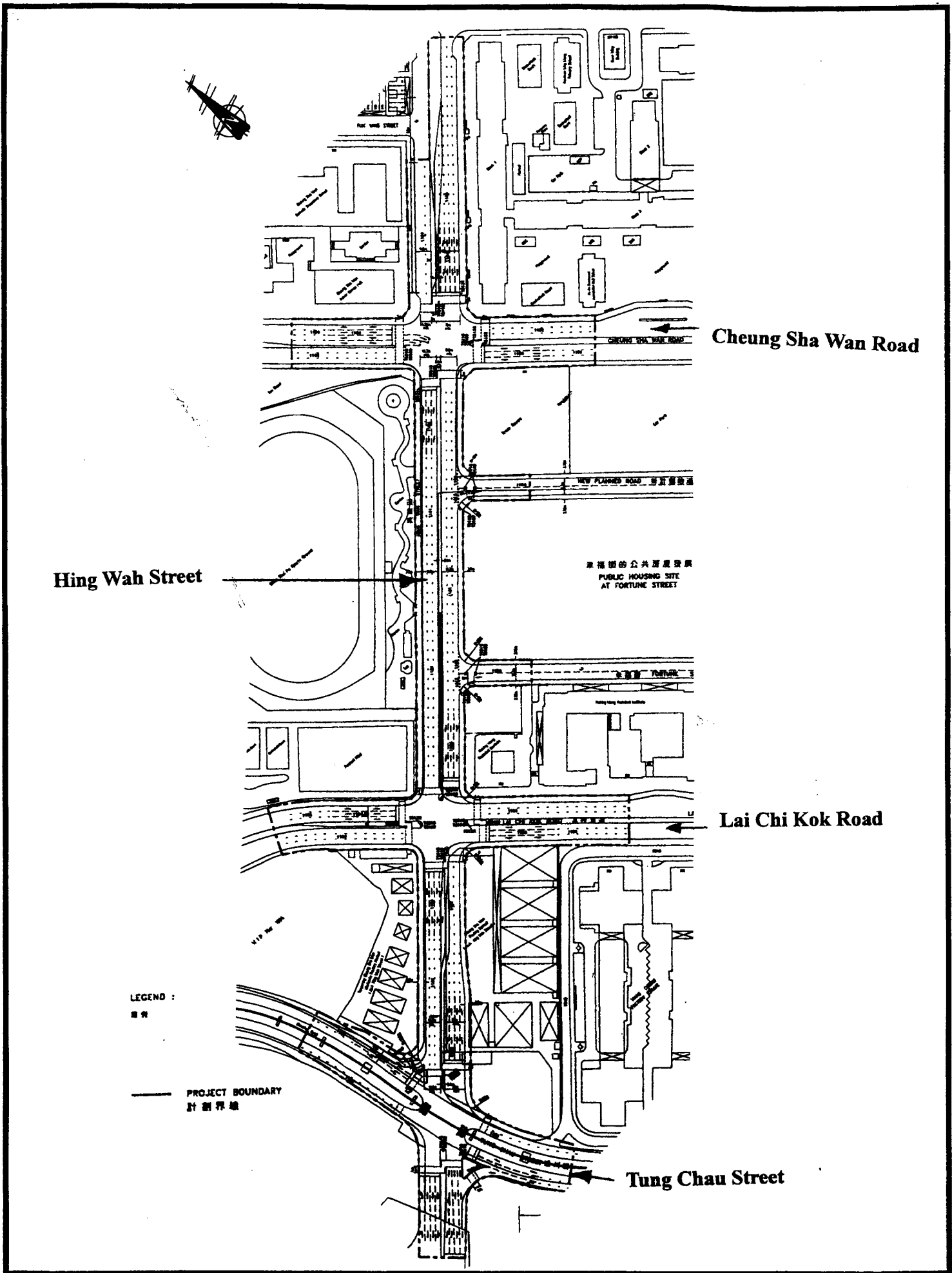
Road Widening of Hing Wah Street (Permanent Layout)
