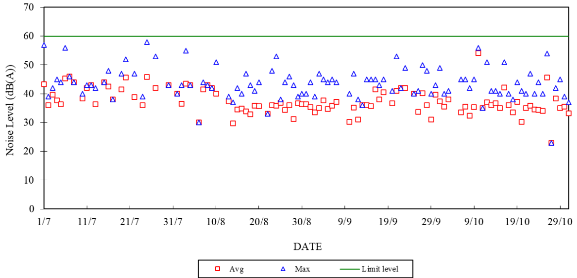
Construction Noise Monitoring in July 2025 - October 2025 NSR at Long Tsai Tsuen/Hung Shing Ye 07:00-23:00 hrs on Holidays and 19:00-23:00 hrs on All Other Days
