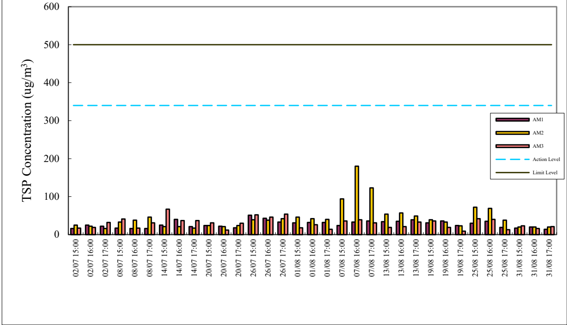
1-hr TSP Air Monitoring Data (July 2025 - August 2025)
