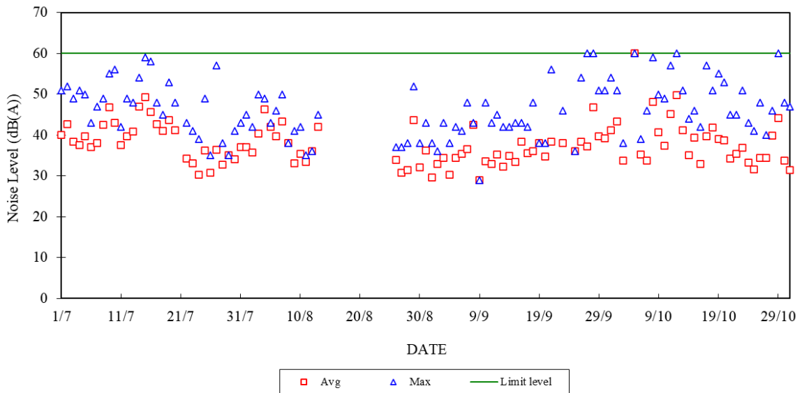
Construction Noise Monitoring in July 2025 - October 2025 NSR at School within Tai Wan San Tsuen 07:00-23:00 hrs on Holidays and 19:00-23:00 hrs on All Other Days
