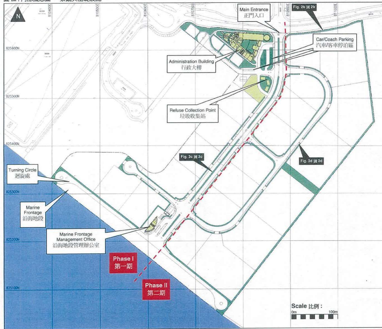
Figure 2a : Conceptual Internal Layout – Landscaping and Infrastructure
