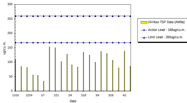
WIL-AM9a 24hr TSP Level at No. 28 Sai Woo Lane (Dec 2009 - Apr 2010)
