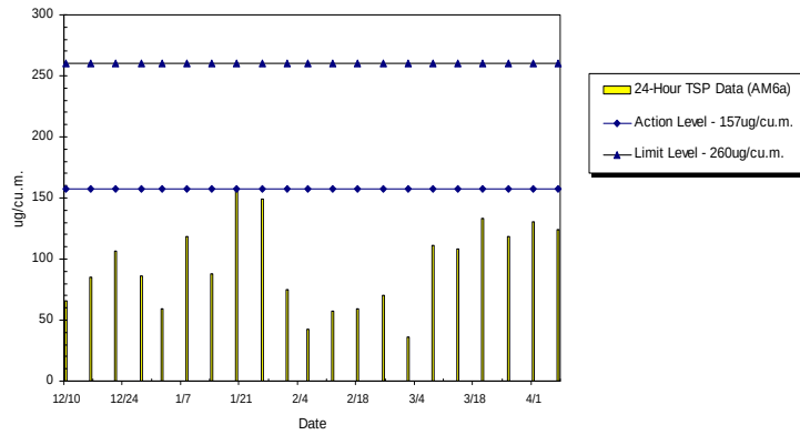
WIL-AM6a 24hr TSP Level at St. Paul's College Primary School (Dec 2009 - Apr 2010)
