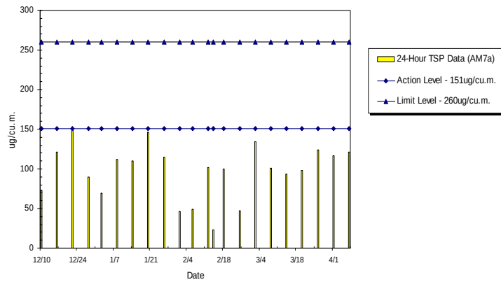
WIL-AM7a 24hr TSP Level at Hill Court (Dec 2009 - Apr 2010)
