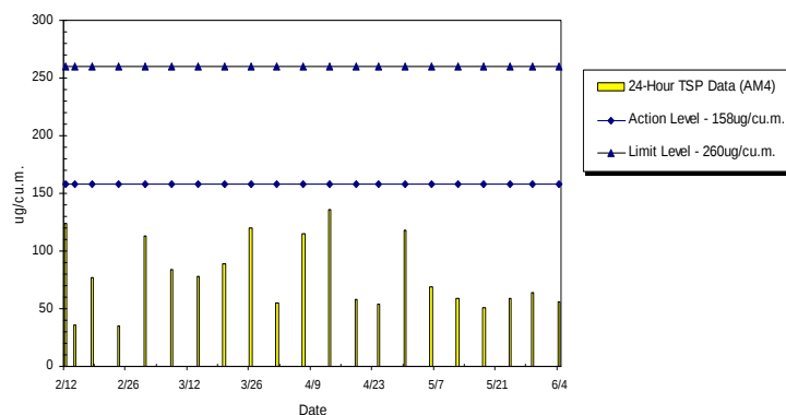
WIL-AM4 24hr TSP Level at Chee Sing Kok Social Centre (Feb 2010 - Jun 2010)
