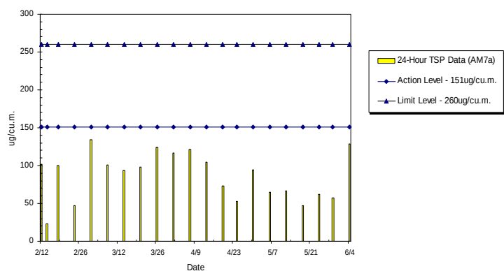
WIL-AM7a 24hr TSP Level at Hill Court (Feb 2010 - Jun 2010)
