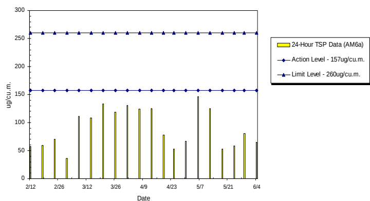
WIL-AM6a 24hr TSP Level at St. Paul's College Primary School (Feb 2010 - Jun 2010)
