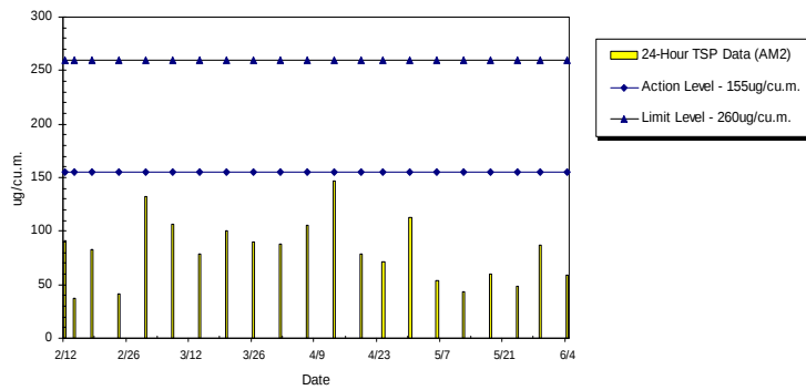
WIL-AM2 24hr TSP Level at Victoria Public Mortuary (Feb 2010 - Jun 2010)
