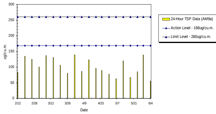
WIL-AM9a 24hr TSP Level at No. 28 Sai Woo Lane (Feb 2010 - Jun 2010)
