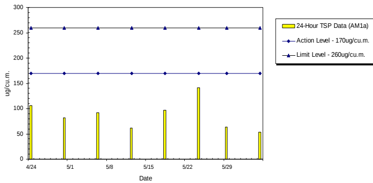
WIL-AM1a 24hr TSP Level at Kwun Lung Lau Block 1 (Apr 2010 - Jun 2010)
