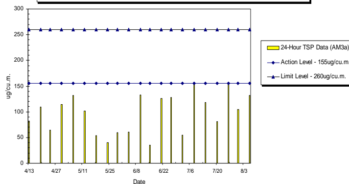
WIL-AM3a 24hr TSP Level at HK IVE (Tsing Yi) Kennedy Town Centre (Apr- Aug 2010)
