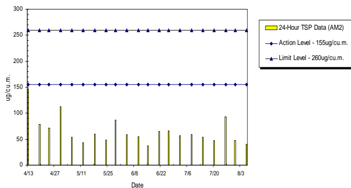
WIL-AM2 24hr TSP Level at Victoria Public Mortuary (Apr 2010 - Aug 2010)
