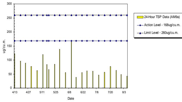
WIL-AM9a 24hr TSP Level at No. 28 Sai Woo Lane (Apr 2010 - Aug 2010)
