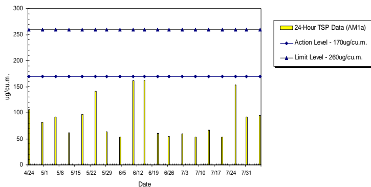
WIL-AM1a 24hr TSP Level at Kwun Lung Lau Block 1 (Apr 2010 - Aug 2010)
