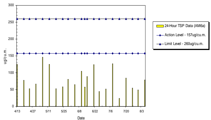
WIL-AM6a 24hr TSP Level at St. Paul's College Primary School (Apr 2010 - Aug 2010)
