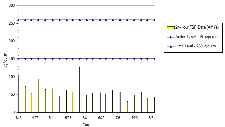
WIL-AM7a 24hr TSP Level at Hill Court (Apr 2010 - Aug 2010)
