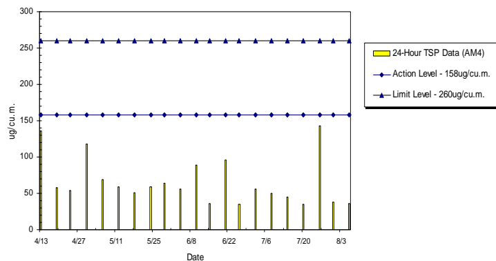
WIL-AM4 24hr TSP Level at Chee Sing Kok Social Centre (Apr 2010 - Aug 2010)
