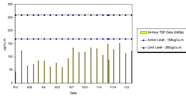
WIL-AM9a 24hr TSP Level at No. 28 Sai Woo Lane (Aug 2010 - Dec 2010)
