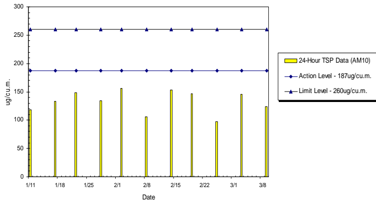
WIL-AM10 24hr TSP Level at Western Court, Ivy Tower (Jan 2011 - Mar 2011)
