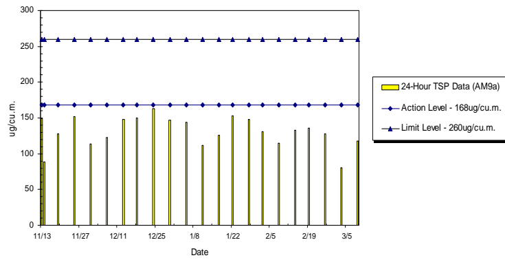
WIL-AM9a 24hr TSP Level at No. 28 Sai Woo Lane (Nov 2010 - Mar 2010)
