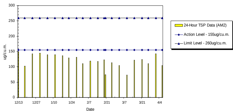
WIL-AM2 24hr TSP Level at Victoria Public Mortuary (Dec 2010 - Apr 2011)
