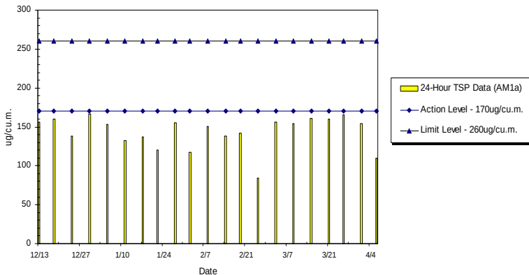
WIL-AM1a 24hr TSP Level at Kwun Lung Lau Block 1 (Dec 2010 - Apr 2011)
