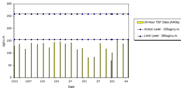
WIL-AM3a 24hr TSP Level at HK IVE (Tsing Yi) Kennedy Town Centre (Dec 2010 - Apr 2011)
