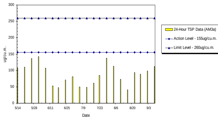
WIL-AM3a 24hr TSP Level at HK IVE (Tsing Yi) Kennedy Town Centre (May 2011 - Sep 2011)
