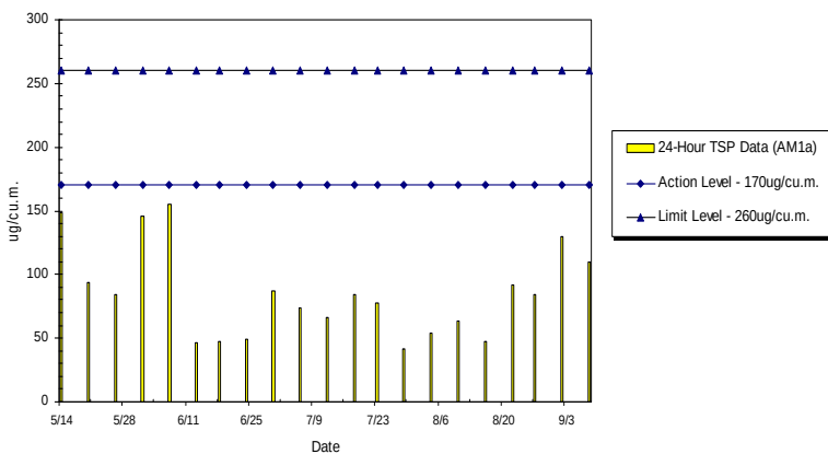
WIL-AM1a 24hr TSP Level at Kwun Lung Lau Block 1 (May 2011 - Sep 2011)
