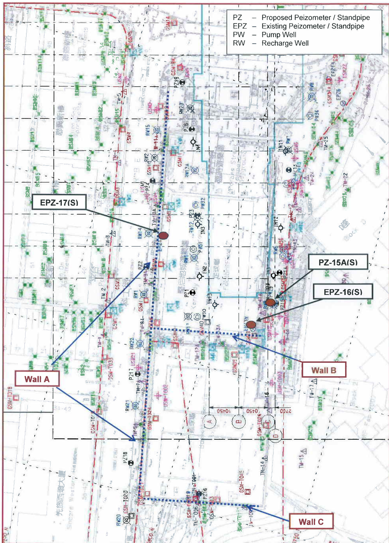
Figure 1 : Location of Standpipe/Piezometers, Pump Wells, Recharge Wells Installed on Site
