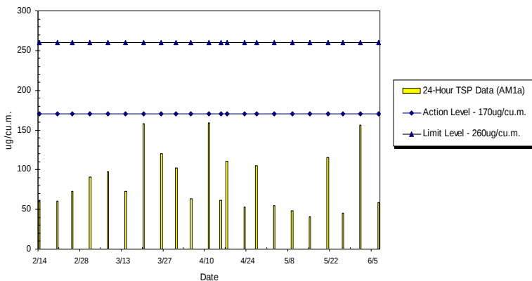
WIL-AM1a 24hr TSP Level at Kwun Lung Lau Block 1 (Feb 2012 - Jun 2012)
