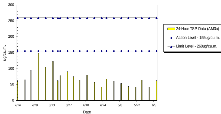
WIL-AM3a 24hr TSP Level at HK IVE (Tsing Yi) Kennedy Town Centre (Feb 2012 - Jun 2012)
