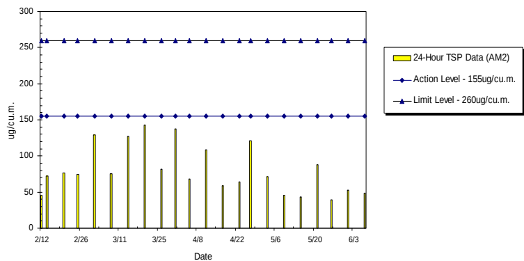
WIL-AM2 24hr TSP Level at Victoria Public Mortuary (Feb 2012 - Jun 2012)
