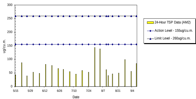
WIL-AM2 24hr TSP Level at Victoria Public Mortuary (May 2012 - Sept 2012)
