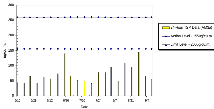
WIL-AM3a 24hr TSP Level at HK IVE (Tsing Yi) Kennedy Town Centre (May 2012 - Sept 2012)
