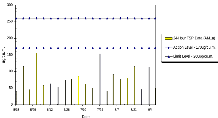
WIL-AM1a 24hr TSP Level at Kwun Lung Lau Block 1 (May 2012 - Sept 2012)
