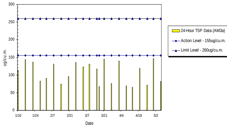
WIL-AM3a 24hr TSP Level at HK IVE (Tsing Yi) Kennedy Town Centre (Jan 2013 - May 2013)
