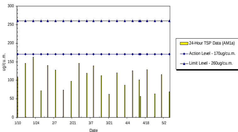
WIL-AM1a 24hr TSP Level at Kwun Lung Lau Block 1 (Jan 2013 - May 2013)
