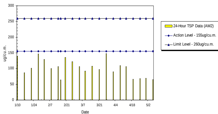
WIL-AM2 24hr TSP Level at Victoria Public Mortuary (Jan 2013 - May 2013)
