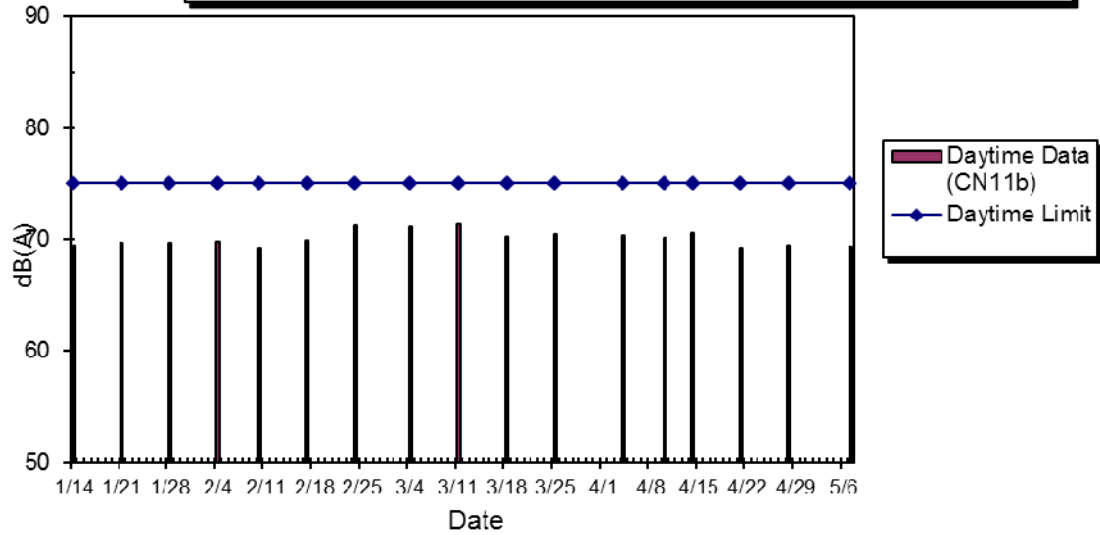
WIL-CN11b Noise Level at The Belcher's Tower 8, Jan 2014 - May 2013
