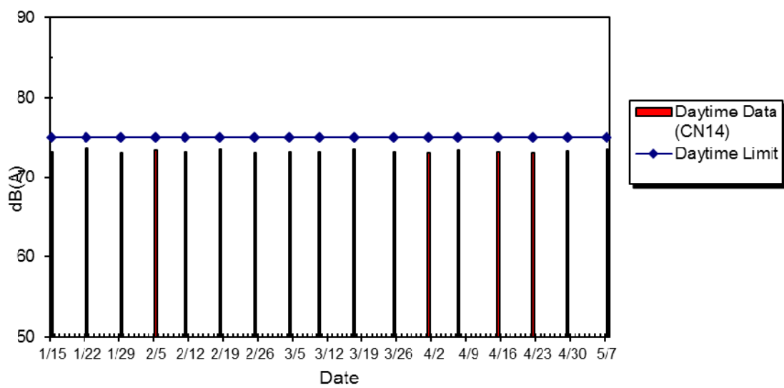
WIL-CN14 Noise Level at Bon-Point, Jan 2014 - May 2014
