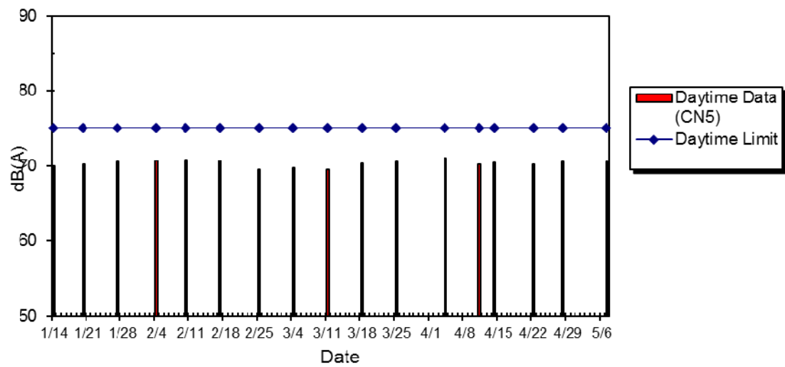
WIL-CN5 Noise Level at Western Court, Jan 2014 - May 2014
