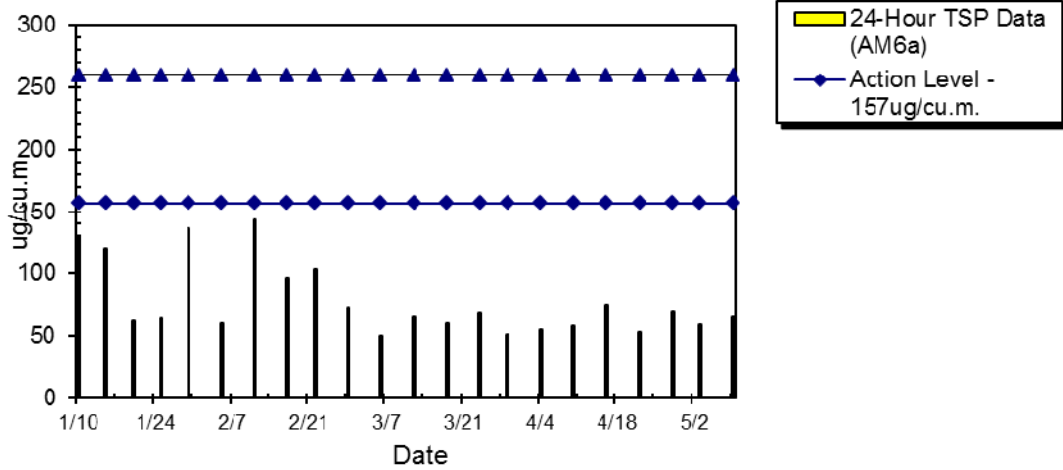
WIL-AM6a 24hr TSP Level at St. Paul's College Primary School (Jan 2014 - May 2014)
