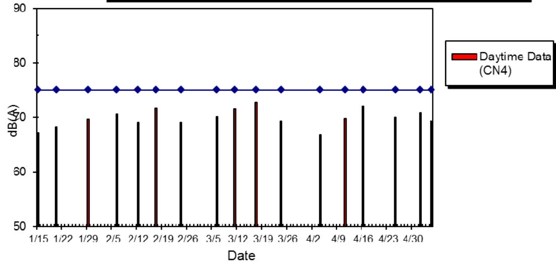
WIL-CN4 Noise Level at Luen Tak Apartments, Jan 2014 - May 2014
