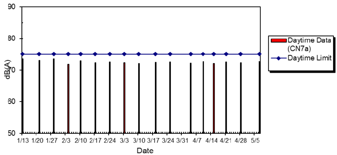
WIL-CN7a Noise Level at Bowie Court, Jan 2014 - May 2014
