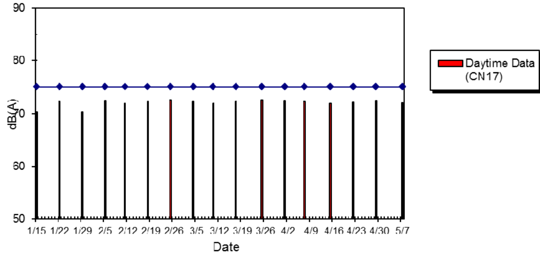
WIL-CN17 Noise Level at No.1 Third Street, Jan 2014 - May 2014
