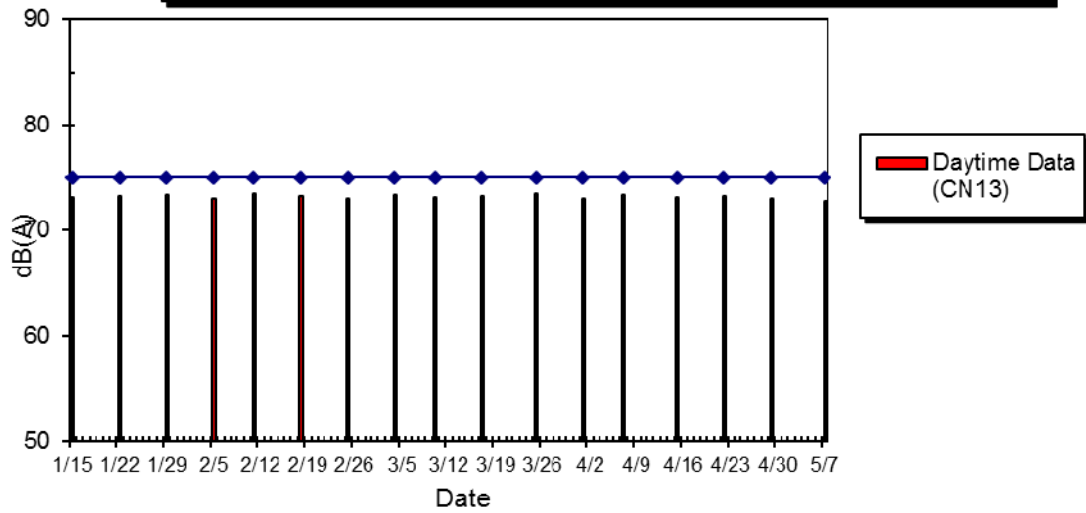
WIL-CN13 Noise Level at No.18-20 Eastern Street, Jan 2014 - May 2014
