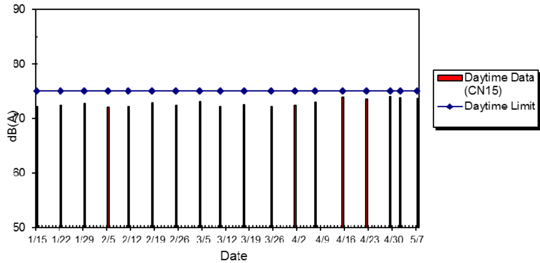
WIL-CN15 Noise Level at Ivy Tower, Jan 2014 - May 2014
