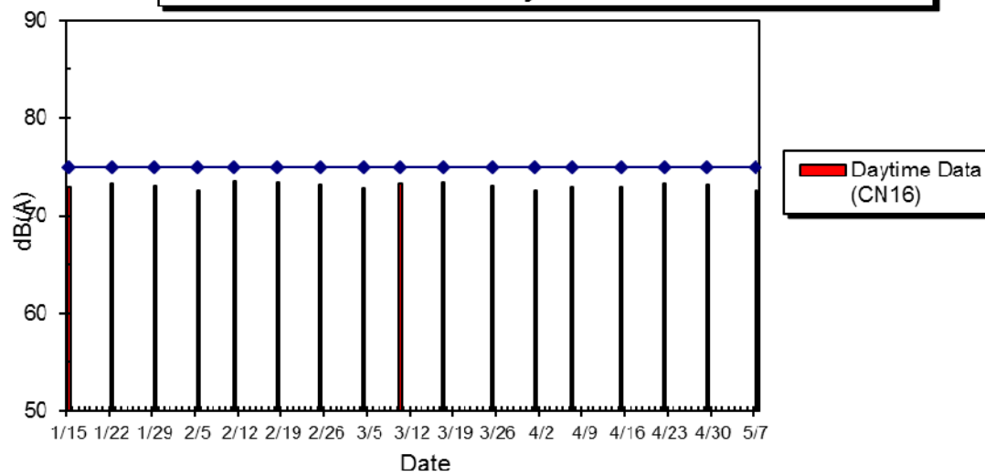
WIL-CN16 Noise Level at No.9-11 Ki Ling Lane, Jan 2014 - May 2014
