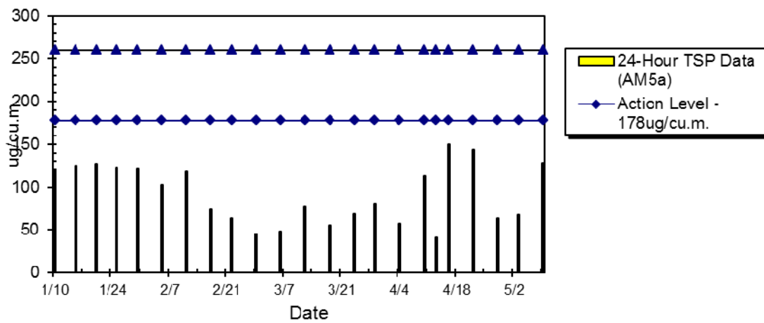
WIL-AM5a 24hr TSP Level at Kennedy Town Fire Station (Jan 2014 - May 2014)
