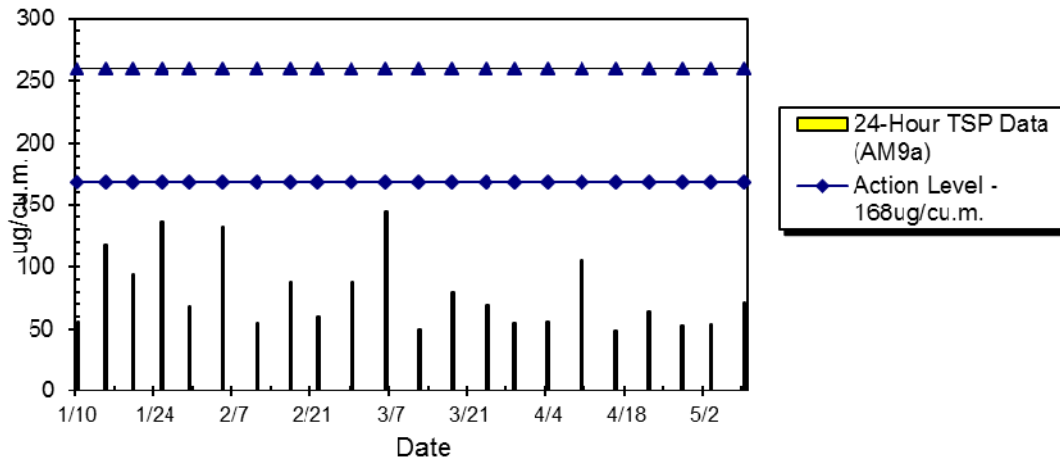
WIL-AM9a 24hr TSP Level at No. 28 Sai Woo Lane (Jan 2014 - May 2014)
