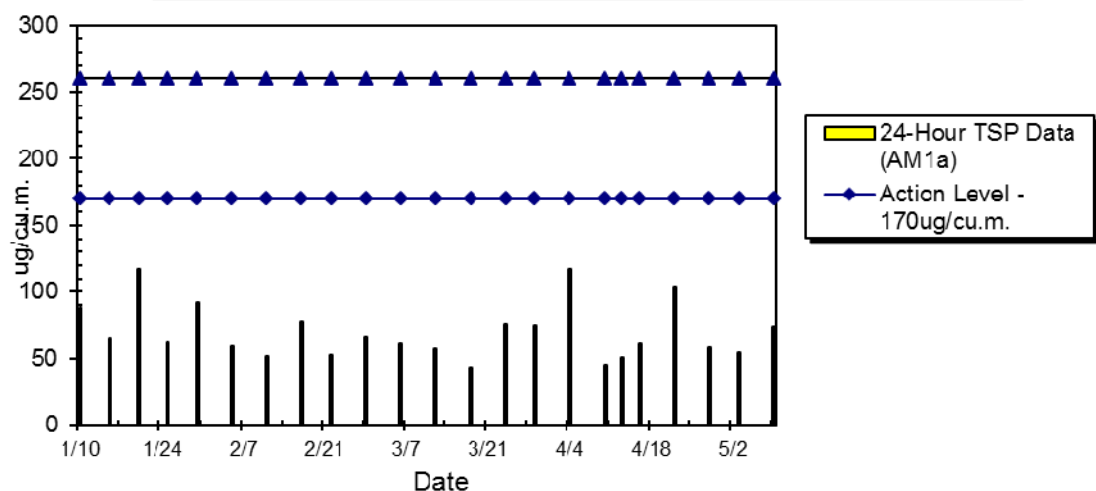
WIL-AM1a 24hr TSP Level at Kwun Lung Lau Block 1 (Jan 2014 - May 2014)
