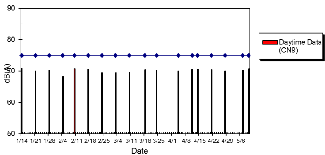
WIL-CN9 Noise Level at Hill Court, Jan 2014 - May 2014
