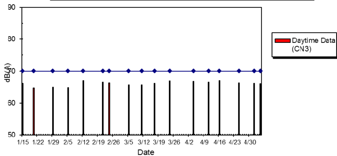
WIL-CN3 Noise Level at Lui Ming Choi Primary School, Jan 2014 - May 2014
