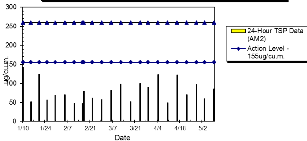
WIL-AM2 24hr TSP Level at Victoria Public Mortuary (Jan 2014 - May 2014)
