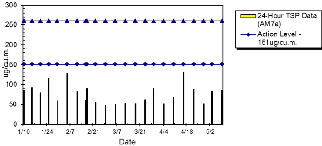
WIL-AM7a 24hr TSP Level at Hill Court (Jan 2014 - May 2014)
