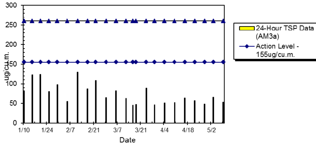
WIL-AM3a 24hr TSP Level at HK IVE (Tsing Yi) Kennedy Town Centre (Jan 2014 - May 2014)
