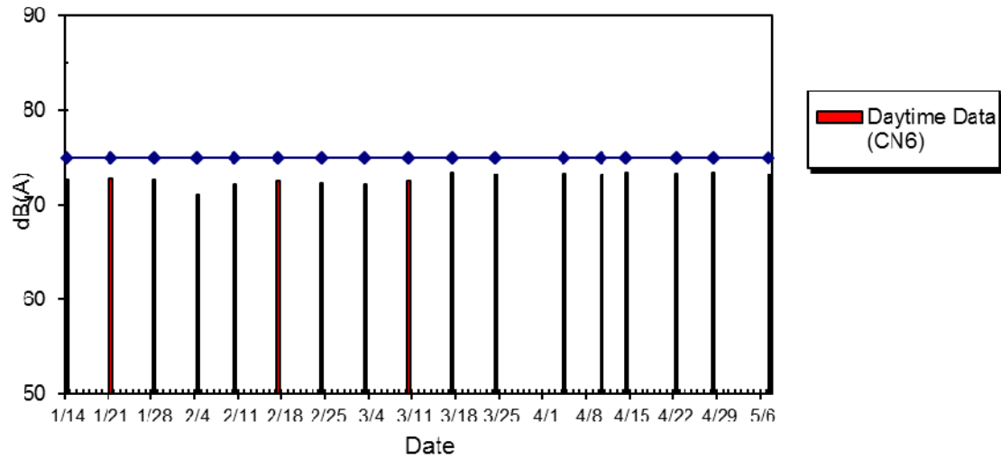
WIL-CN6 Noise Level at Yick Fung Garden (Block A), Jan 2014 - May 2014
