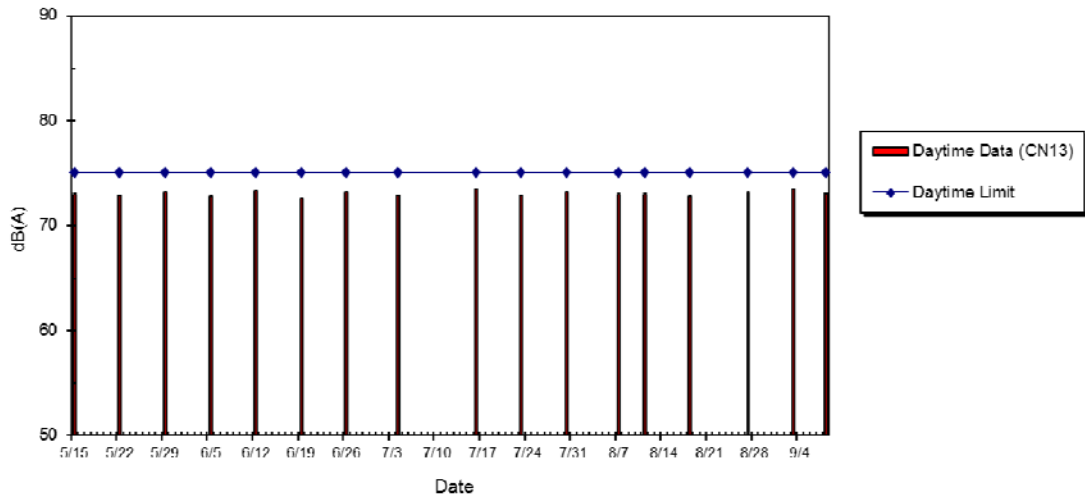
WIL-CN13 Noise Level at No.18-20 Eastern Street, May 2014 - Sept 2014
