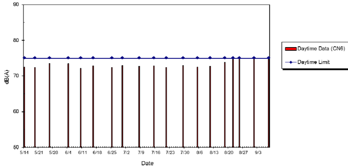
WIL-CN6 Noise Level at Yick Fung Garden (Block A), May 2014 - Sept 2014
