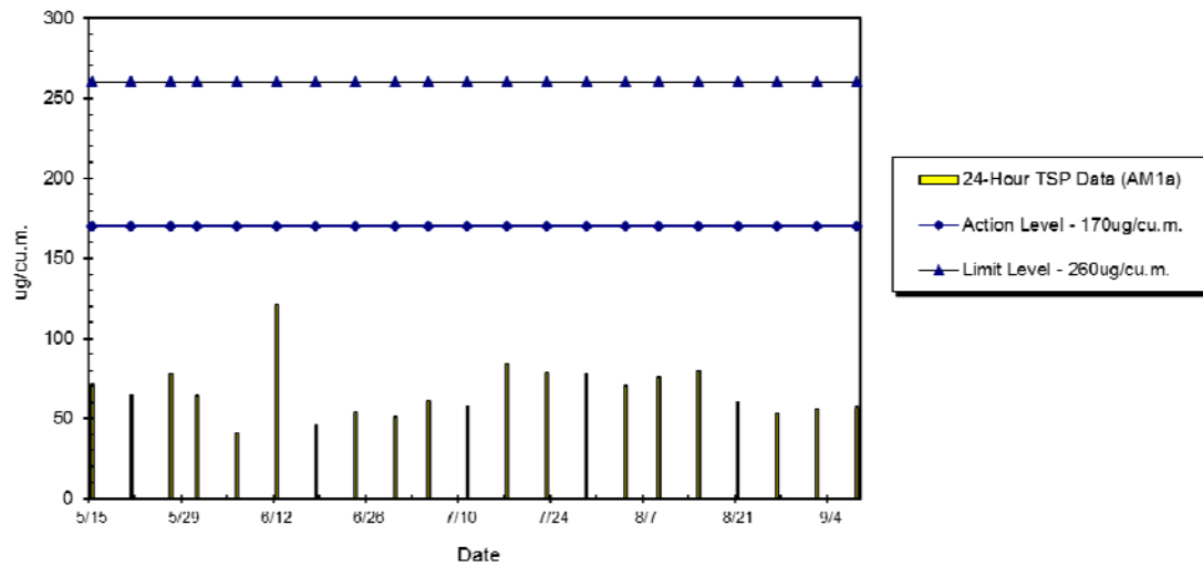
WIL-AM1a 24hr TSP Level at Kwun Lung Lau Block 1 (May 2014 - Sept 2014)
