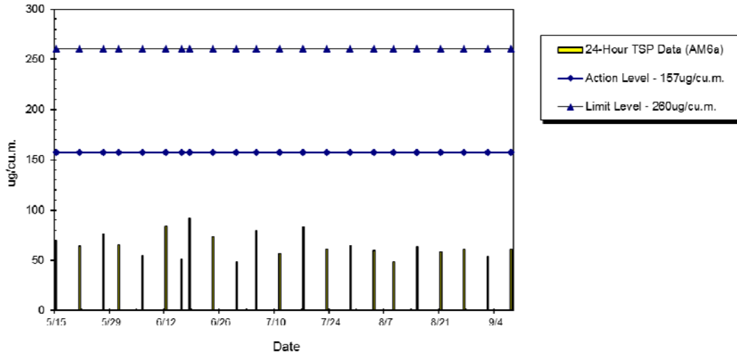
WIL-AM6a 24hr TSP Level at St. Paul's College Primary School (May 2014 - Sept 2014)
