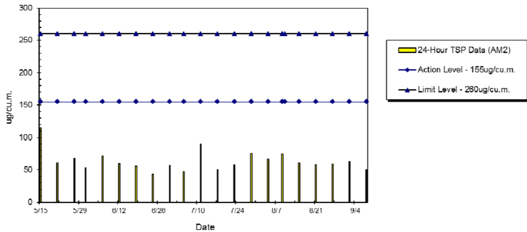
WIL-AM2 24hr TSP Level at Victoria Public Mortuary (May 2014 - Sept 2014)
