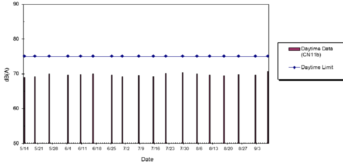
WIL-CN11b Noise Level at The Belcher's Tower 8, May 2014 - Sept 2014
