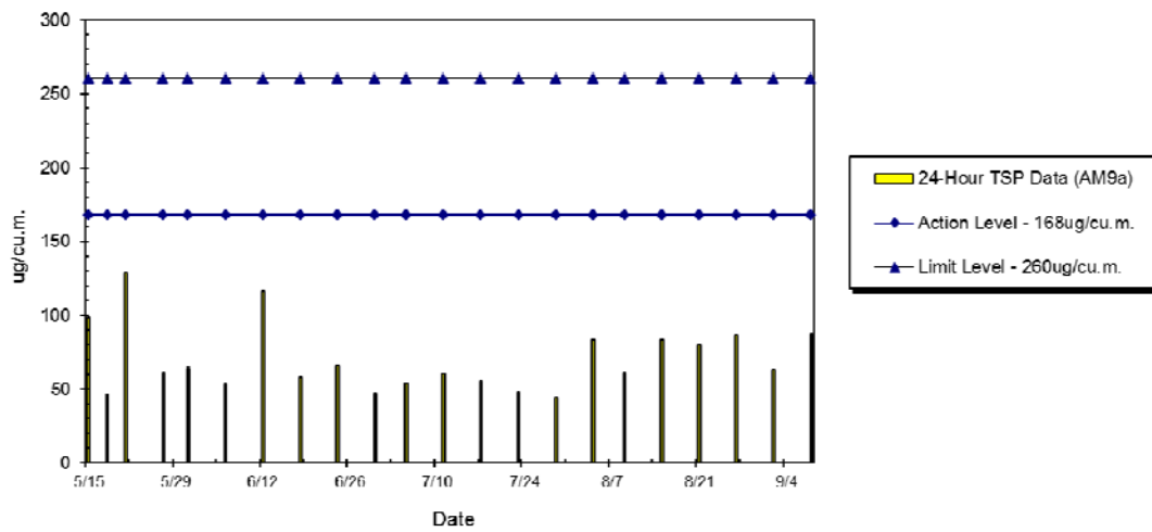
WIL-AM9a 24hr TSP Level at No. 28 Sai Woo Lane (May 2014 - Sept 2014)
