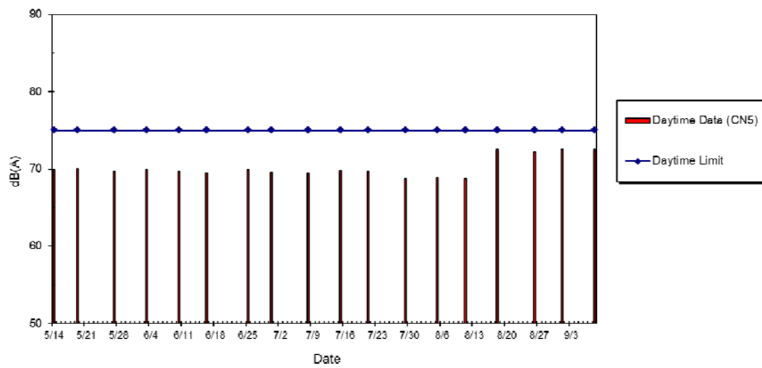
WIL-CN5 Noise Level at Western Court, May 2014 - Sept 2014
