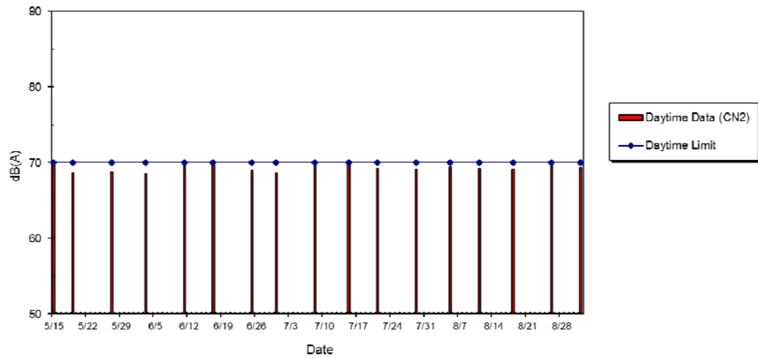
WIL-CN2 Noise Level at HK IVE (Tsing Yi) Kennedy Town Centre, May 2014 - Sept 2014
