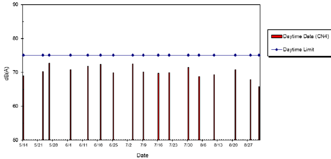
WIL-CN4 Noise Level at Luen Tak Apartments, May 2014 - Sept 2014
