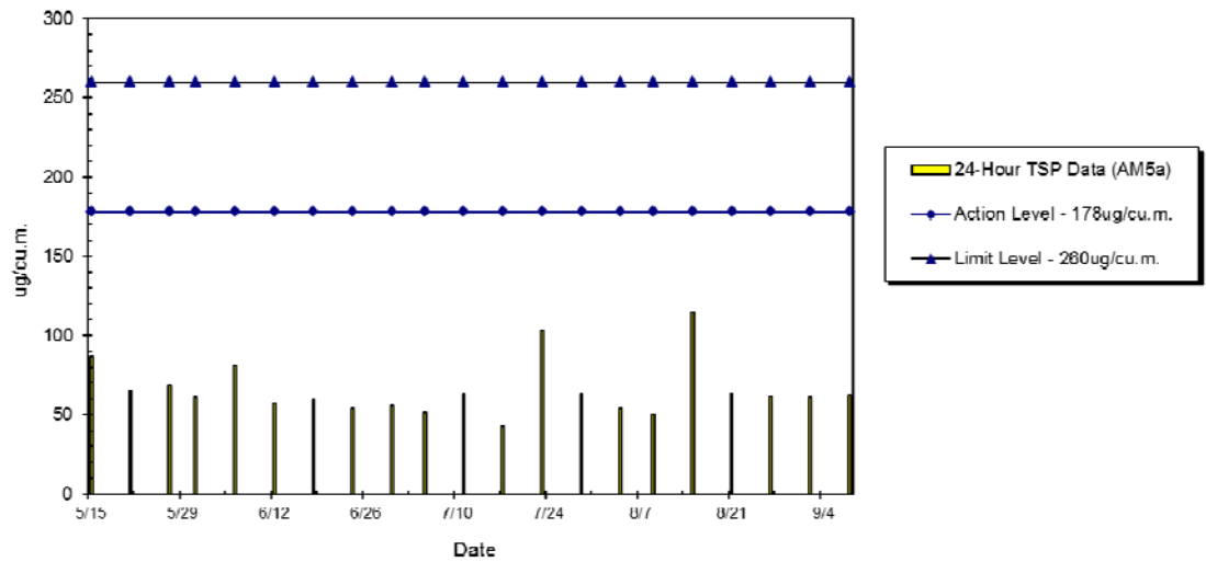
WIL-AM5a 24hr TSP Level at Kennedy Town Fire Station (May 2014 - Sept 2014)
