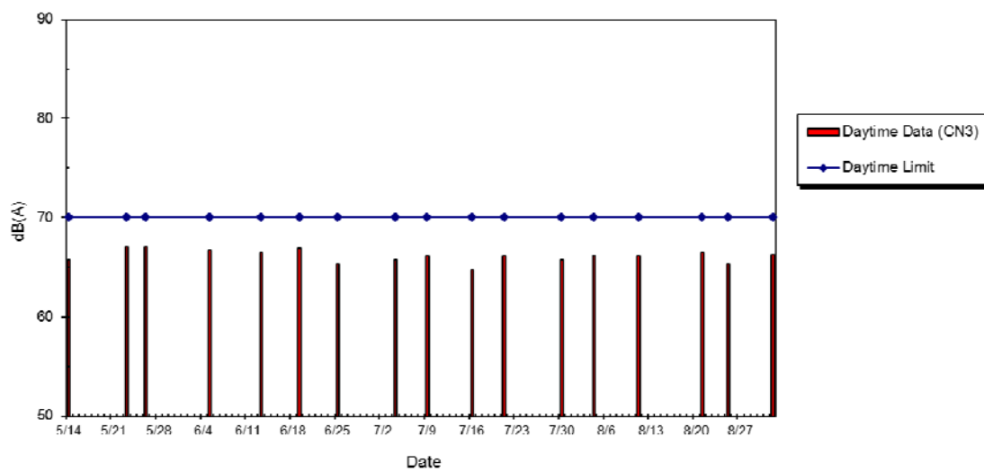
WIL-CN3 Noise Level at Lui Ming Choi Primary School, May 2014 - Sept 2014
