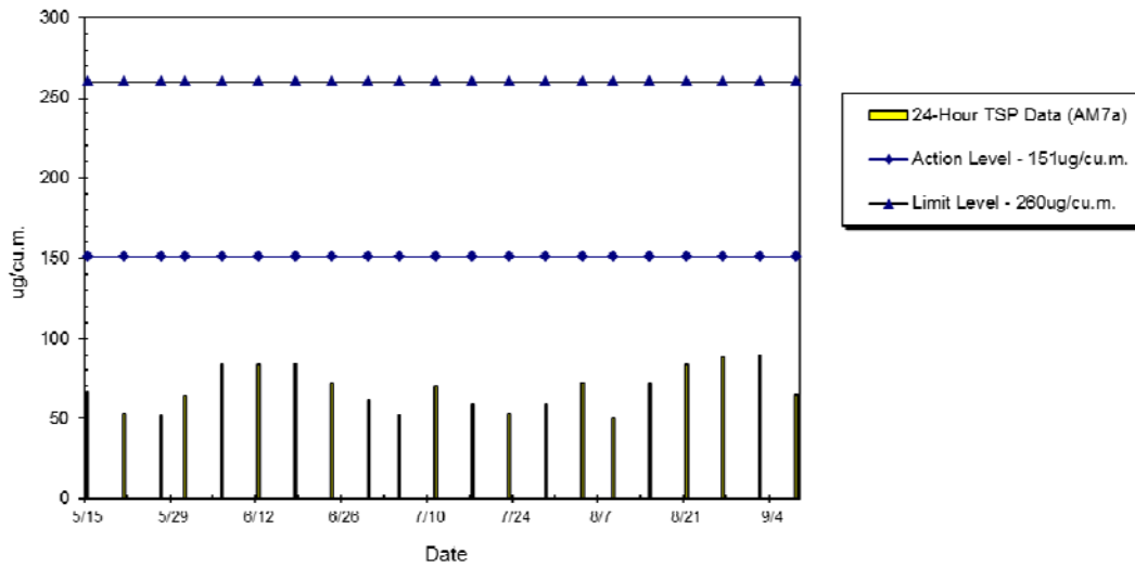
WIL-AM7a 24hr TSP Level at Hill Court (May 2014 - Sept 2014)
