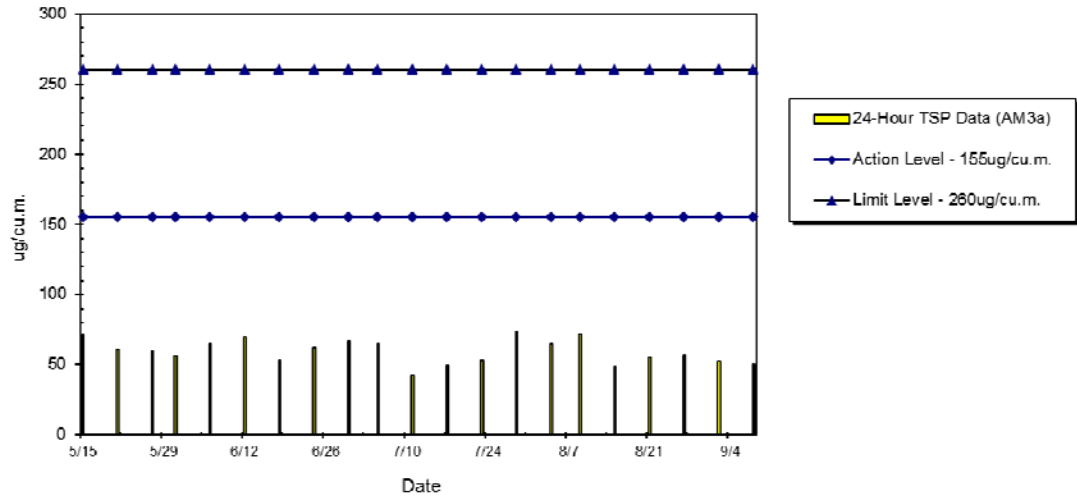
WIL-AM3a 24hr TSP Level at HK IVE (Tsing Yi) Kennedy Town Centre (May 2014 - Sept 2014)
