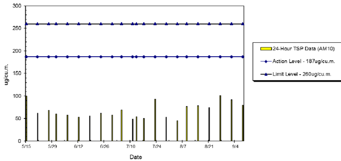
WIL-AM10 24hr TSP Level at Western Court, Ivy Tower (May 2014 - Sept 2014)
