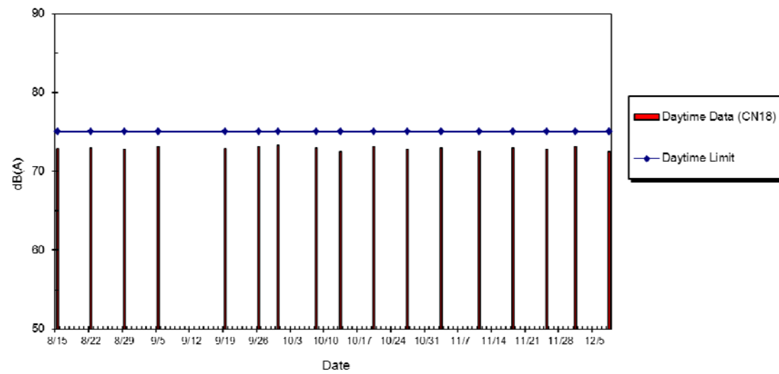
WIL-CN18 Noise Level at Princeton Tower, Aug 2014 - Dec 2014
