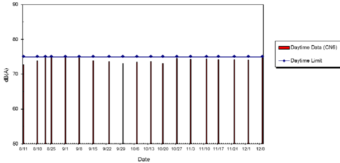
WIL-CN6 Noise Level at Yick Fung Garden (Block A), Aug 2014 - Dec 2014
