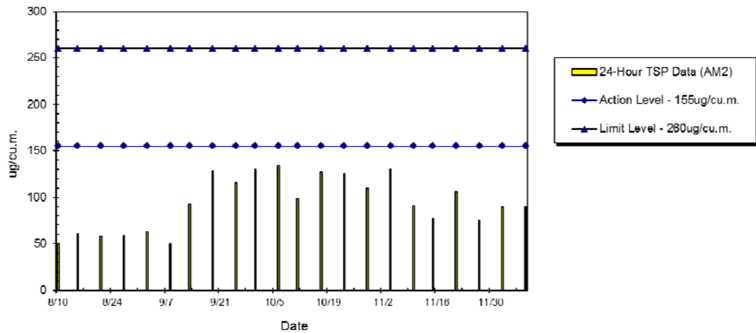
WIL-AM2 24hr TSP Level at Victoria Public Mortuary (Aug 2014 - Dec 2014)
