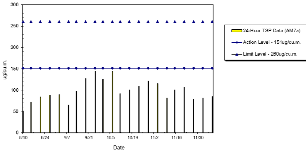
WIL-AM7a 24hr TSP Level at Hill Court (Aug 2014 - Dec 2014)
