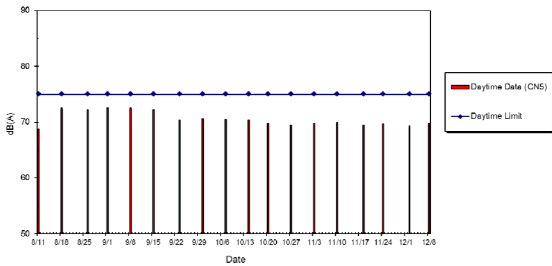
WIL-CN5 Noise Level at Western Court, Aug 2014 - Dec 2014
