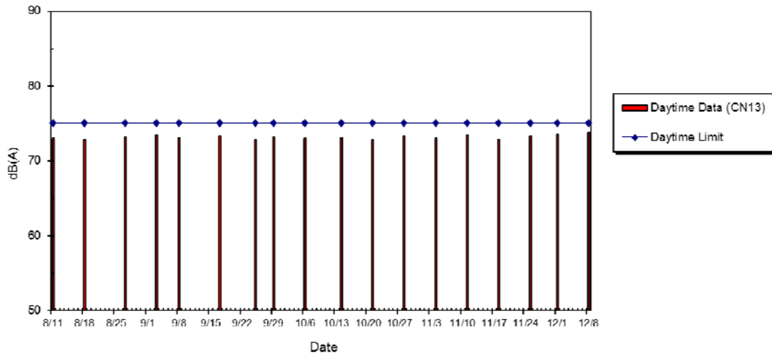
WIL-CN13 Noise Level at No.18-20 Eastern Street, Aug 2014 - Dec 2014
