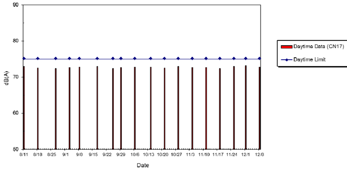
WIL-CN17 Noise Level at No.1 Thlrd Street, Aug 2014 - Dec 2014
