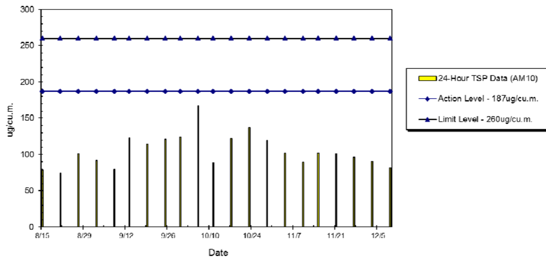
WIL-AM10 24hr TSP Level at Western Court, Ivy Tower (Aug 2014 - Dec 2014)
