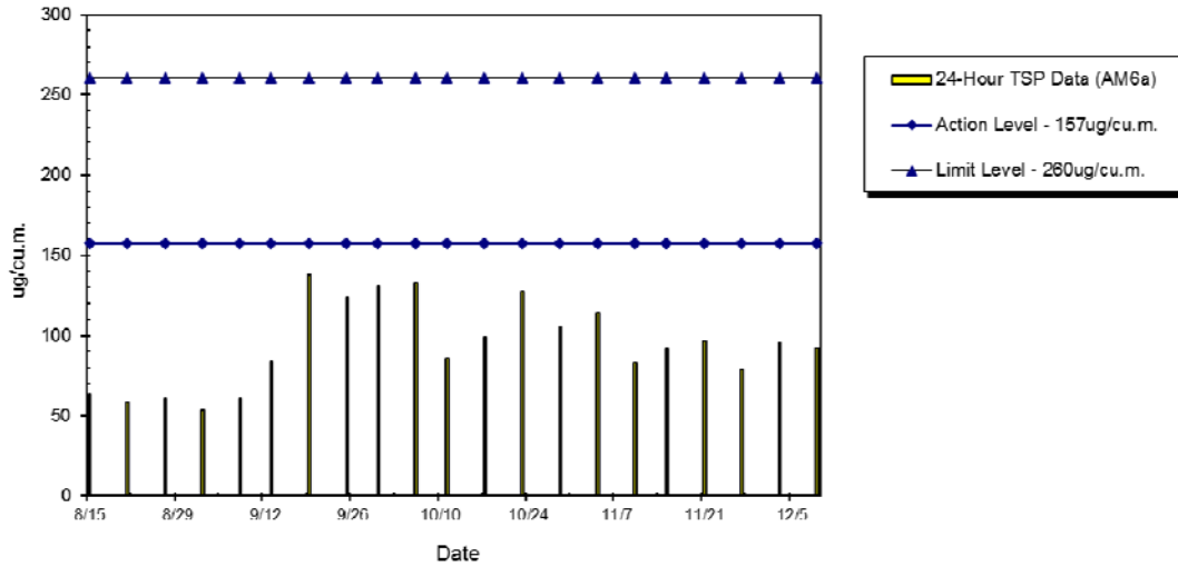
WIL-AM6a 24hr TSP Level at St. Paul's College Primary School (Aug 2014 - Dec 2014)
