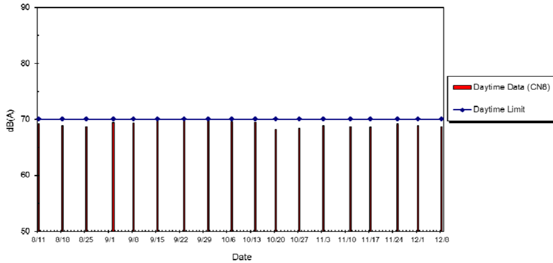
WIL-CN8 Noise Level at St. Paul's College Primary School, Aug 2014 - Dec 2014
