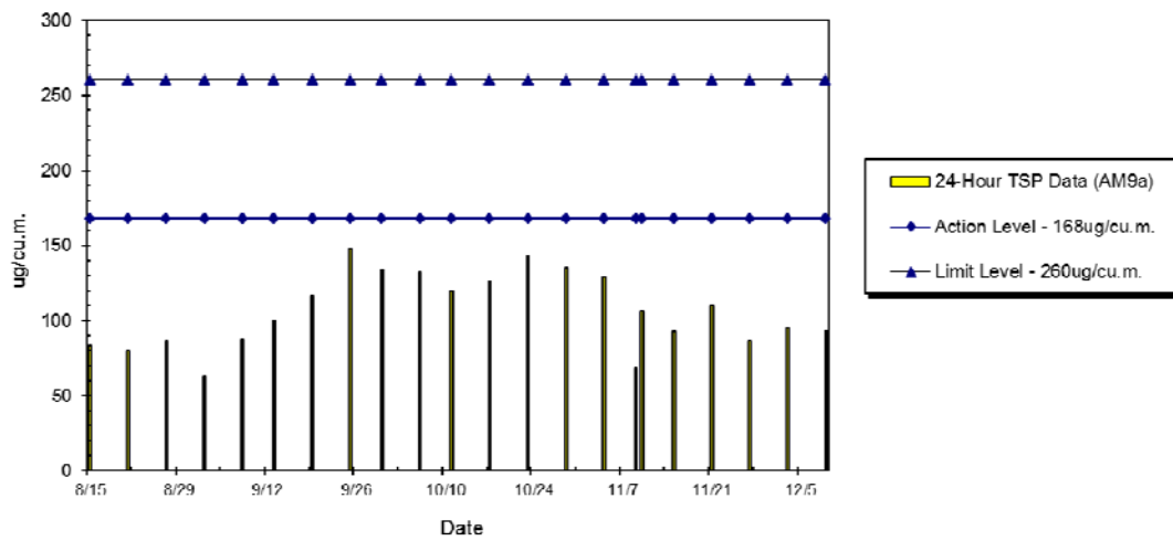
WIL-AM9a 24hr TSP Level at No. 28 Sai Woo Lane (Aug 2014 - Dec 2014)
