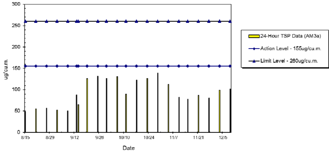
WIL-AM3a 24hr TSP Level at HK IVE (Tsing Yi) Kennedy Town Centre (Aug 2014 - Dec 2014)
