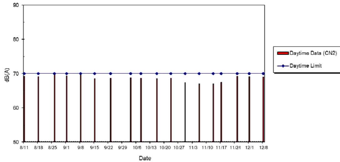
WIL-CN2 Noise Level at HK IVE (Tsing Yi) Kennedy Town Centre, Aug 2014 - Dec 2014
