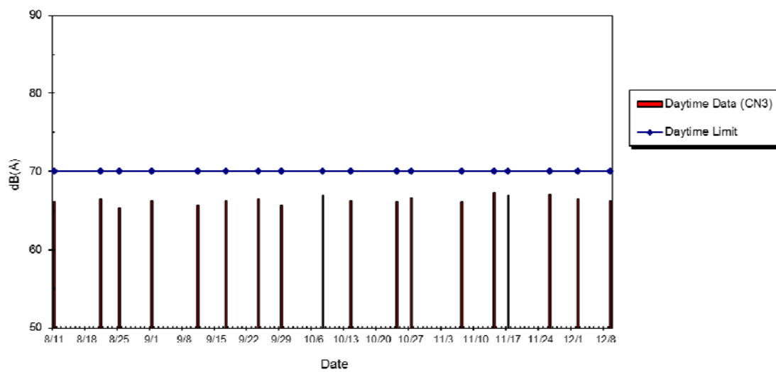
WIL-CN3 Noise Level at Lui Ming Choi Primary School, Aug 2014 - Dec 2014
