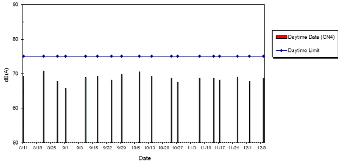
WIL-CN4 Noise Level at Luen Tak Apartments, Aug 2014 - Dec 2014
