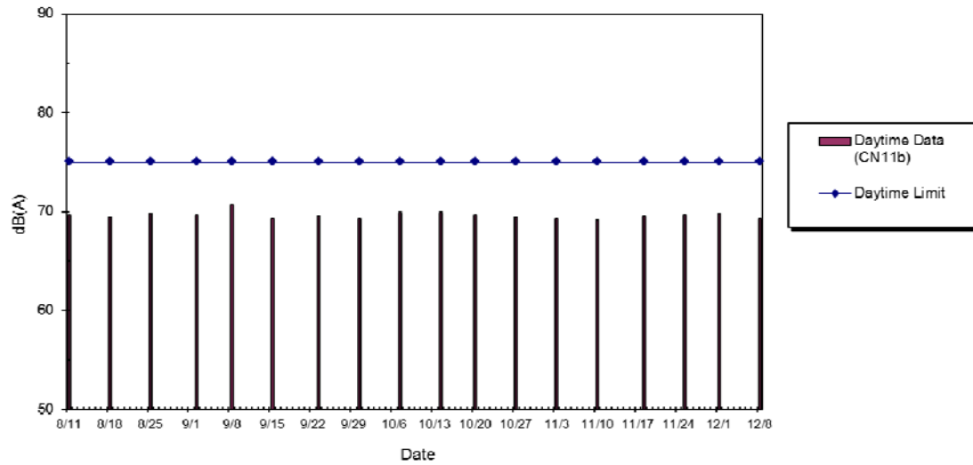
WIL-CN11b Noise Level at The Belcher's Tower 8, Aug 2014 - Dec 2014
