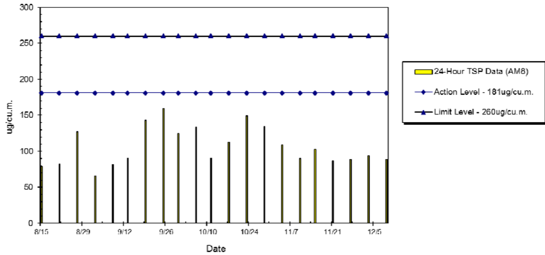
WIL-AM8 24hr TSP Level at Bon-Point (Aug 2014 - Dec 2014)
