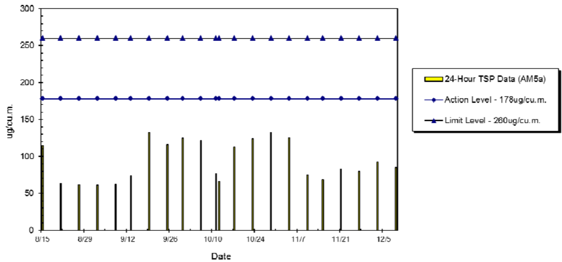
WIL-AM5a 24hr TSP Level at Kennedy Town Fire Station (Aug 2014 - Dec 2014)
