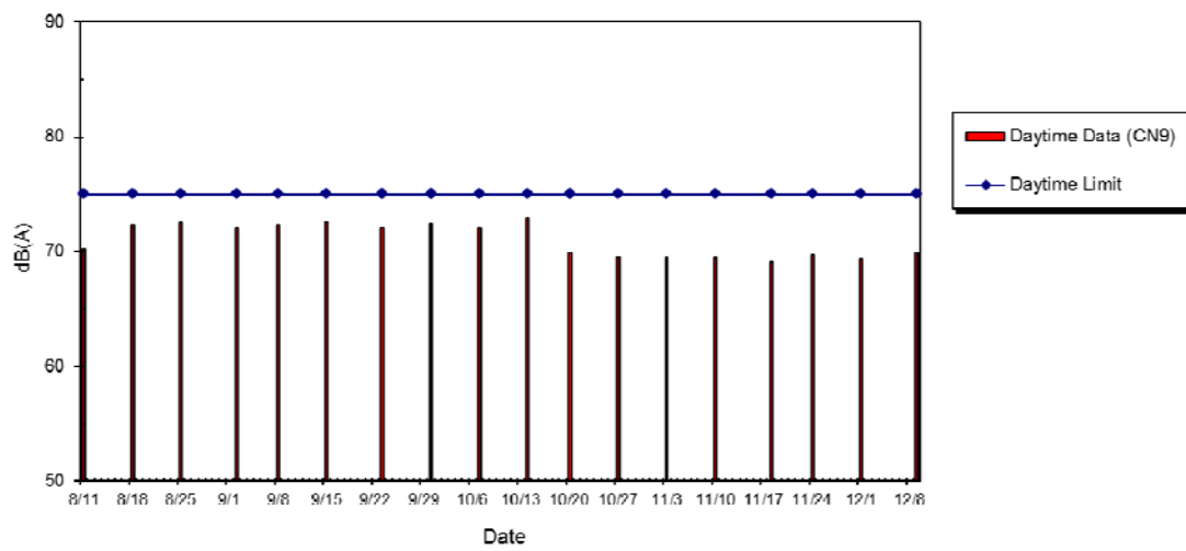
WIL-CN9 Noise Level at Hill Court, Aug 2014 - Dec 2014
