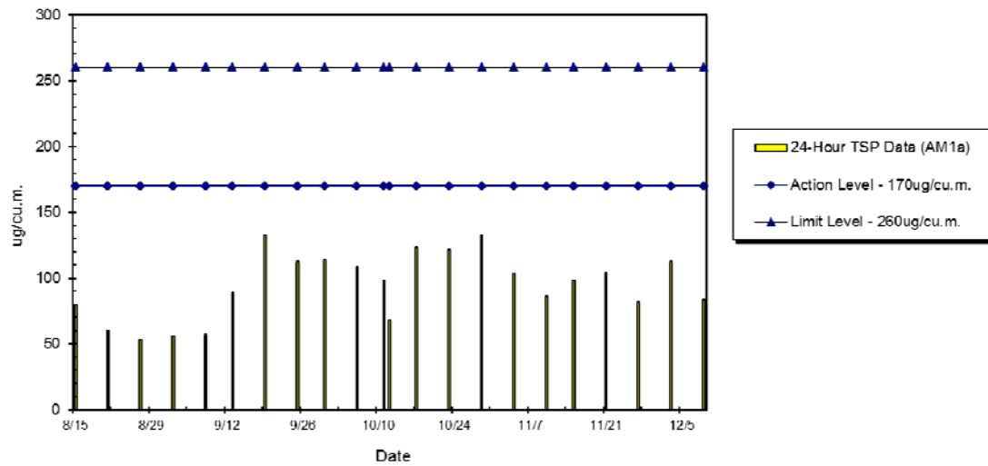
WIL-AM1a 24hr TSP Level at Kwun Lung Lau Block 1 (Aug 2014 - Dec 2014)
