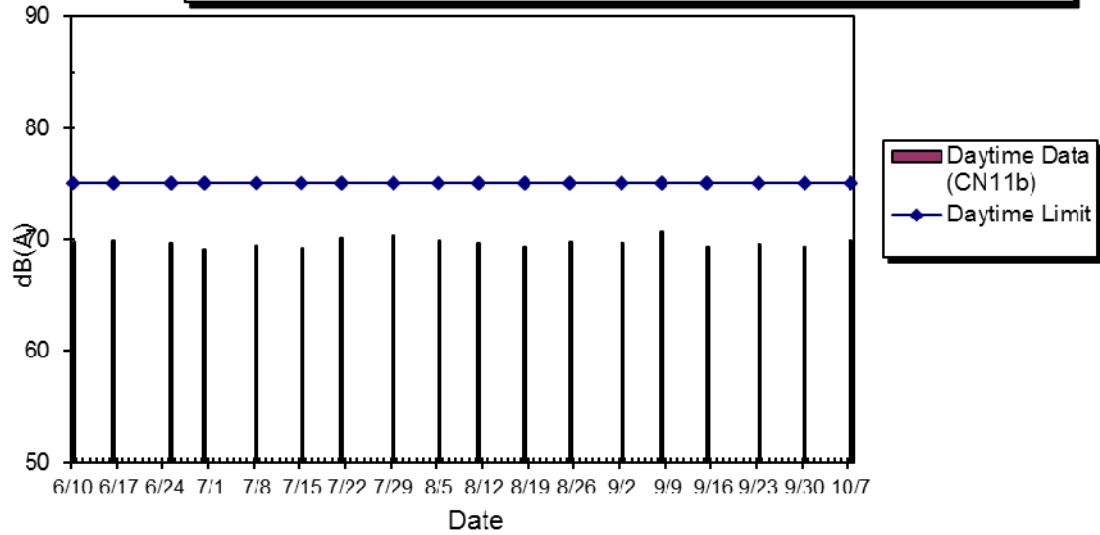
WIL-CN11b Noise Level at The Belcher's Tower 8, Jun 2014 - Oct 2014
