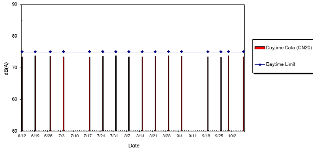
WIL-CN20 Noise Level at Ka On Building, Jun 2014 - Oct 2014
