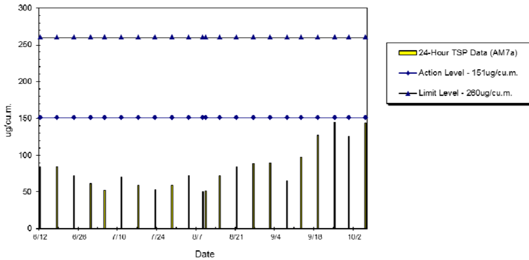
WIL-AM7a 24hr TSP Level at Hill Court (Jun 2014 - Oct 2014)
