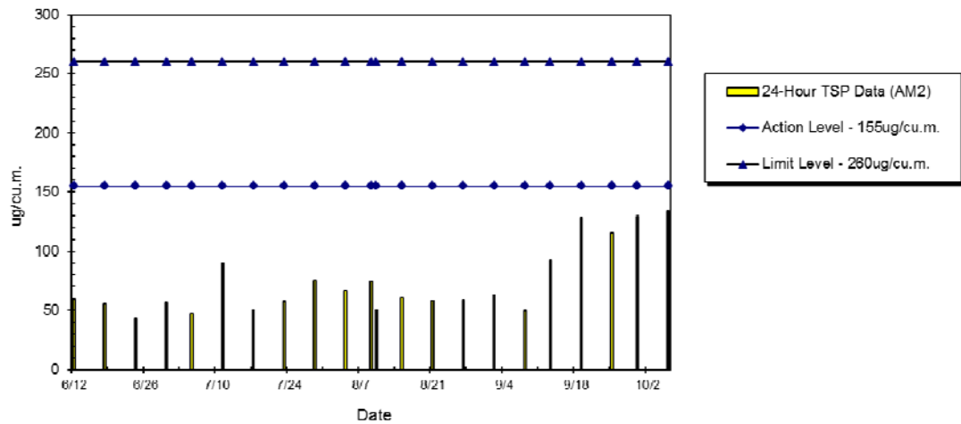
WIL-AM2 24hr TSP Level at Victoria Public Mortuary (Jun 2014 - Oct 2014)
