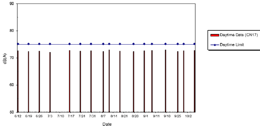
WIL-CN17 Noise Level at No.1 Third Street, Jun 2014 - Oct 2014
