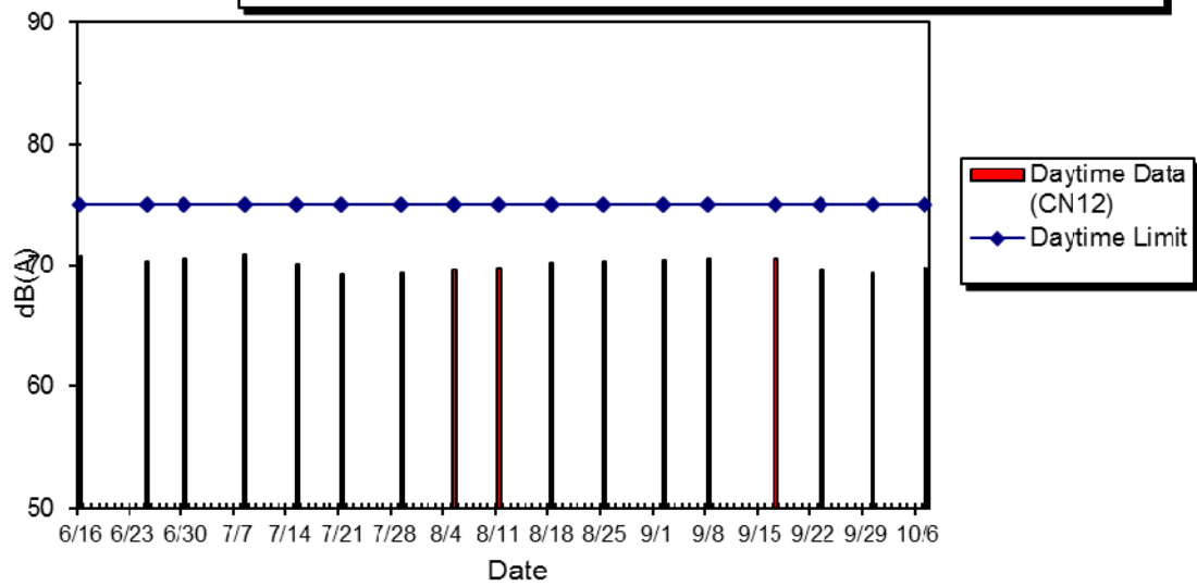
WIL-CN12 Noise Level at Wah Po Building, Jun 2014 - Oct 2014
