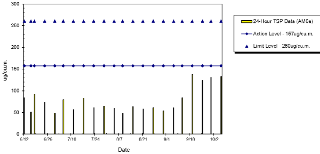
WIL-AM6a 24hr TSP Level at St. Paul's College Primary School (Jun 2014 - Oct 2014)
