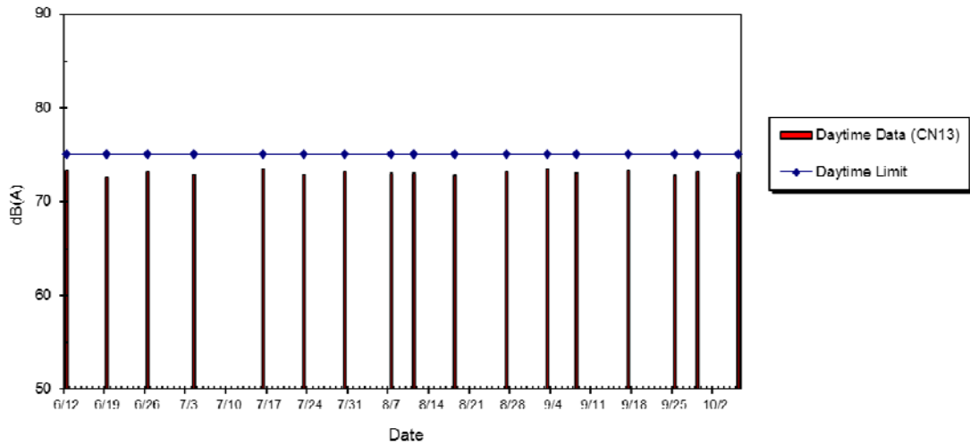
WIL-CN13 Noise Level at No.18-20 Eastern Street, Jun 2014 - Oct 2014
