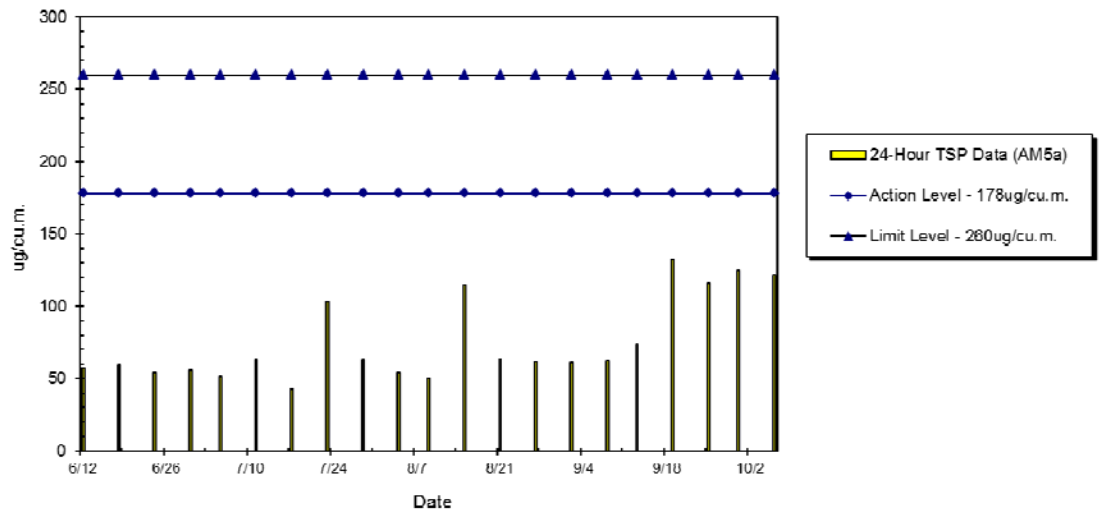
WIL-AM5a 24hr TSP Level at Kennedy Town Fire Station (Jun 2014 - Oct 2014)
