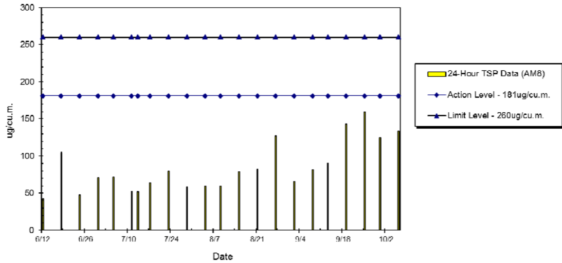
WIL-AM8 24hr TSP Level at Bon-Point (Jun 2014 - Oct 2014)
