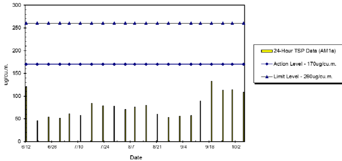
WIL-AM1a 24hr TSP Level at Kwun Lung Lau Block 1 (Jun 2014 - Oct 2014)
