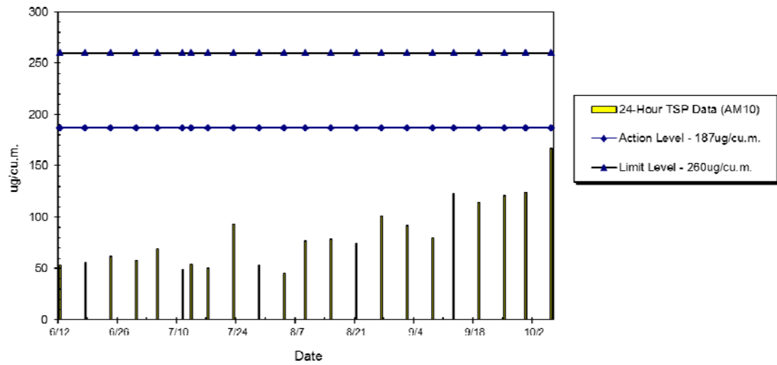
WIL-AM10 24hr TSP Level at Western Court, Ivy Tower (Jun 2014 - Oct 2014)
