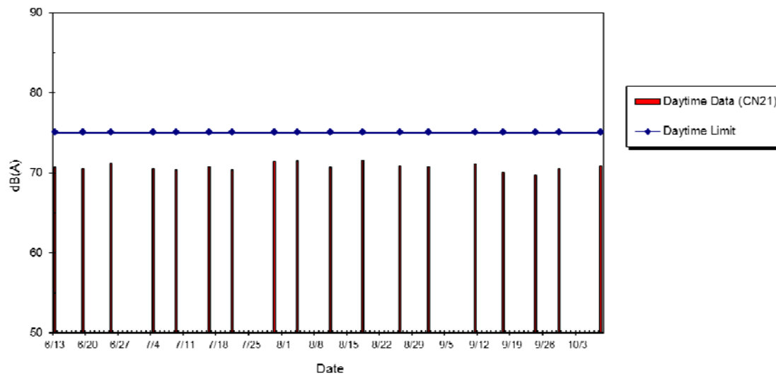
WIL-CN21 Noise Level at The Merton (Block 2), Jun 2014 - Oct 2014
