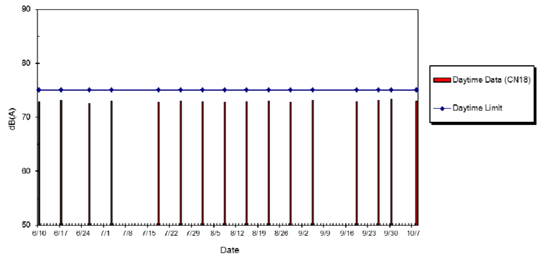
WIL-CN18 Noise Level at Princeton Tower, Jun 2014 - Oct 2014
