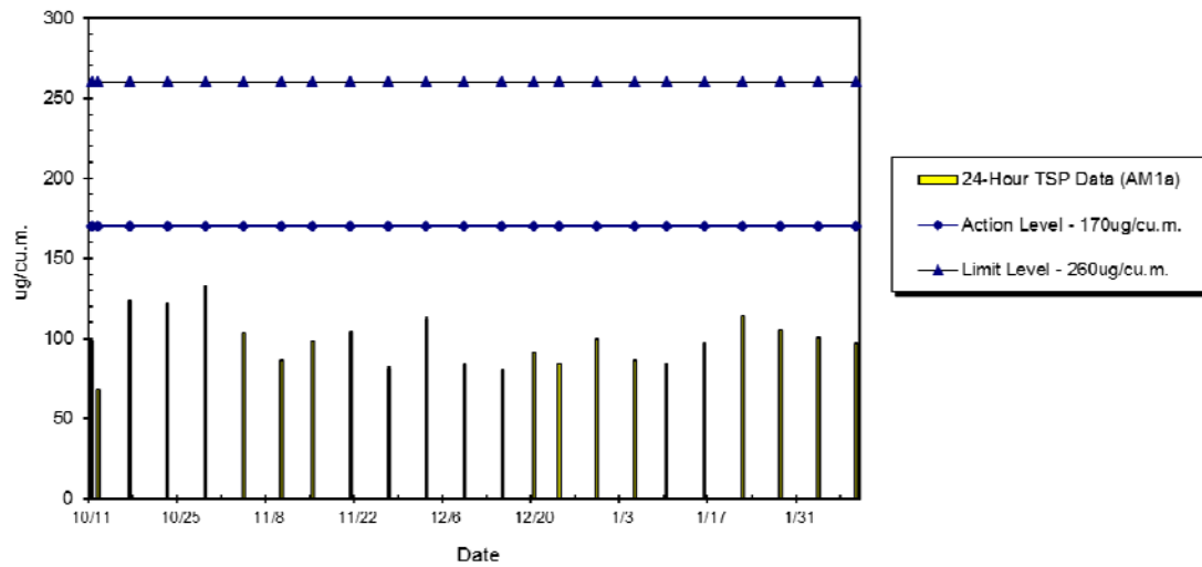
WIL-AM1a 24hr TSP Level at Kwun Lung Lau Block 1 (Oct 2014 - Feb 2015)
