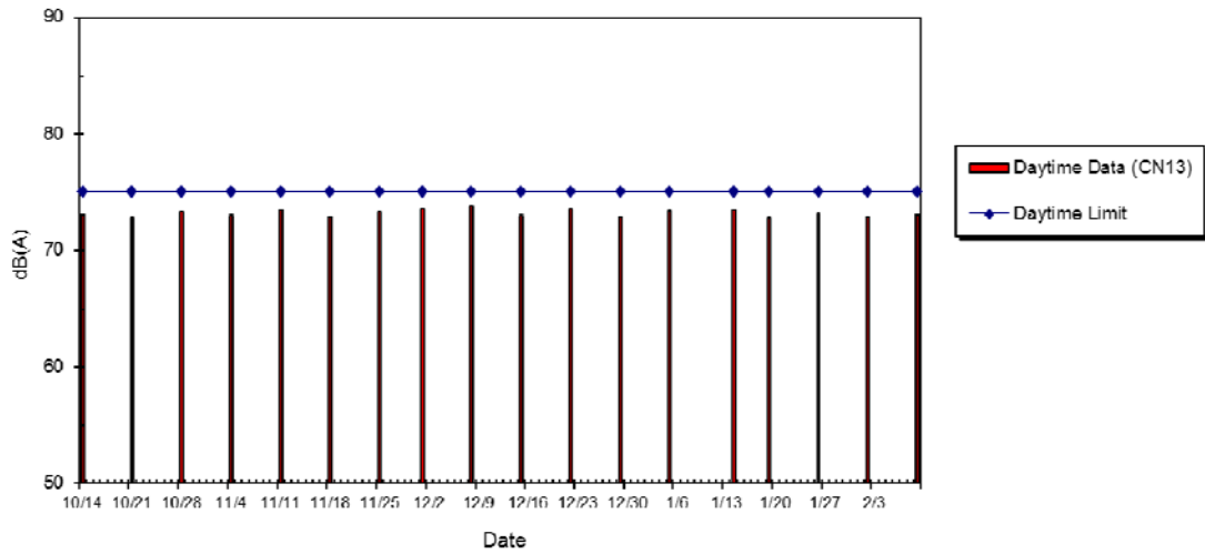
WIL-CN13 Noise Level at No.18-20 Eastern Street, Oct 2014 - Feb 2015
