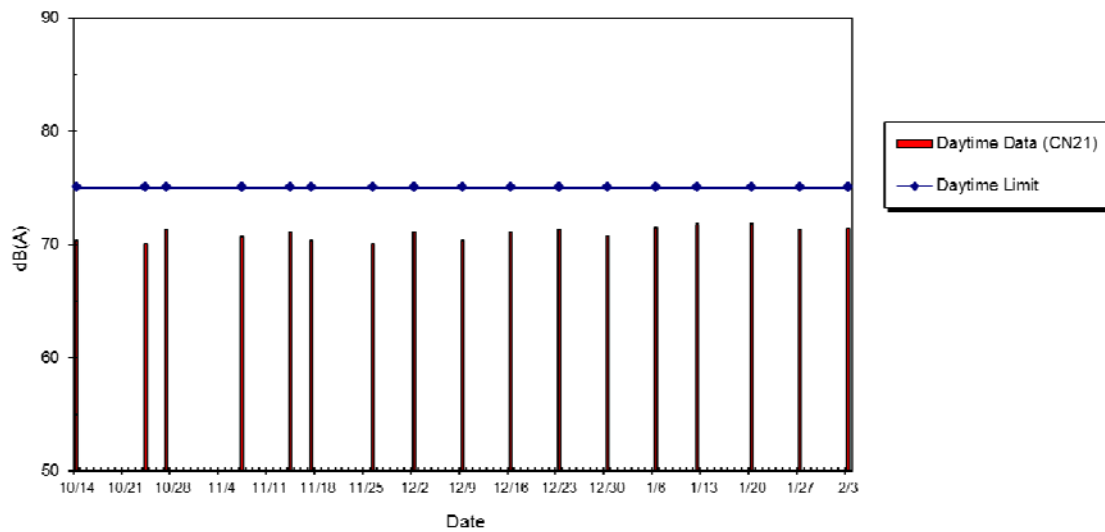
WIL-CN21 Noise Level at The Merton (Block 2), Oct 2014 - Feb 2015
