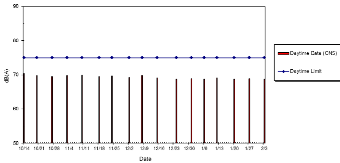
WIL-CN5 Noise Level at Western Court, Oct 2014 - Feb 2015
