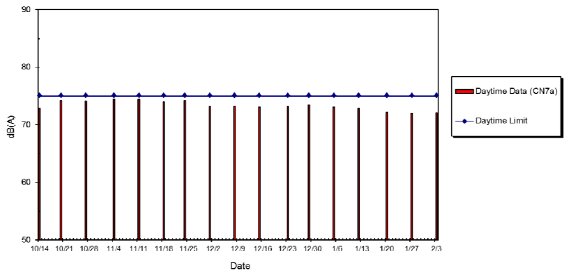
WIL-CN7a Noise Level at Bowie Court, Oct 2014 - Feb 2015
