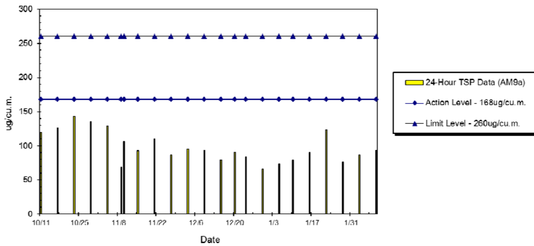
WIL-AM9a 24hr TSP Level at No. 28 Sai Woo Lane (Oct 2014 - Feb 2015)
