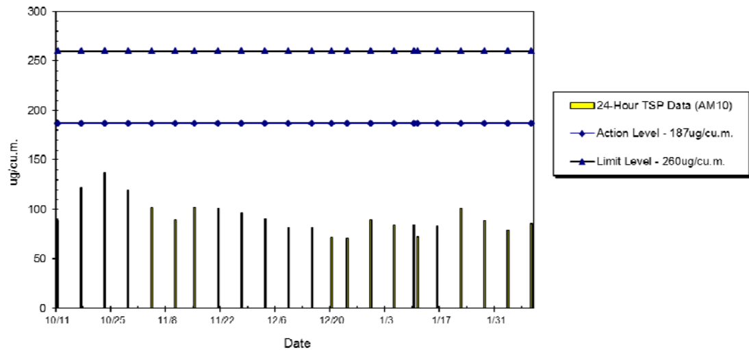
WIL-AM10 24hr TSP Level at Western Court, Ivy Tower (Oct 2014 - Feb 2015)
