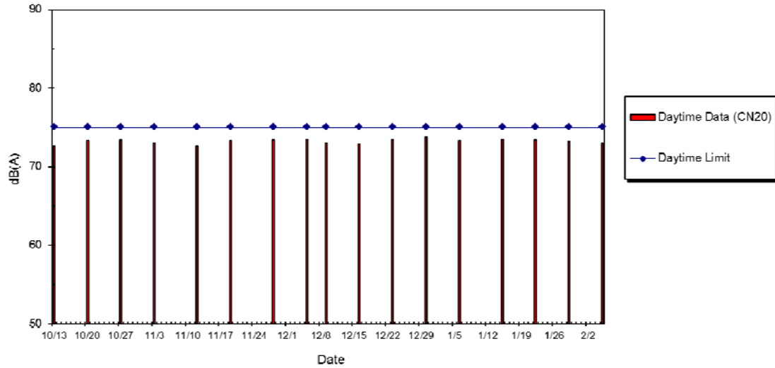
WIL-CN20 Noise Level at Ka On Building, Oct 2014 - Feb 2015
