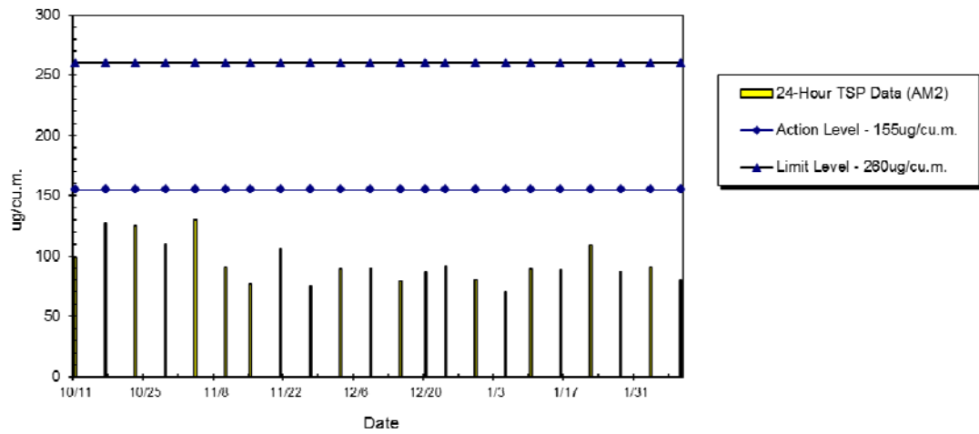
WIL-AM2 24hr TSP Level at Victoria Public Mortuary (Oct 2014 - Feb 2015)
