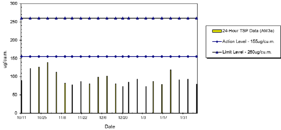
WIL-AM3a 24hr TSP Level at HK IVE (Tsing Yi) Kennedy Town Centre (Oct 2014 - Feb 2015)
