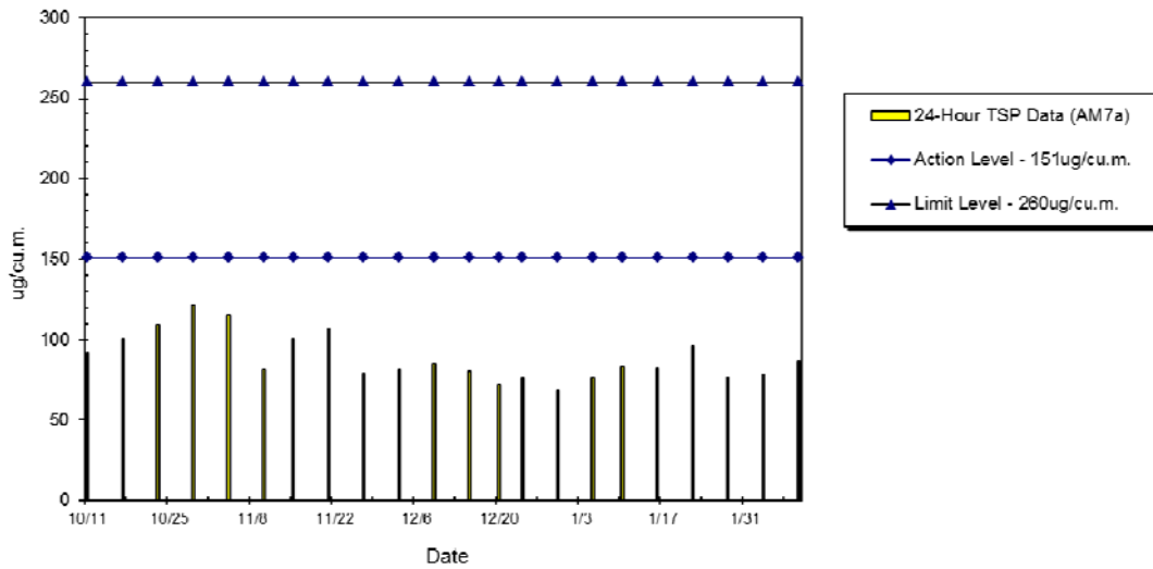
WIL-AM7a 24hr TSP Level at Hill Court (Oct 2014 - Feb 2015)
