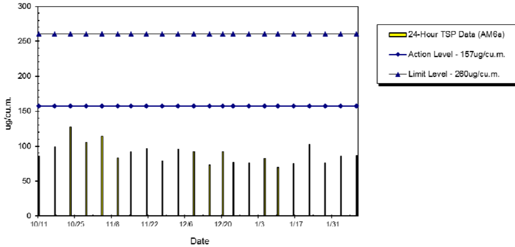
WIL-AM6a 24hr TSP Level at St. Paul's College Primary School (Oct 2014 - Feb 2015)
