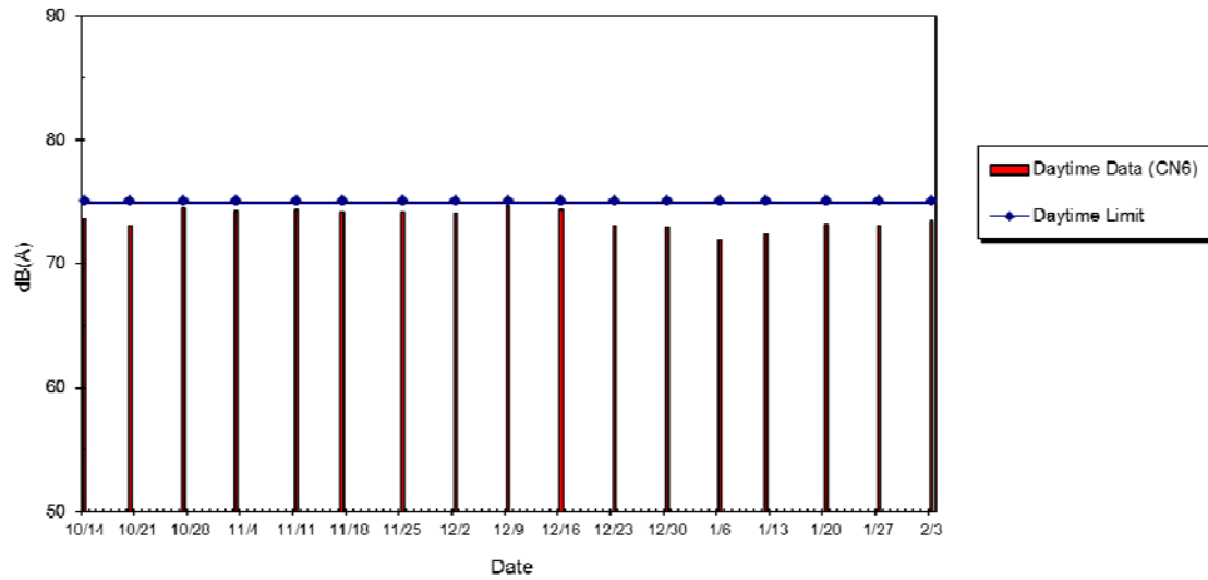
WIL-CN6 Noise Level at Yick Fung Garden (Block A), Oct 2014 - Feb 2015
