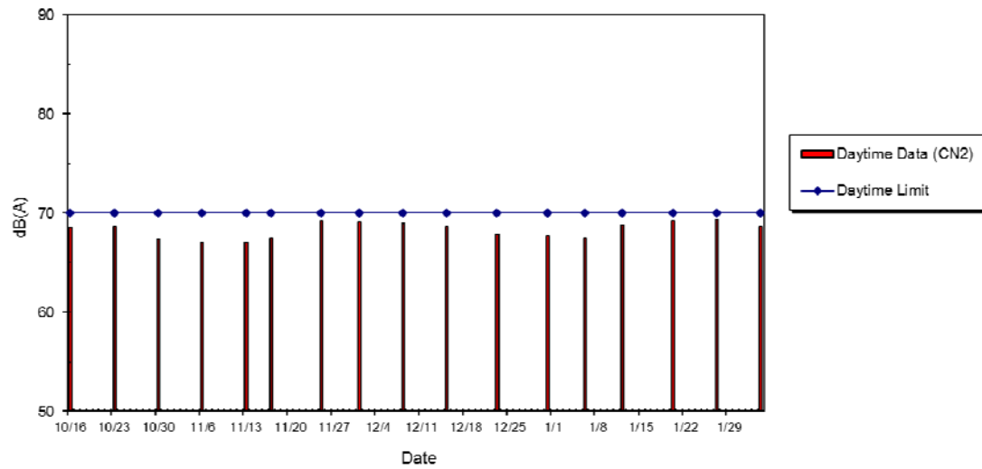
WIL-CN2 Noise Level at HK IVE (Tsing Yi) Kennedy Town Centre, Oct 2014 - Feb 2015
