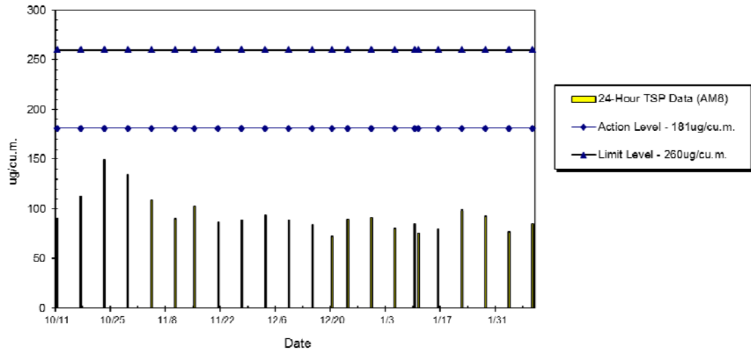
WIL-AM8 24hr TSP Level at Bon-Point (Oct 2014 - Feb 2015)
