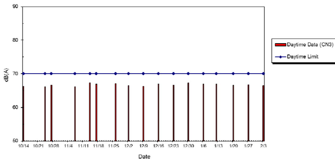
WIL-CN3 Noise Level at Lui Ming Choi Primary School, Oct 2014 - Feb 2015
