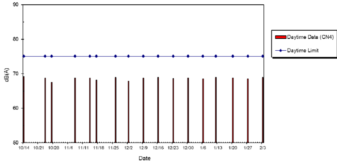
WIL-CN4 Noise Level at Luen Tak Apartments, Oct 2014 - Feb 2015
