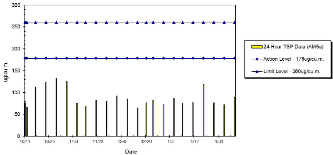
WIL-AM5a 24hr TSP Level at Kennedy Town Fire Station (Oct 2014 - Feb 2015)
