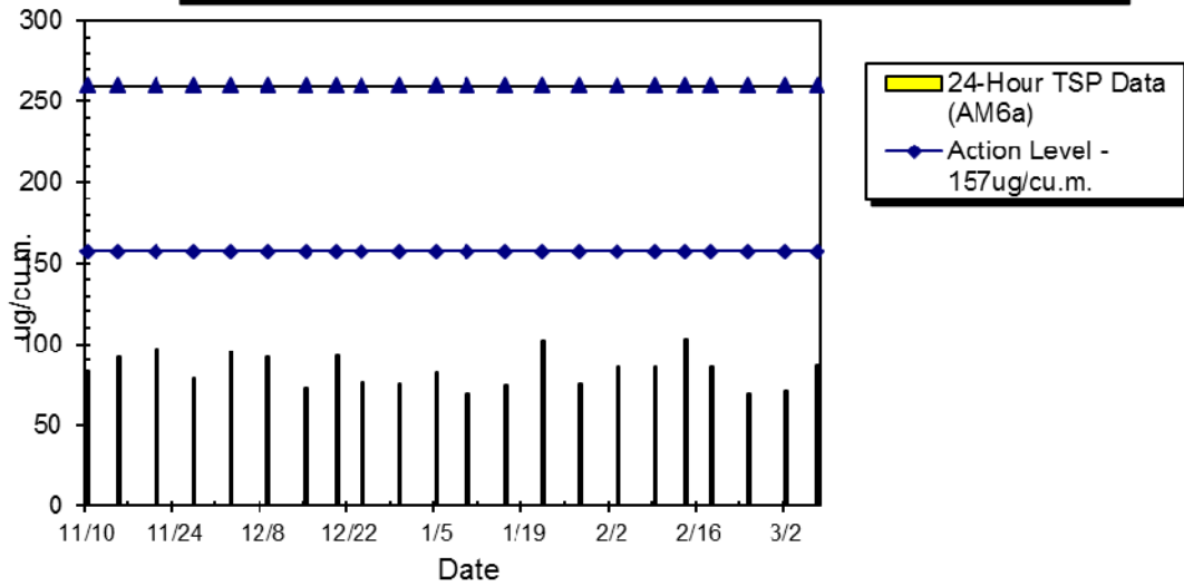
WIL-AM6a 24hr TSP Level at St. Paul's College Primary School (Nov 2014 - Mar 2015)
