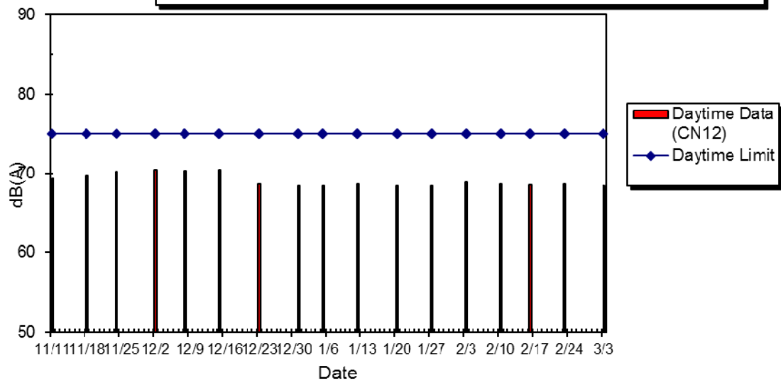
WIL-CN12 Noise Level at Wah Po Building, Nov 2014 - Mar 2015
