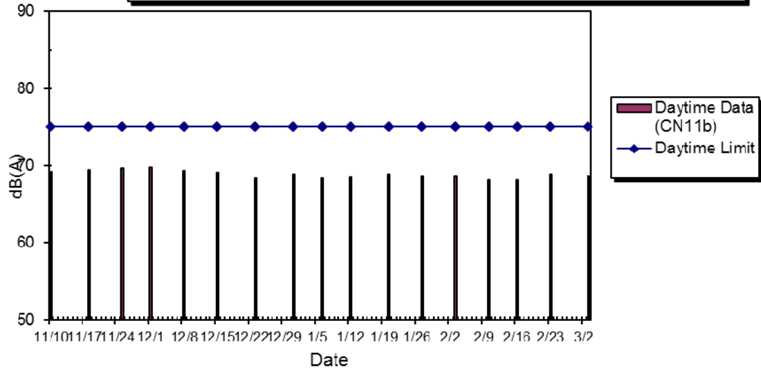
WIL-CN11b Noise Level at The Belcher's Tower 8, Nov 2014 - Mar 2015
