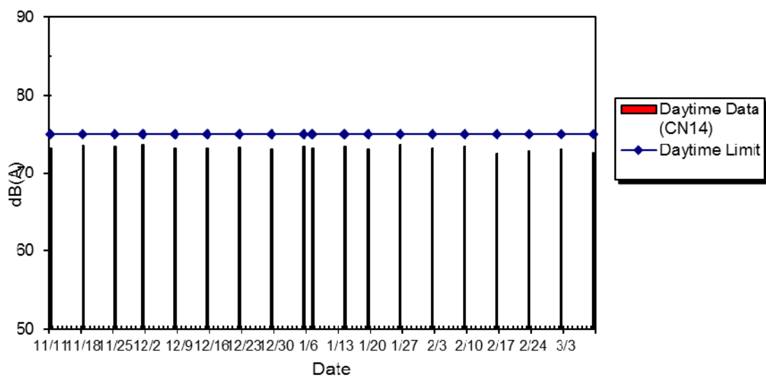
WIL-CN14 Noise Level at Bon-Point, Nov 2014 - Mar 2015
