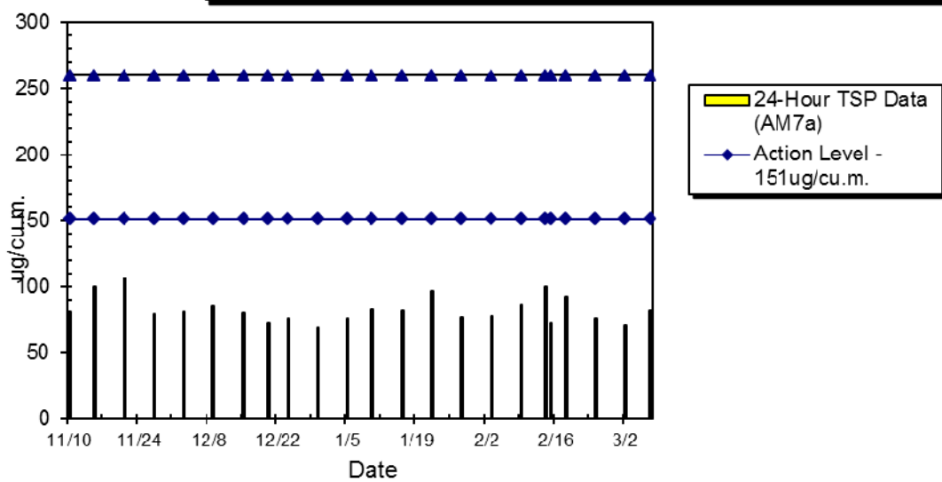
WIL-AM7a 24hr TSP Level at Hill Court (Nov 2014 - Mar 2015)
