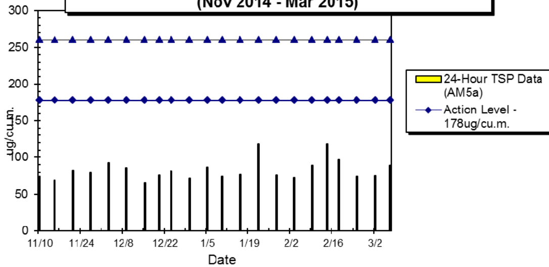
WIL-AM5a 24hr TSP Level at Kennedy Town Fire Station (Nov 2014 - Mar 2015)
