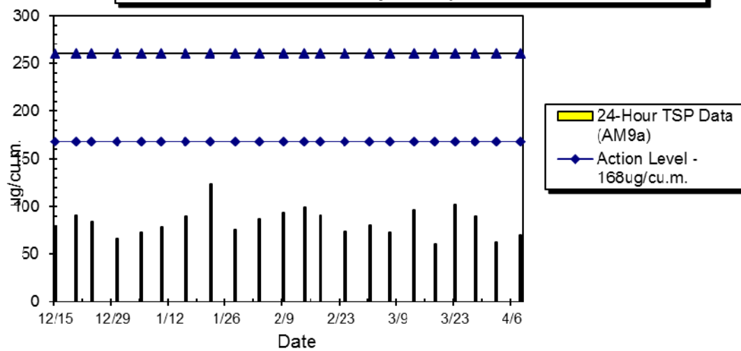
WIL-AM9a 24hr TSP Level at No. 28 Sai Woo Lane (Dec 2014 - Apr 2015)
