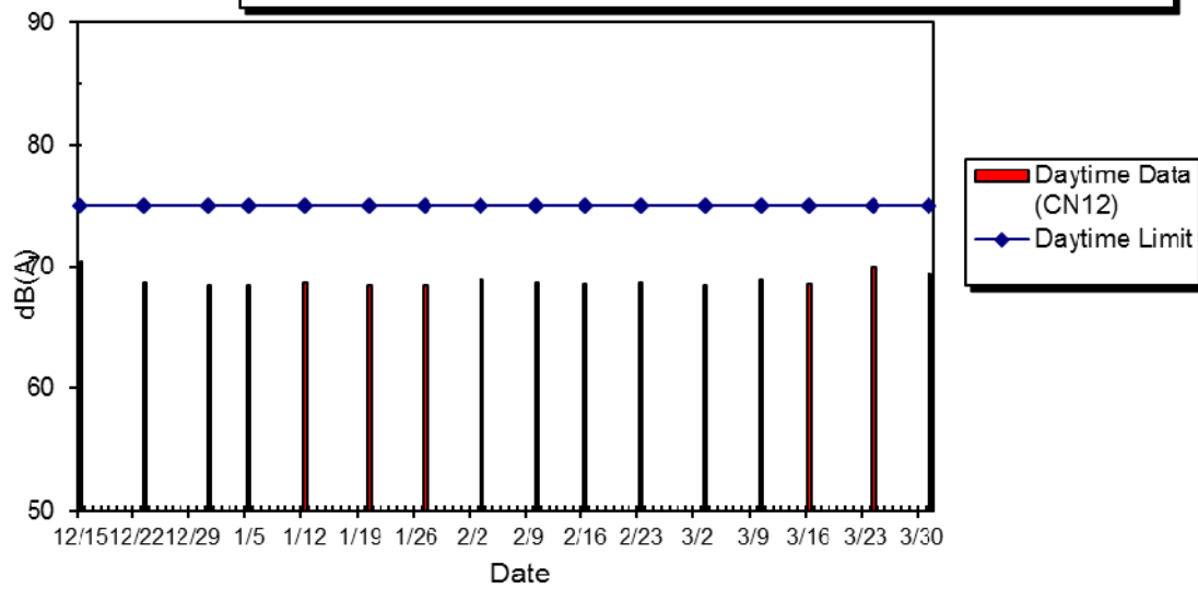
WIL-CN12 Noise Level at Wah Po Building, Dec 2014 - Apr 2015
