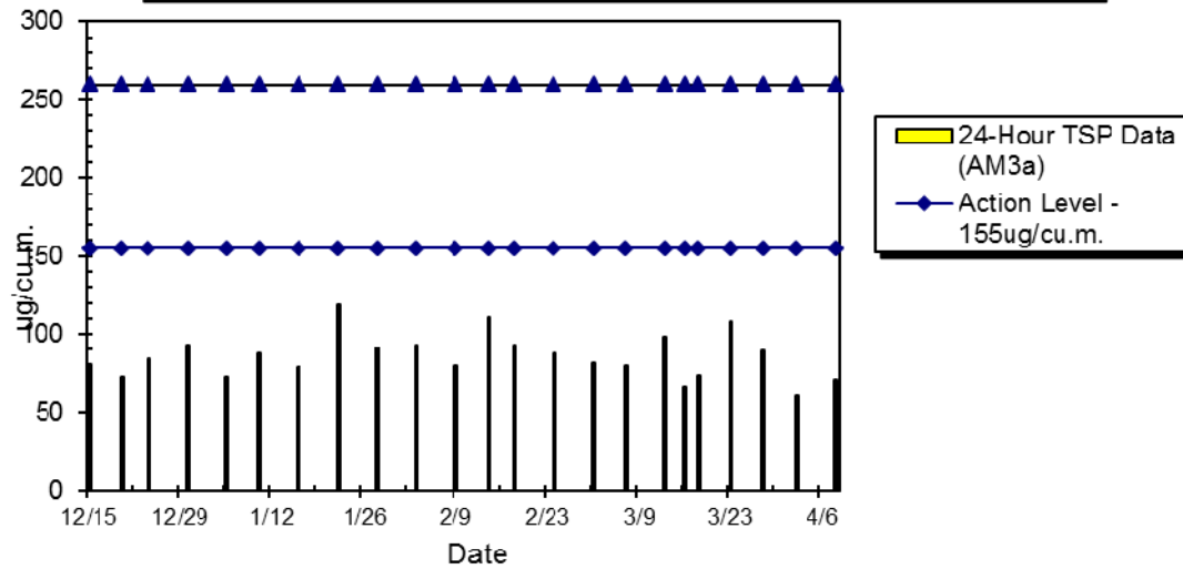
WIL-AM3a 24hr TSP Level at HK IVE (Tsing Yi) Kennedy Town Centre (Dec 2014 - Apr 2015)
