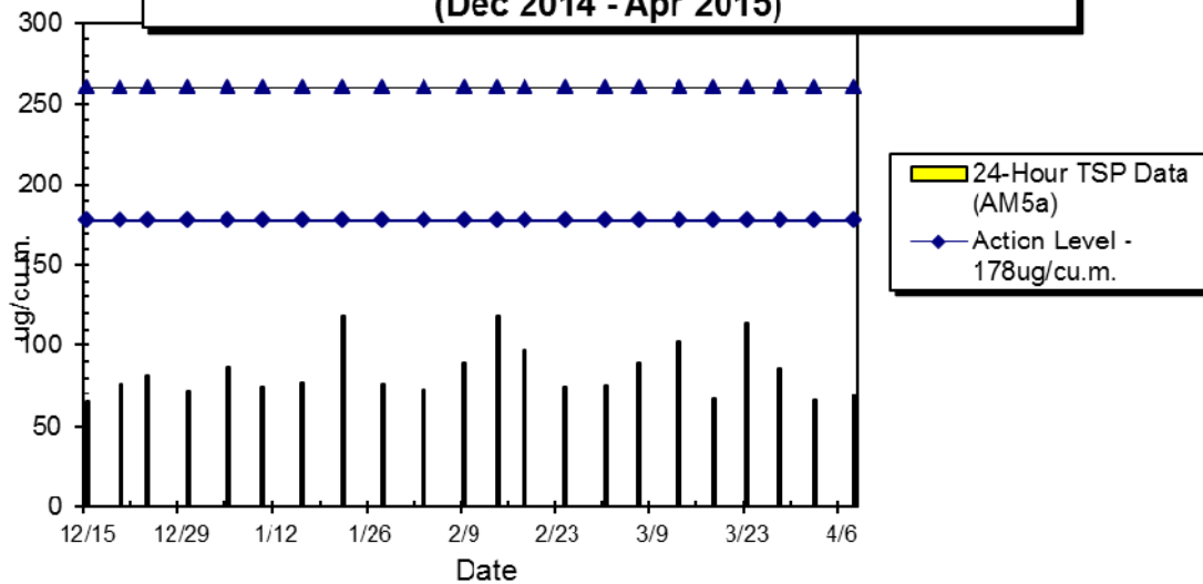
WIL-AM5a 24hr TSP Level at Kennedy Town Fire Station (Dec 2014 - Apr 2015)
