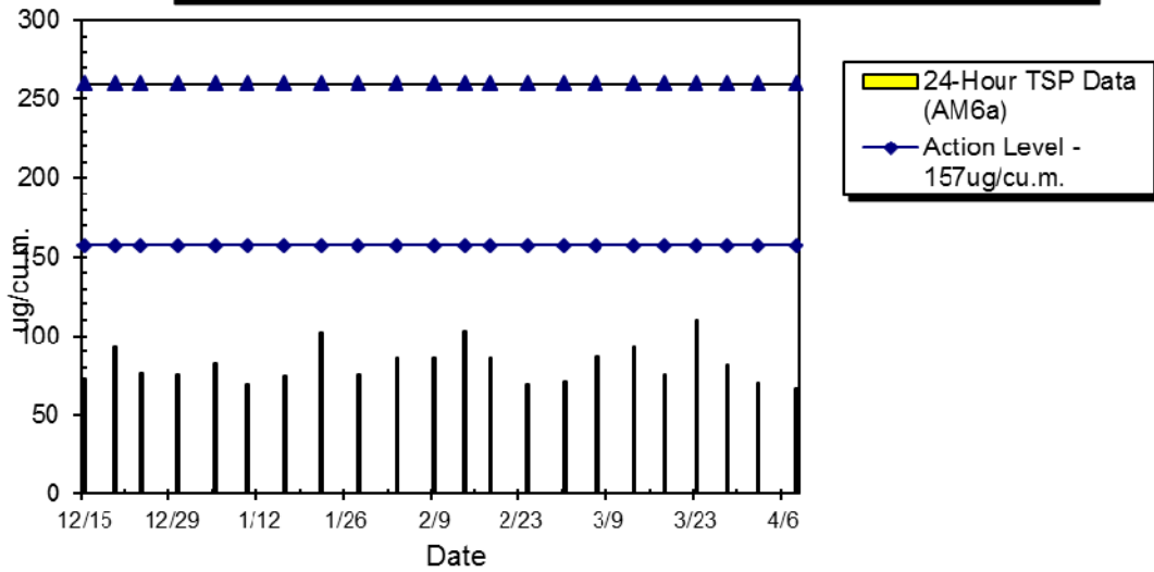
WIL-AM6a 24hr TSP Level at St. Paul's College Primary School (Dec 2014 - Apr 2015)
