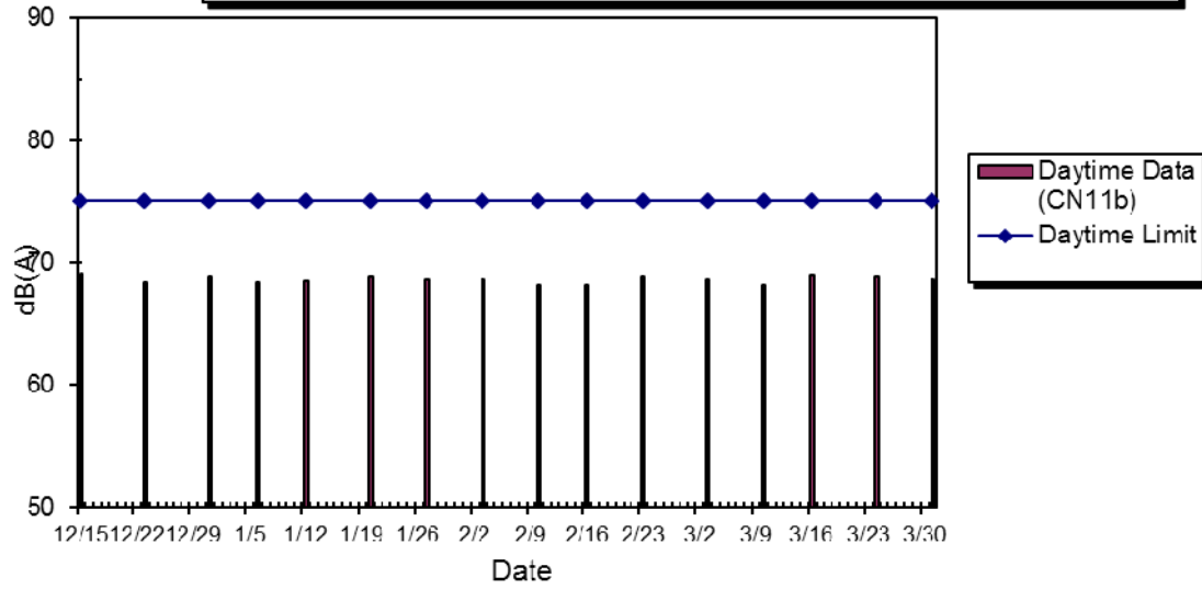
WIL-CN11b Noise Level at The Belcher's Tower 8, Dec 2014 - Apr 2015
