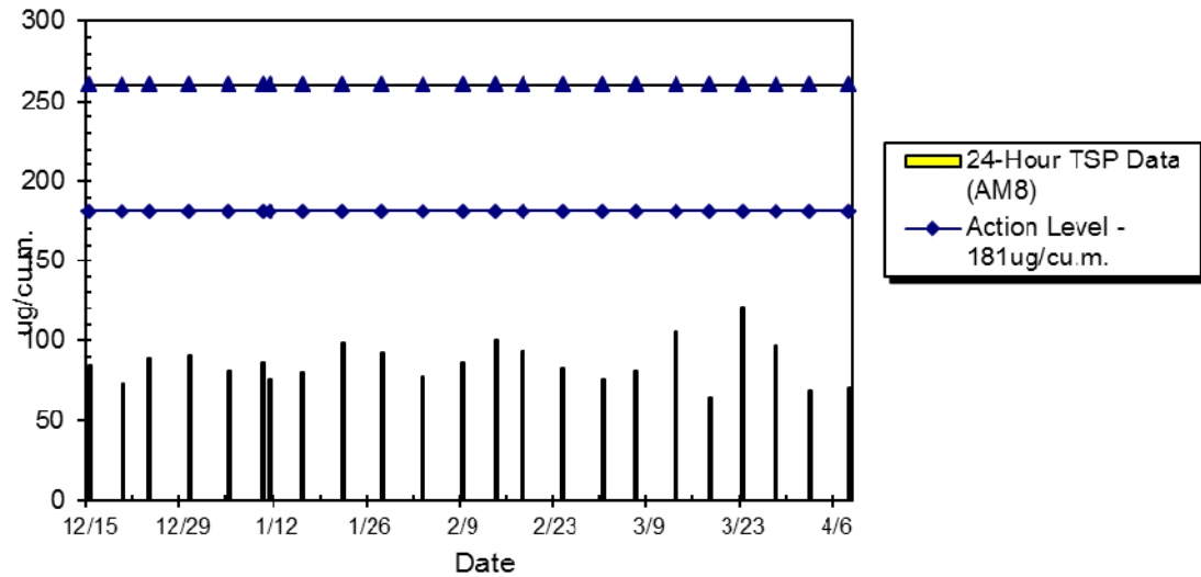
WIL-AM8 24hr TSP Level at Bon-Point (Dec 2014 - Apr 2015)
