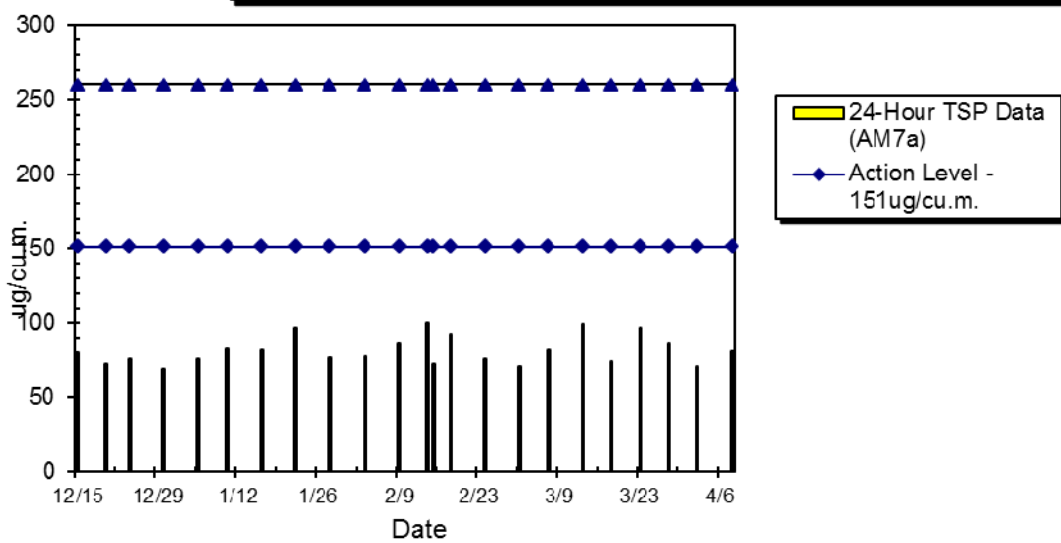
WIL-AM7a 24hr TSP Level at Hill Court (Dec 2014 - Apr 2015)
