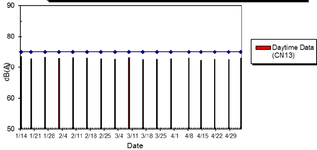
WIL-CN13 Noise Level at No.18-20 Eastern Street, Jan 2015 - May 2015
