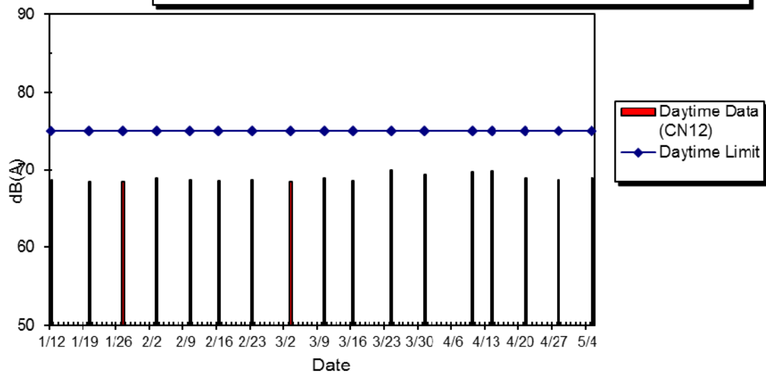
WIL-CN12 Noise Level at Wah Po Building, Jan 2015 - May 2015
