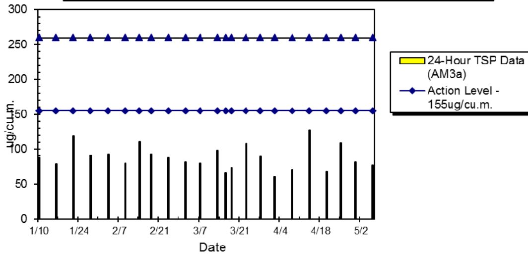
WIL-AM3a 24hr TSP Level at HK IVE (Tsing Yi) Kennedy Town Centre (Jan 2015 - May 2015)
