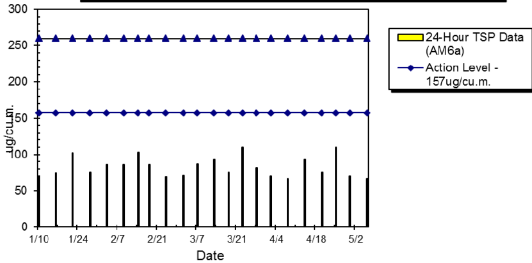
WIL-AM6a 24hr TSP Level at St. Paul's College Primary School (Jan 2015 - May 2015)
