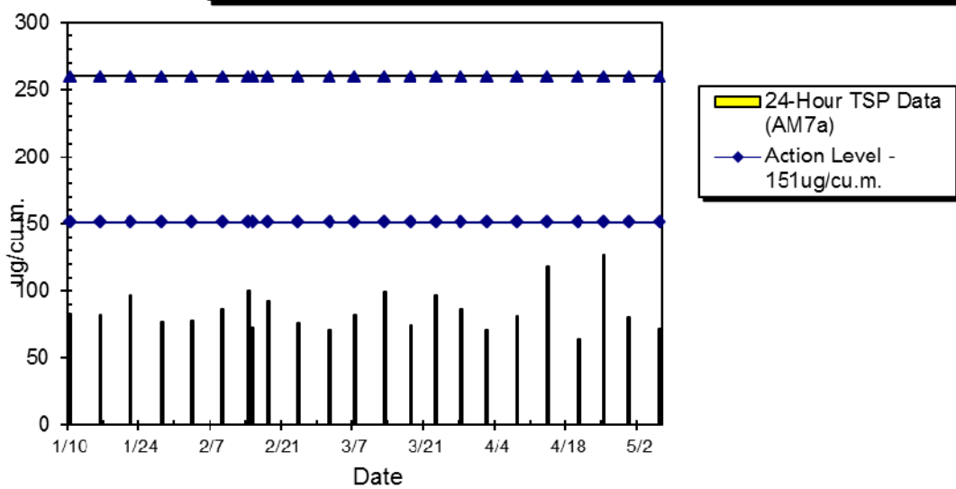
WIL-AM7a 24hr TSP Level at Hill Court (Jan 2015 - May 2015)
