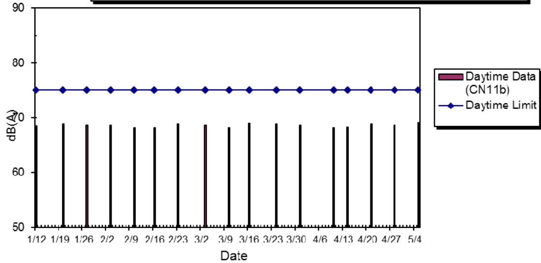
WIL-CN11b Noise Level at The Belcher's Tower 8, Jan 2015 - May 2015
