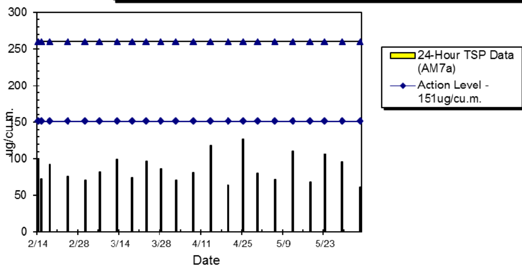
WIL-AM7a 24hr TSP Level at Hill Court (Feb 2015 - Jun 2015)
