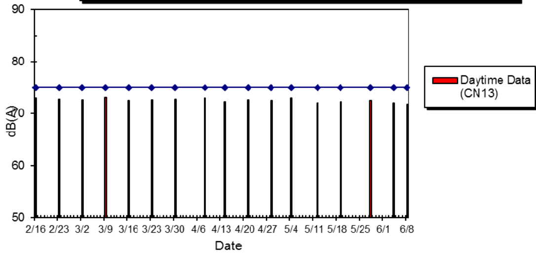
WIL-CN13 Noise Level at No.18-20 Eastern Street, Feb 2015 - Jun 2015
