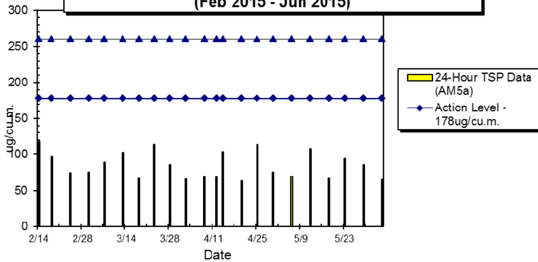
WIL-AM5a 24hr TSP Level at Kennedy Town Fire Station (Feb 2015 - Jun 2015)
