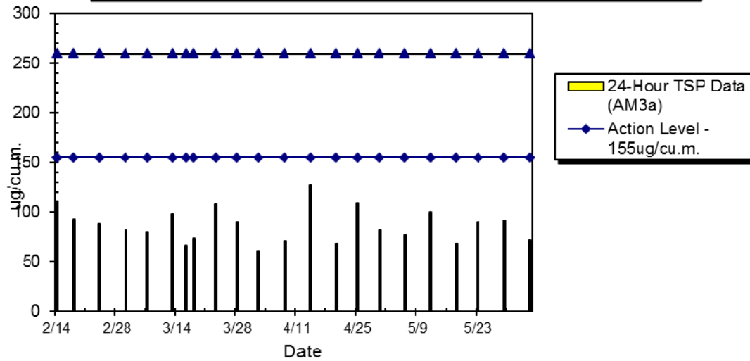
WIL-AM3a 24hr TSP Level at HK IVE (Tsing Yi) Kennedy Town Centre (Feb 2015 - Jun 2015)
