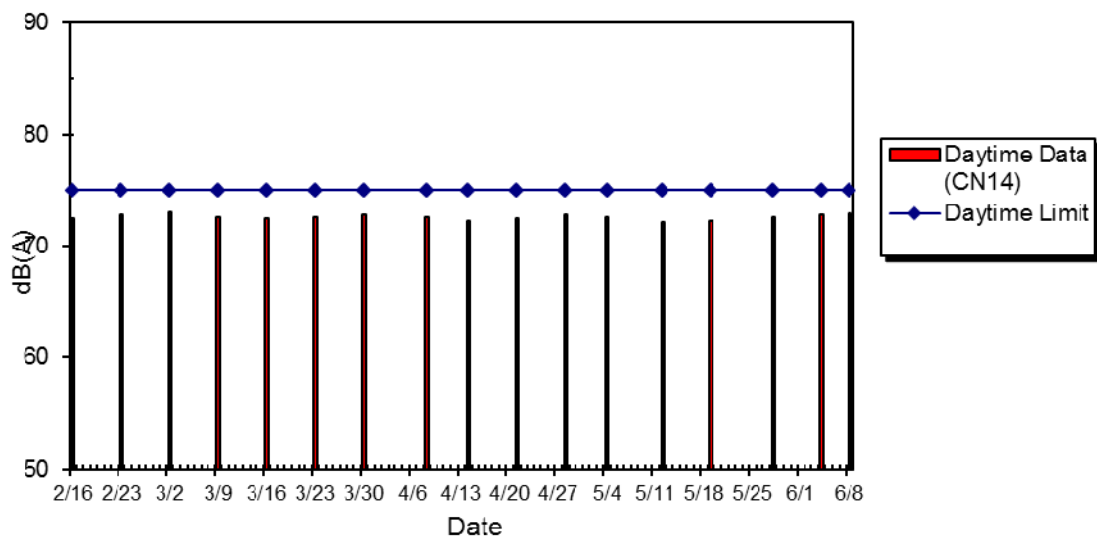
WIL-CN14 Noise Level at Bon-Point, Feb 2015 - Jun 2015
