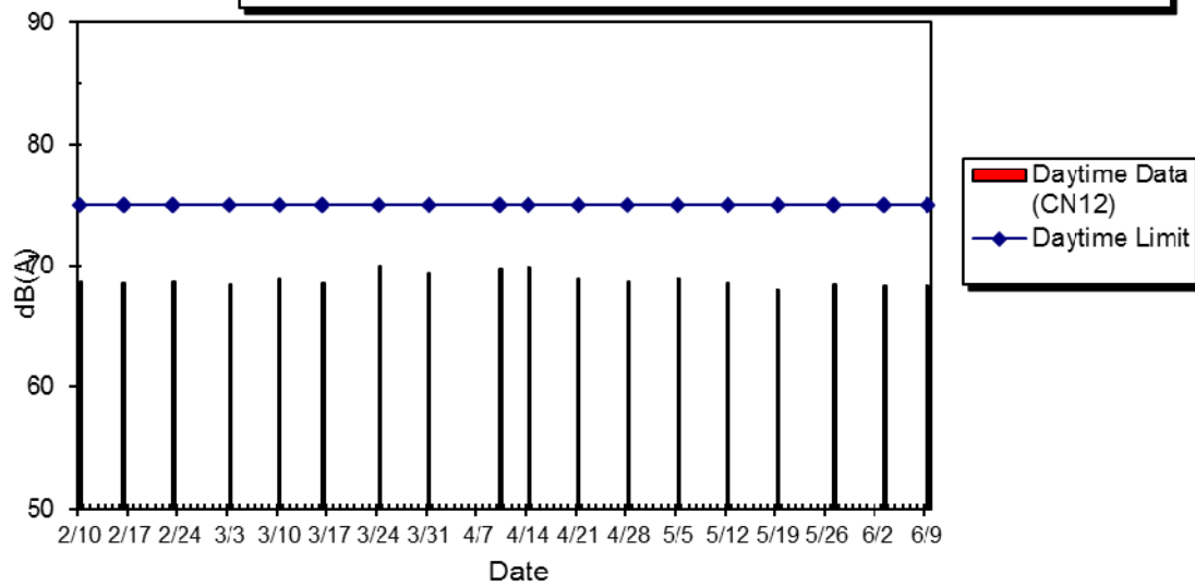
WIL-CN12 Noise Level at Wah Po Building, Feb 2015 - Jun 2015
