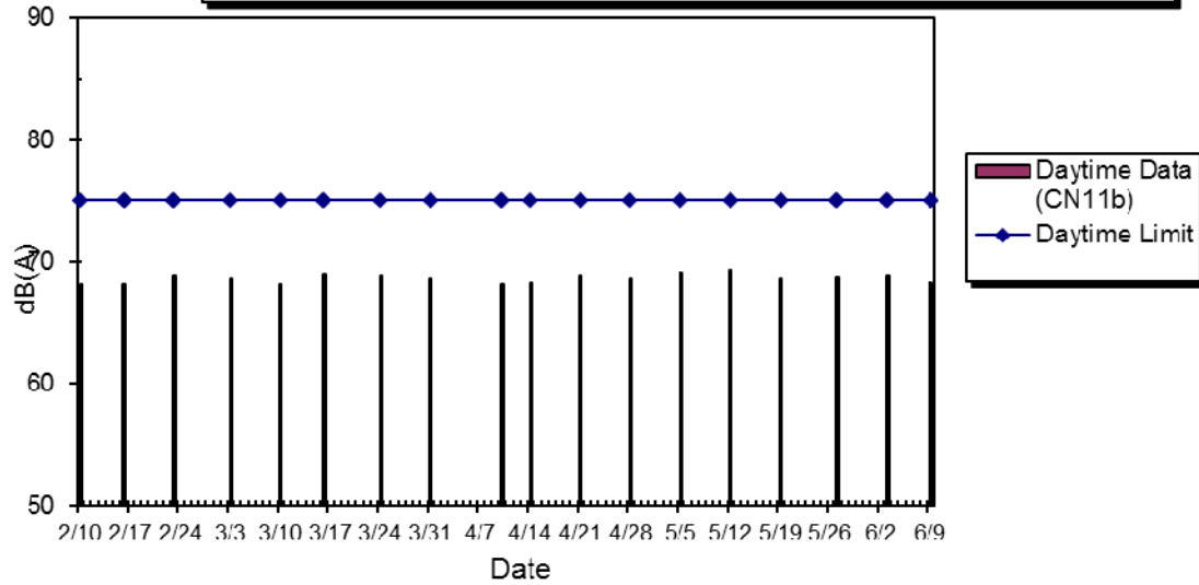
WIL-CN11b Noise Level at The Belcher's Tower 8, Feb 2015 - Jun 2015
