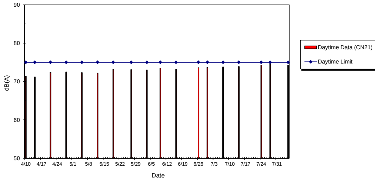
WIL-CN21 Noise Level at The Merton (Block 2), Apr 2015 - Aug 2015
