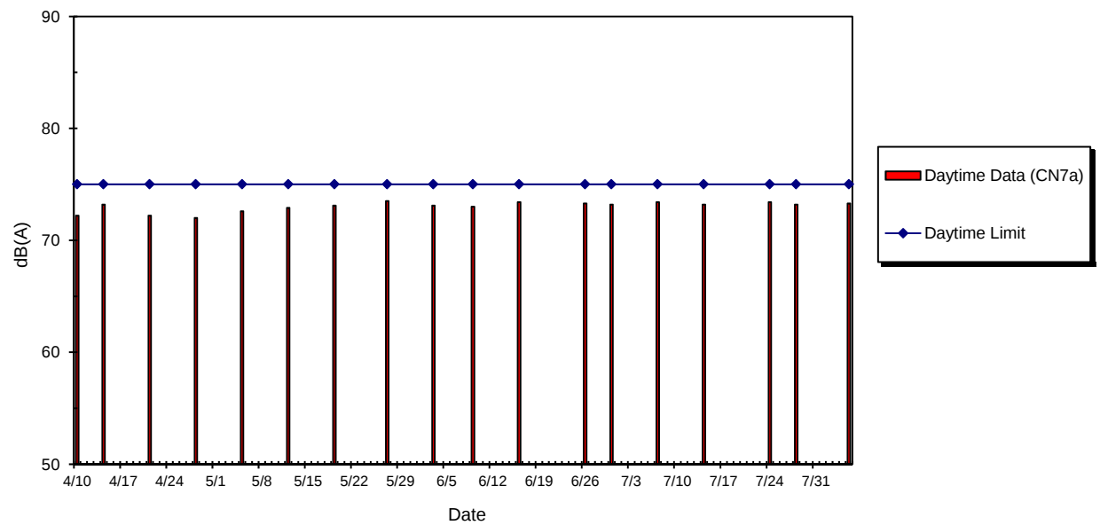
WIL-CN7a Noise Level at Bowie Court, Apr 2015 - Aug 2015
