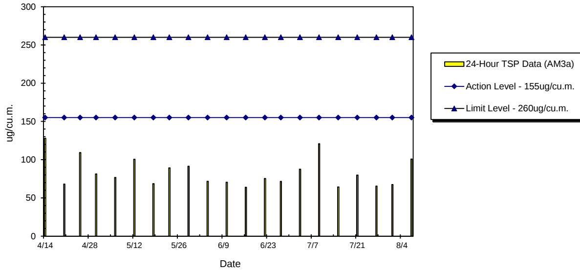
WIL-AM3a 24hr TSP Level at HK IVE (Tsing Yi) Kennedy Town Centre (Apr 2015 - Aug 2015)
