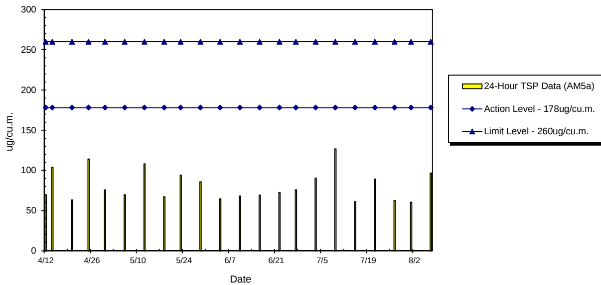
WIL-AM5a 24hr TSP Level at Kennedy Town Fire Station (Apr 2015 - Aug 2015)
