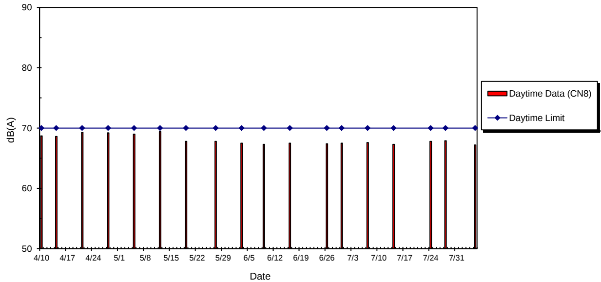
WIL-CN8 Noise Level at St. Paul's College Primary School, Apr 2015 - Aug 2015
