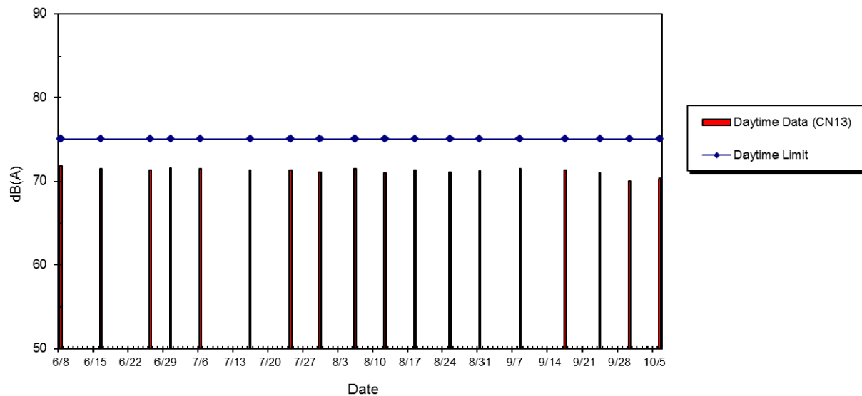
WIL-CN13 Noise Level at No.18-20 Eastern Street, Jun 2015 - Oct 2015
