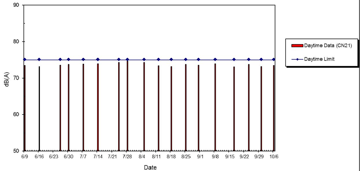
WIL-CN21 Noise Level at The Merton (Block 2), Jun 2015 - Oct 2015
