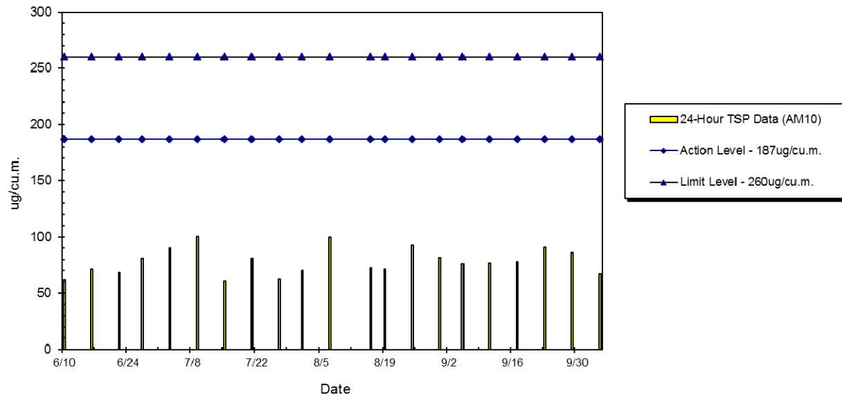
WIL-AM10 24hr TSP Level at Western Court, Ivy Tower (Jun 2015 - Oct 2015)
