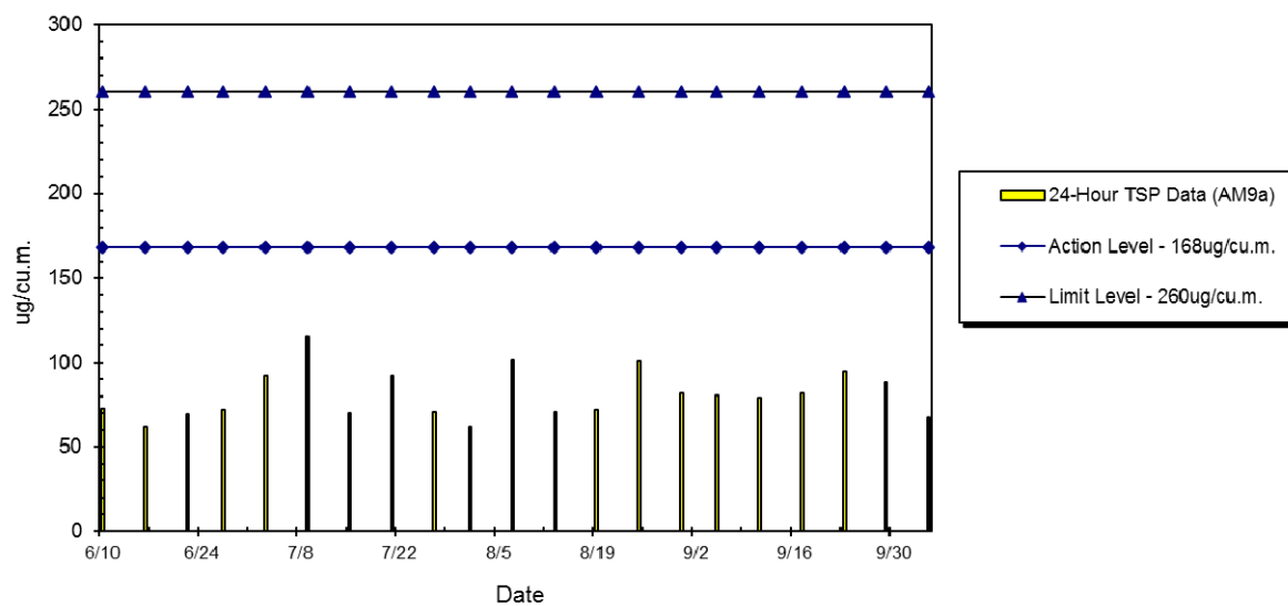
WIL-AM9a 24hr TSP Level at No. 28 Sai Woo Lane (Jun 2015 - Oct 2015)
