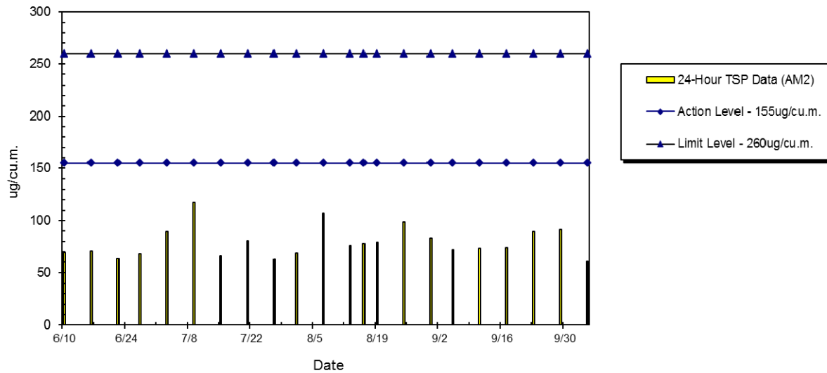
WIL-AM2 24hr TSP Level at Victoria Public Mortuary (Jun 2015 - Oct 2015)
