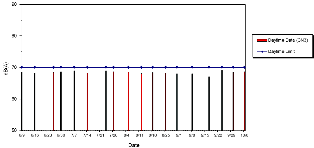
WIL-CN3 Noise Level at Lui Ming Choi Primary School, Jun 2015 - Oct 2015
