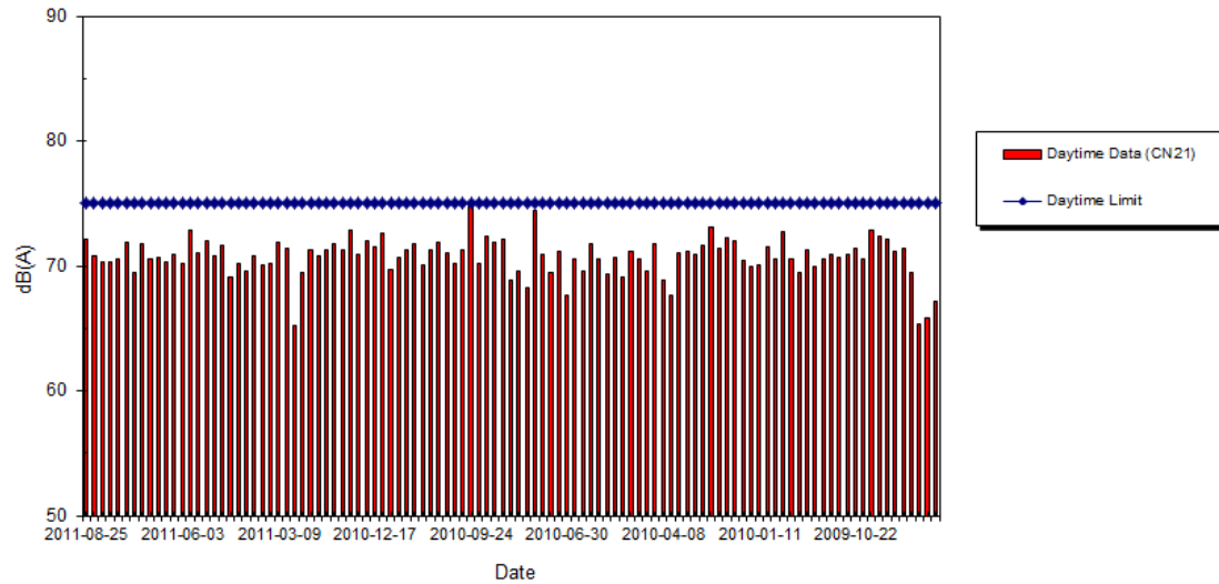
WIL-CN21 Noise Level at The Merton (Block 2), Aug 2009 - Aug 2011
