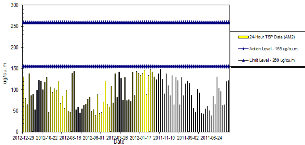
WIL-AM2 24hr TSP Level at Victoria Public Mortuary (May 2011 - Dec 2012)
