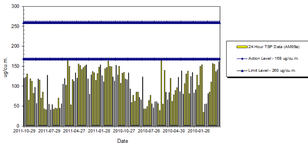
WIL-AM9a 24hr TSP Level at No. 28 Sai Woo Lane (Nov 2009 - Oct 2011)
