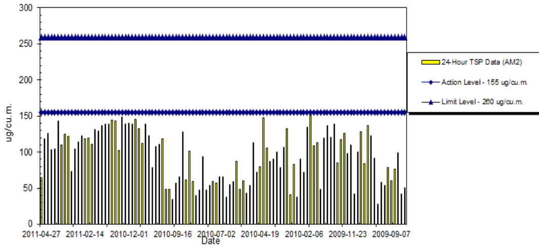
WIL-AM2 24hr TSP Level at Victoria Public Mortuary (Aug 2009 - Apr 2011)
