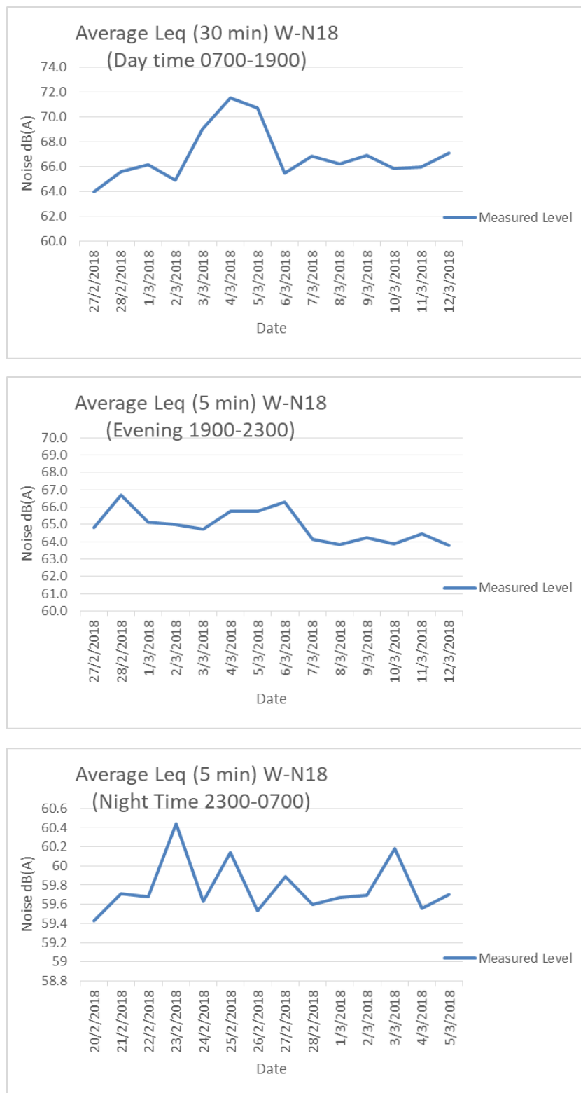
Figure F.2 Measured Noise Level for Hydan Place (W-N18)
