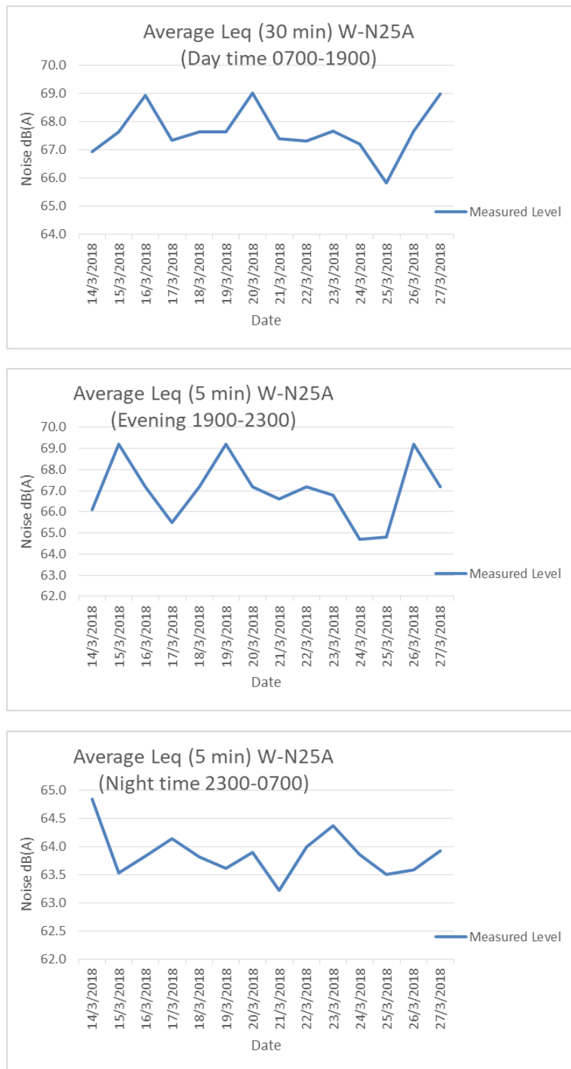
Figure F.3 Measured Noise Level for Prosperous Garden Block 1 (W-N25A)
