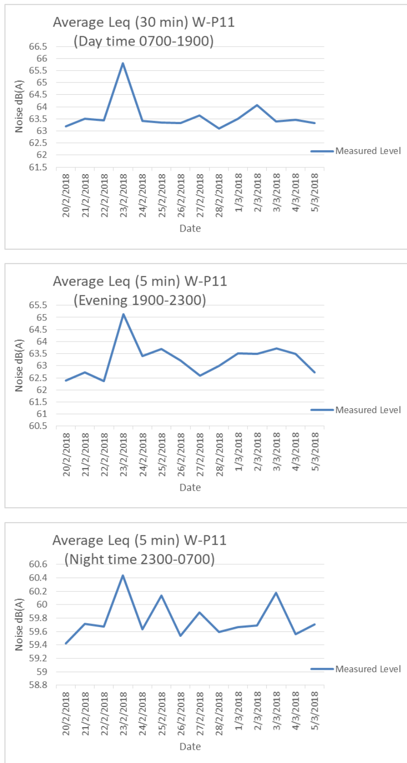
Figure F.4 Measured Noise Level for The Coronation (W-P11)
