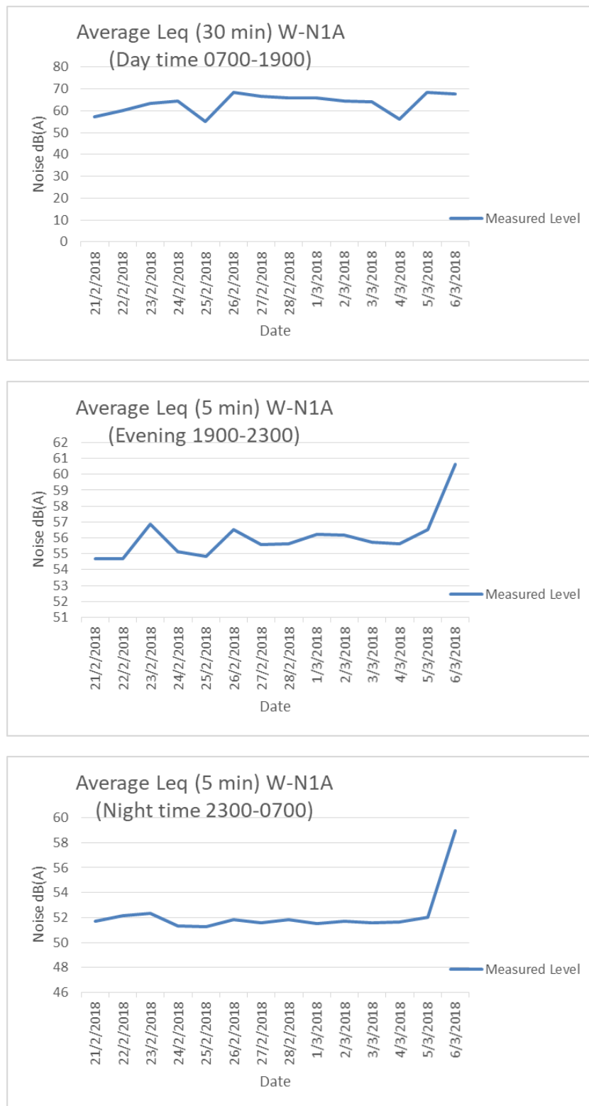
Figure F.1 Measured Noise Level for Yau Ma Tei Catholic Primary School (W-N1A)
