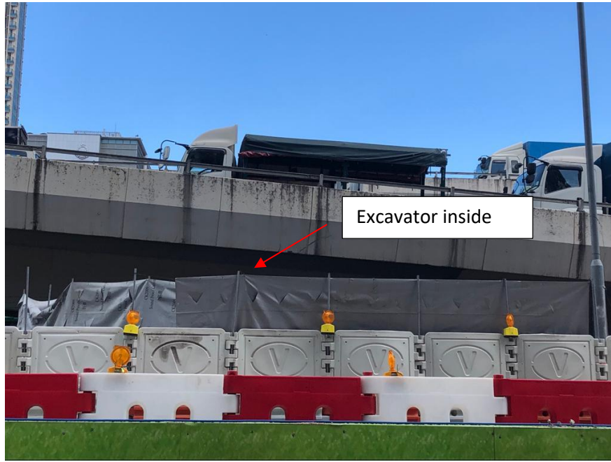
Figure A1: Erected noise barrier mat surrounding the excavator
