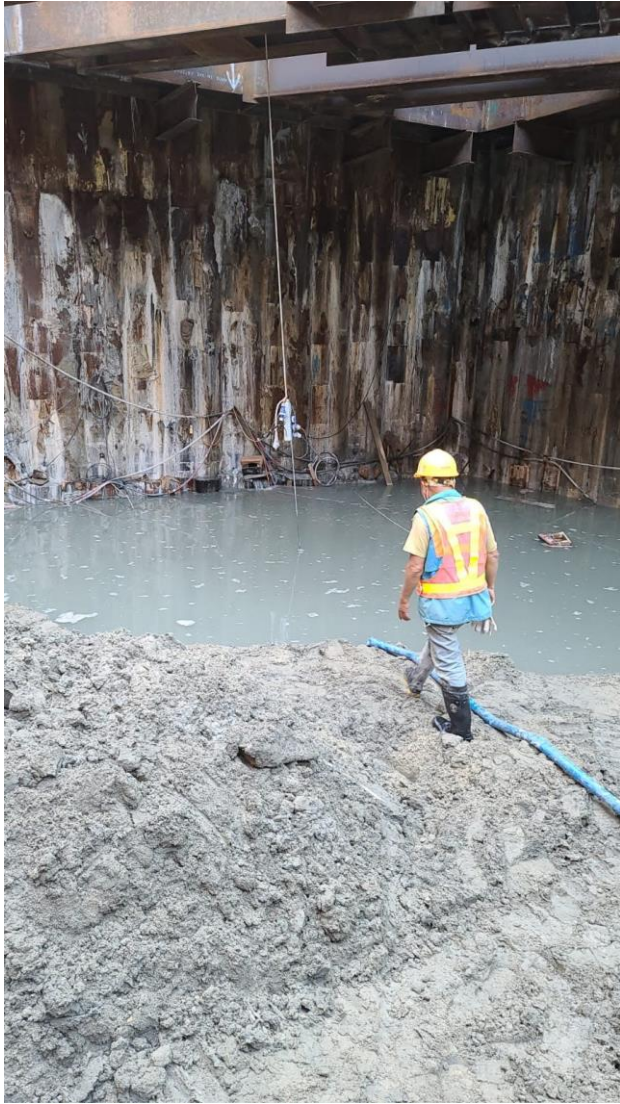
Figure A1: Water seepage at the cofferdam of ventilation adit in Portion 1D
