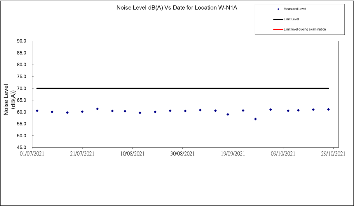
Figure 1: Graphical Illustration of Measured Noise Levels at W-N1A Remark: No examination was at W-N1A in the reporting month so limit levels for all monitoring days were 70 dB(A).
