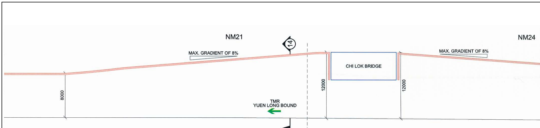
LONGITUDINAL SECTION ALONG TMR YUEN LONG BOUND BETWEEN NM21 AND NM24 (N.T.S.)
