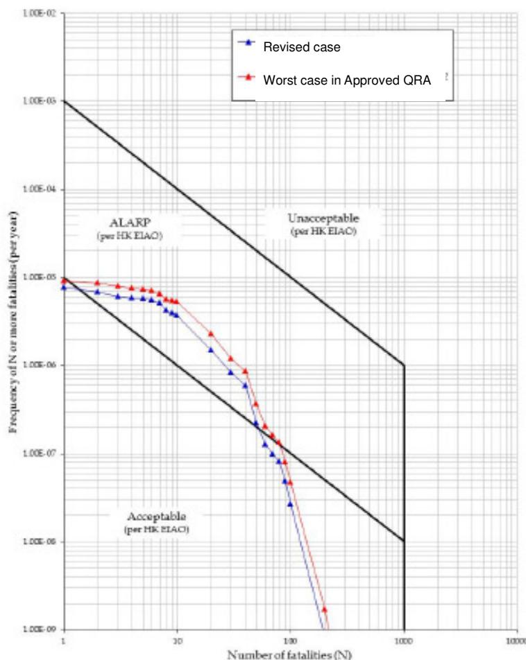
Figure 1 F-N Curve (Societal Risk) for Storage and Transport of Explosives
