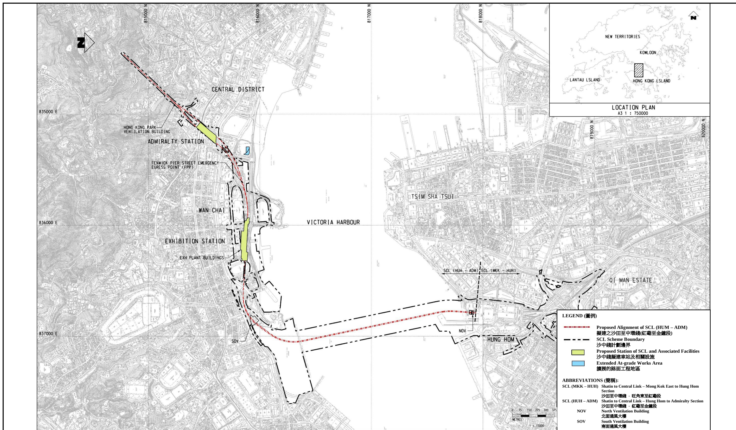
Figure 1: Alignment of Shatin to Central Link - Hung Hom to Admiralty Section
