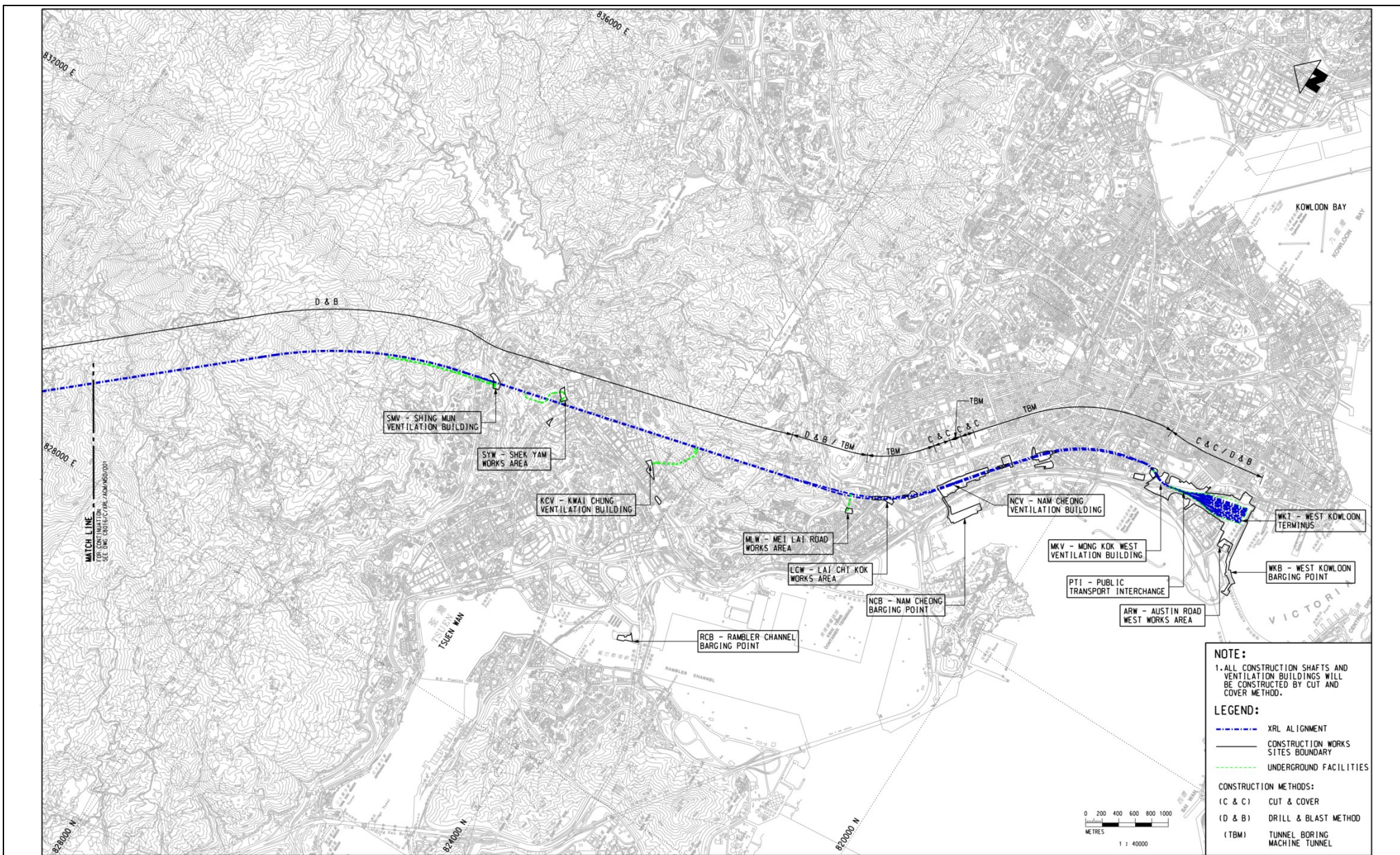
Figure 2: Overall View of Alignment & Works Sites [This figure was prepared based on Figure No. C8016/C/XRL/ACM/M50/002 (REV. F) submitted under Application No. VEP-439/2014]
