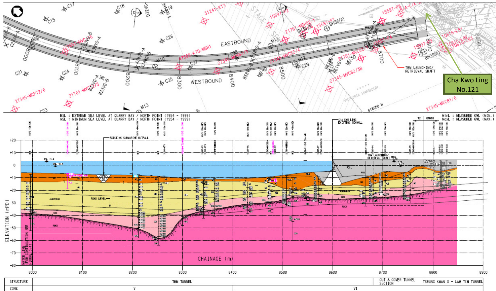
Figure B-3 Longitudinal Geological Profile at Cha Kwo Ling
