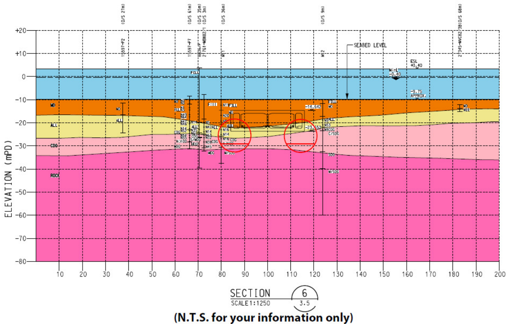
Figure B-4 Geological Cross Section at Ch8550 near Retrieval Shaft
