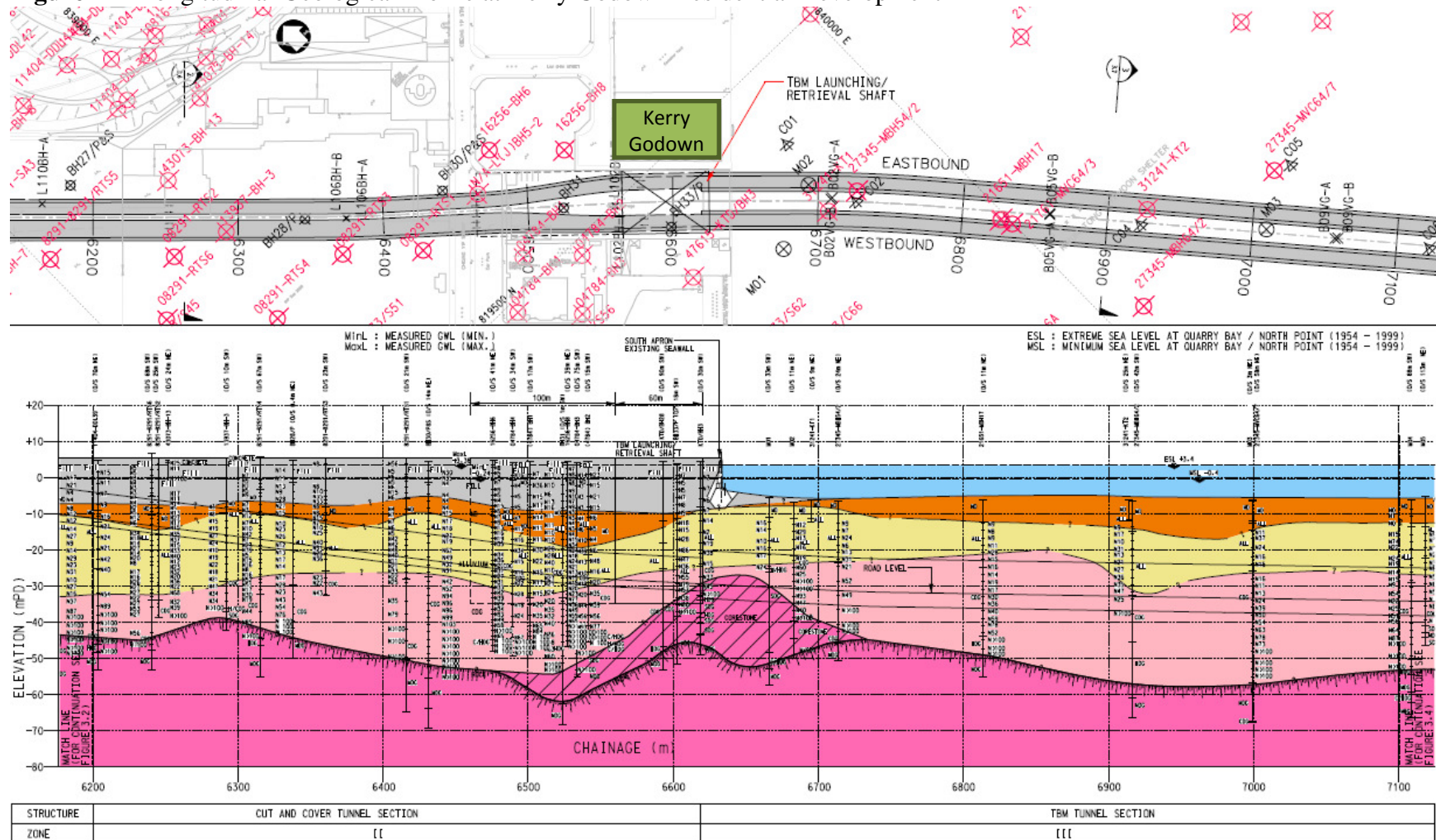
Figure B-1 Longitudinal Geological Profile at Kerry Godown Residential Development
