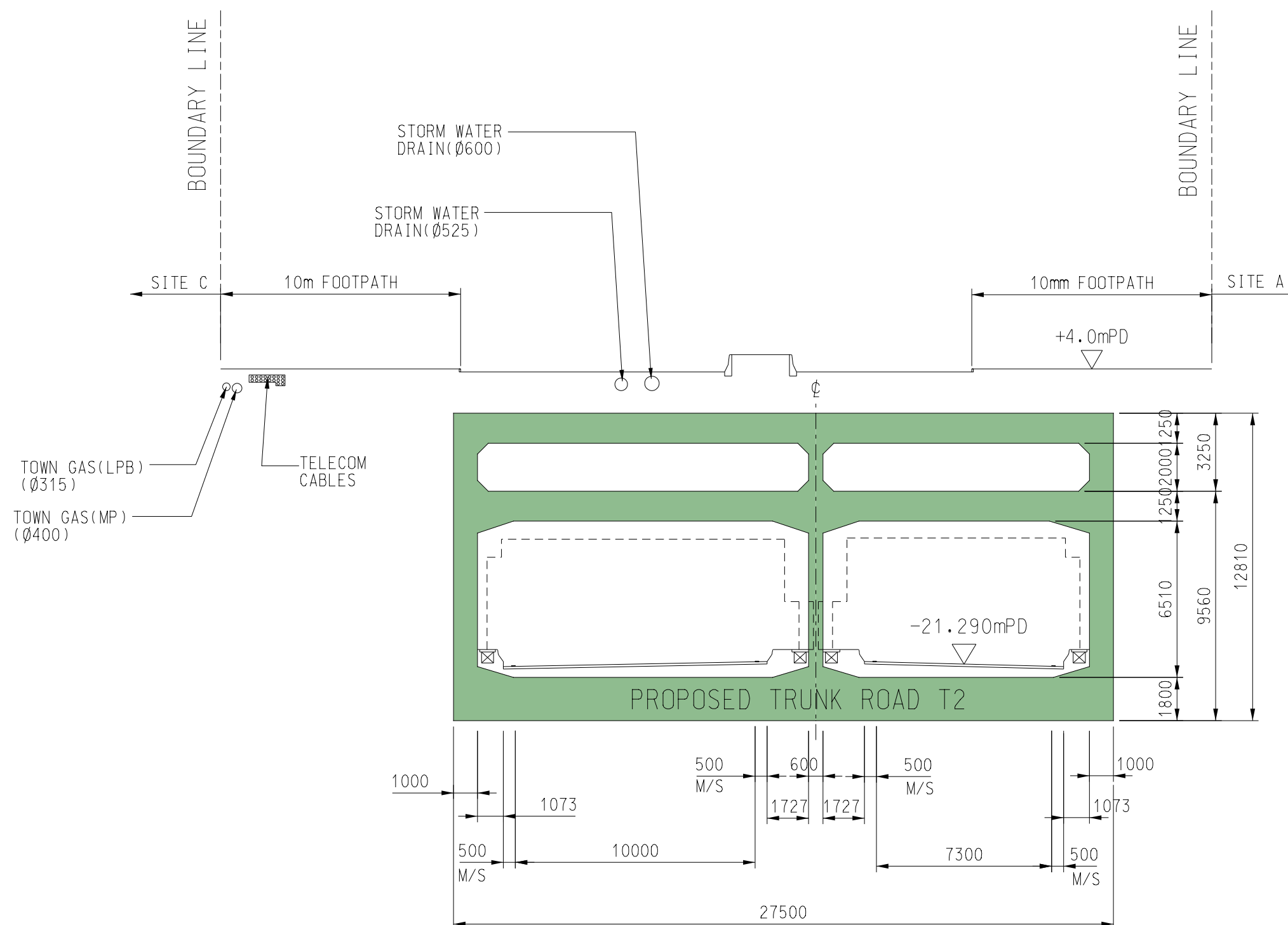
TYPICAL SECTION
