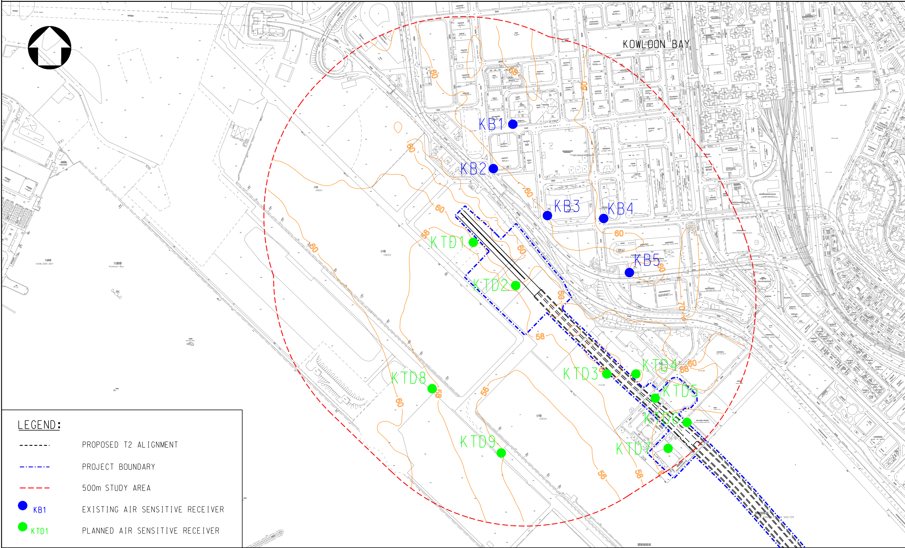
OVERALL CUMULATIVE 24HR RSP CONCENTRATION AT 1.5M ABOVE GROUND LEVEL AT KT AREA (AQO: 180 \mu\text{g}/\text{m}^3 )
