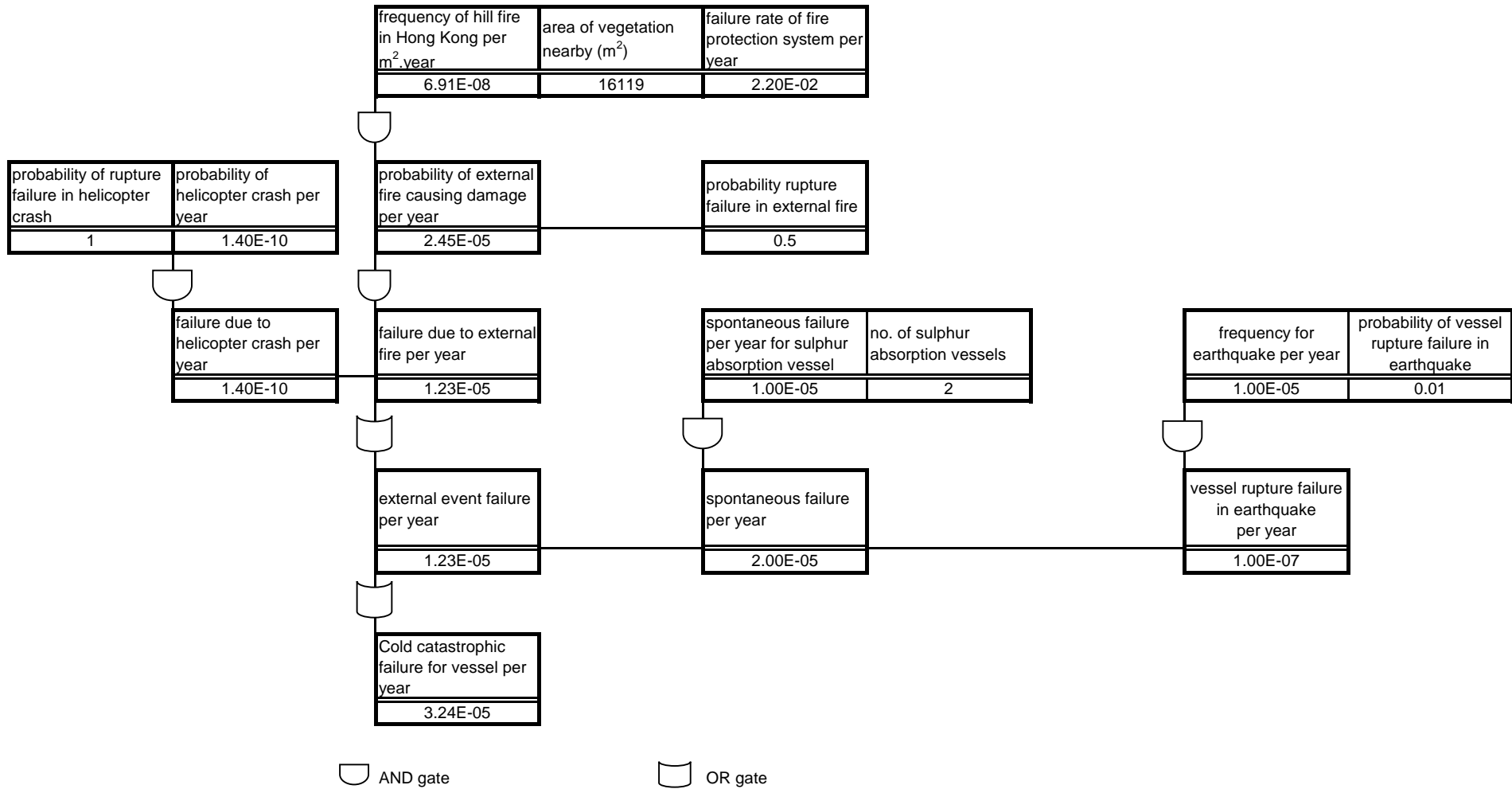
Figure 5 Catastrophic Failure of Sulphur Absorption Vessels
