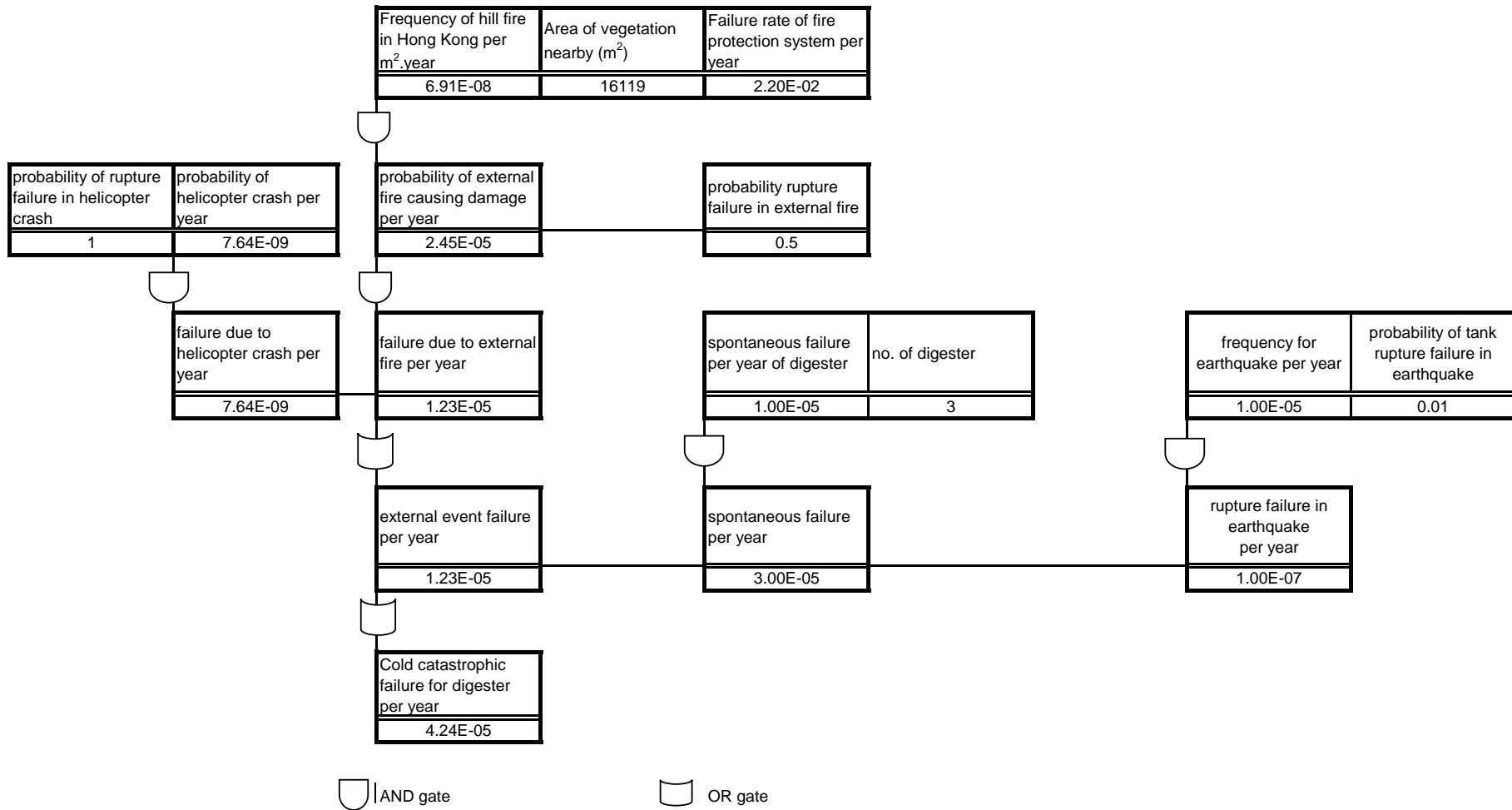
Figure 3 Catastrophic Failure of Digesters
